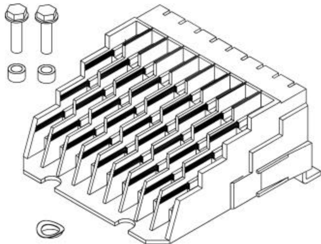
Figure 18. Secondary Disconnect.
