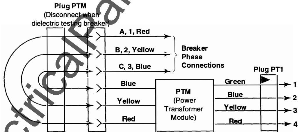
Figure 7-3 Digitrip RMS/R 700/800 PT Module
