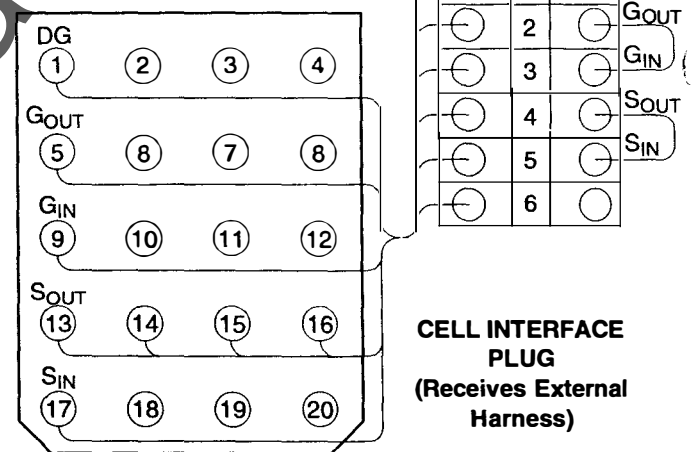
RMS/R 500 CELL HARNESS STYLE NO. 6502C71G01 6503C57G01
