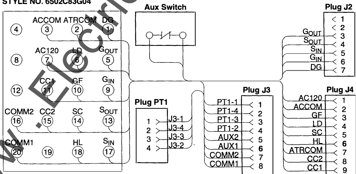
Figure 7-1 Digitrip RMS/R 7/800 External Harness
