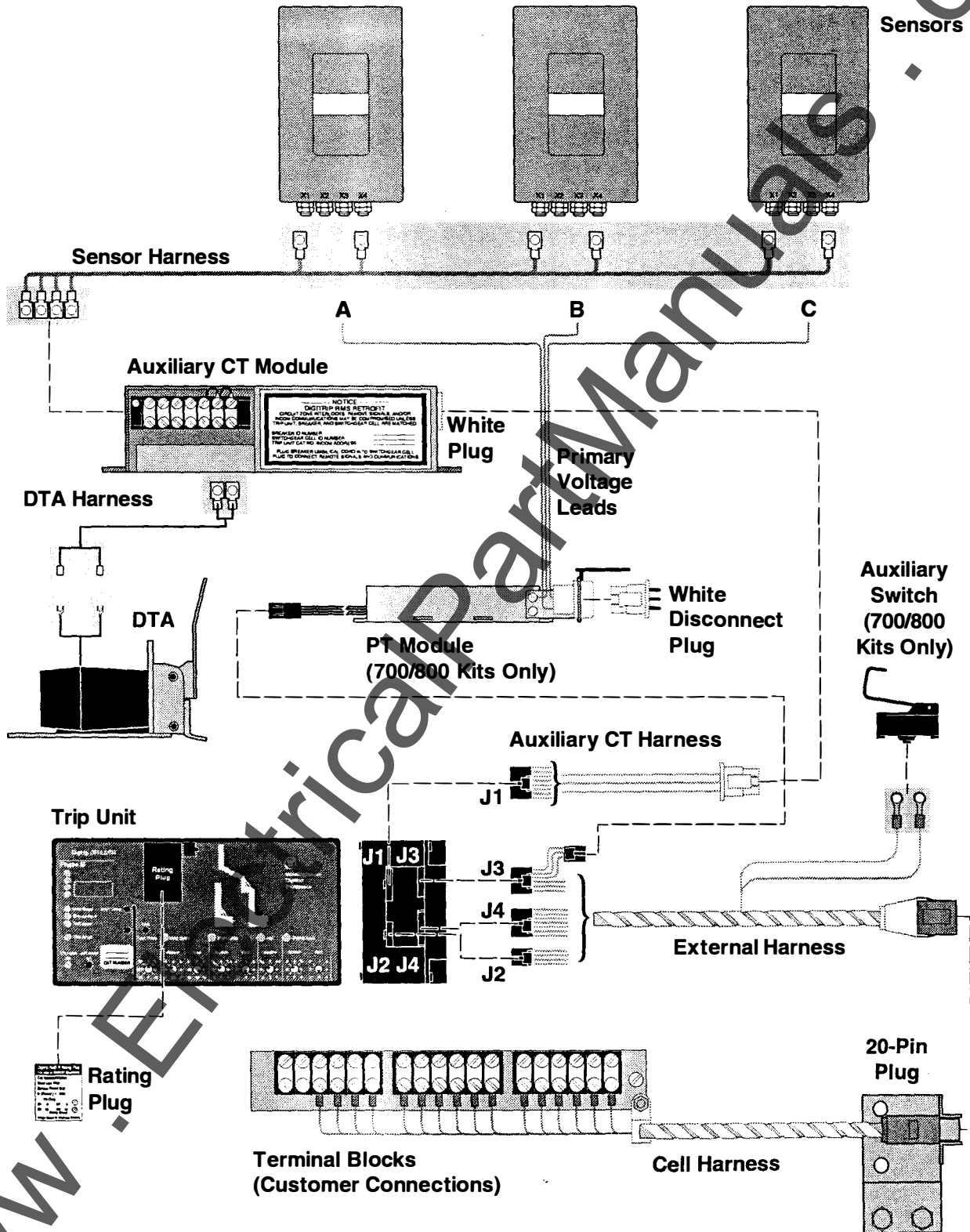
Figure 3-1 Digitrip Retrofit System
