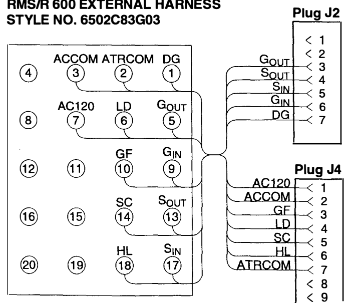
Figure 6-1 Digitrip RMS/R 600 External Harness
