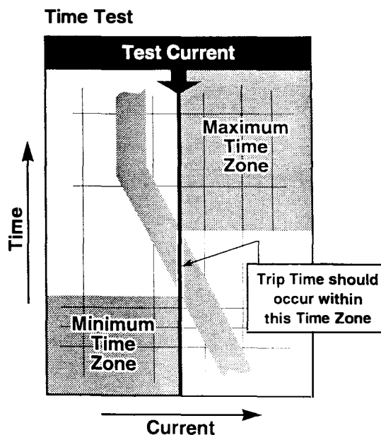
Figure 8-1 Pick-up Test and Time Test
