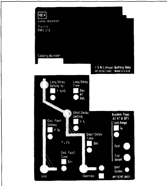
Fig. 2.5 Long Time/Short Time/Ground/Protection (LSG)
