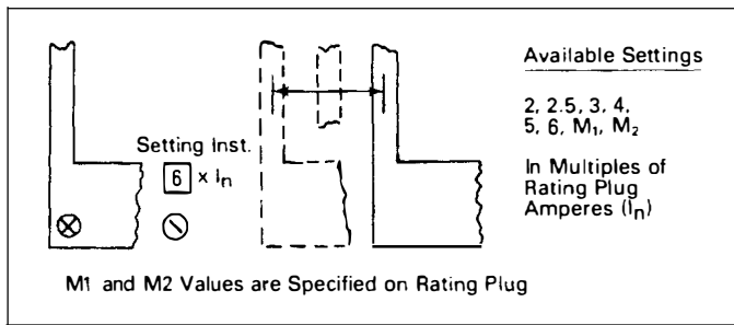
Fig. 4.5 Instantaneous Current Settings
