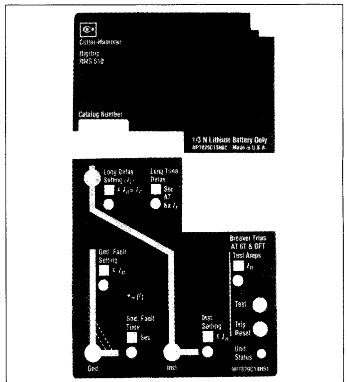
Fig. 2.4 Long Time/Instantaneous/Ground Fault Protection (LIG)
