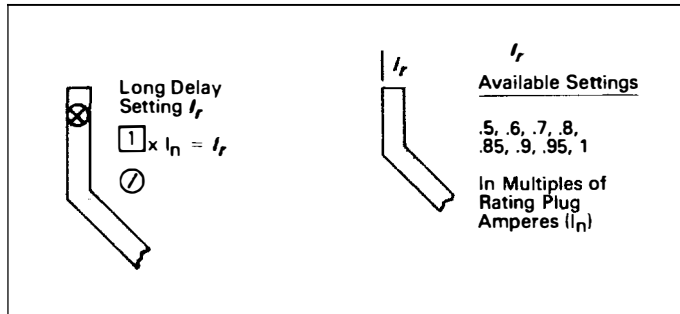
Fig. 4.1 Long Delay Current Settings
