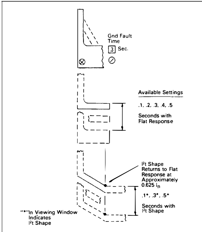
Fig. 4.7 Ground Fault Time Delay Settings
