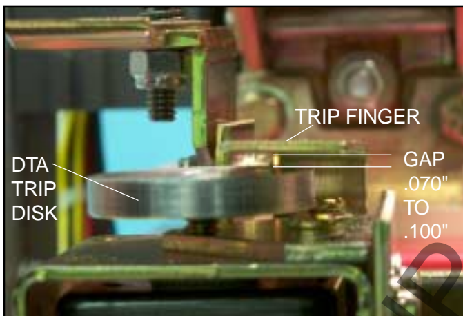
Fig. 48 Proper Air Gap Adjustment.
