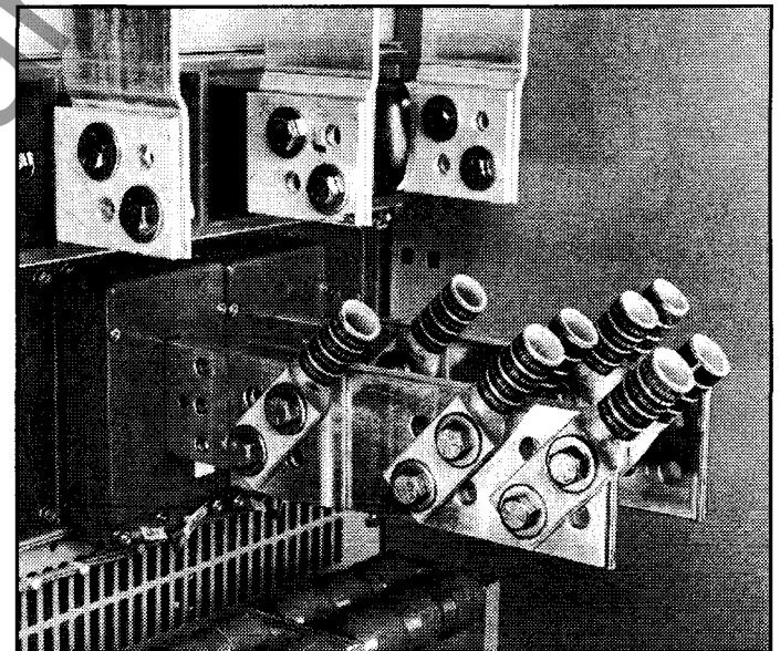
Figure 3-10 Load Runbacks with Lug Adapters
