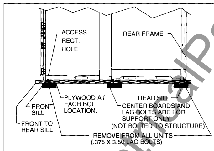
Figure 2-5 Shipping Skid
