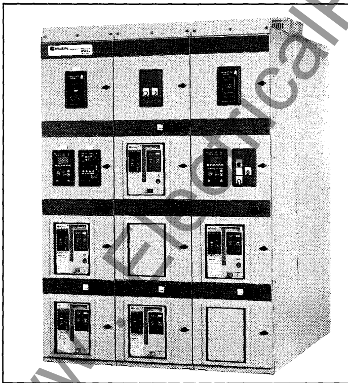
Figure 1-1 Type Magnum DS Low-Voltage Indoor Switchgear (Front View)
