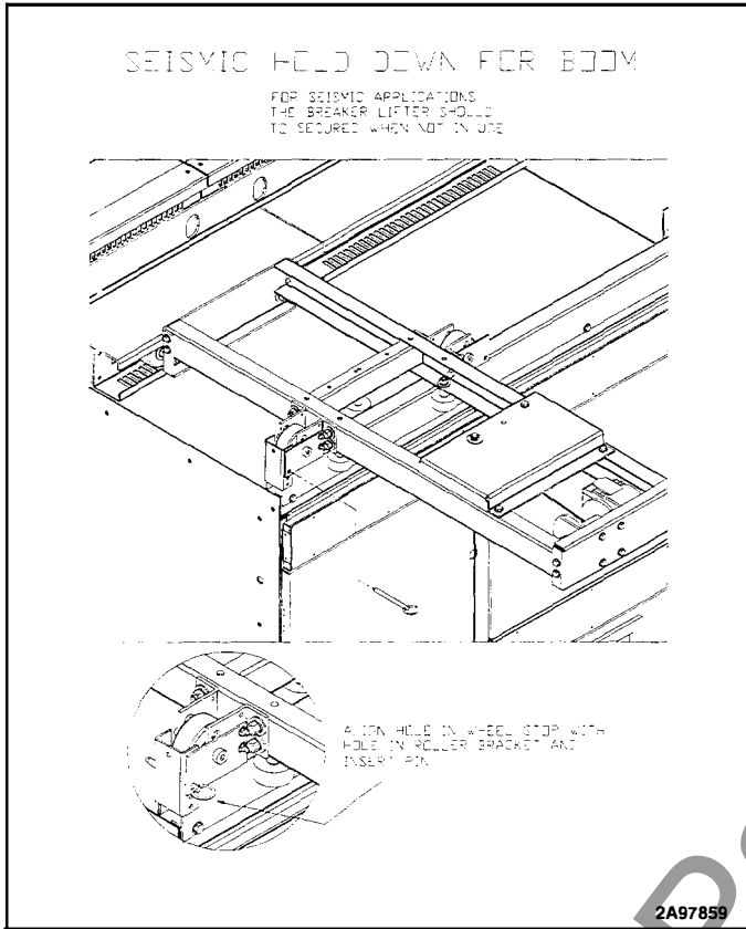
Figure 4-7 Breaker Lifter Installation
