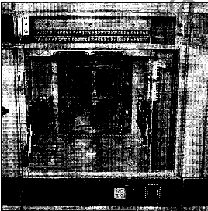
Figure 3-4 Magnum DS Breaker Cell
