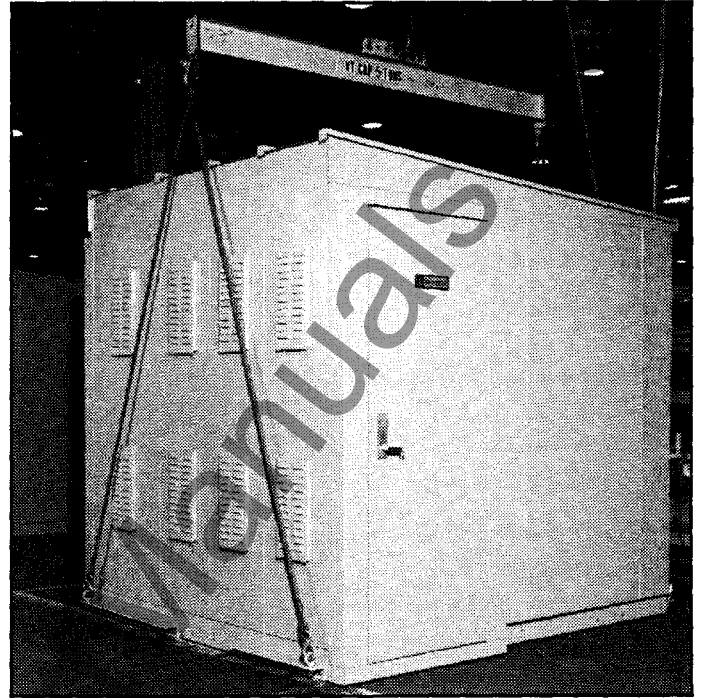
Figure 2-3 Outdoor Assembly Lifting Method
