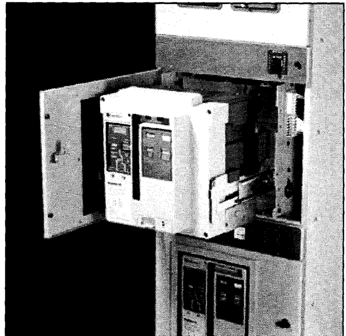
Figure 3-3 Magnum DS Breaker on Extension Rails
