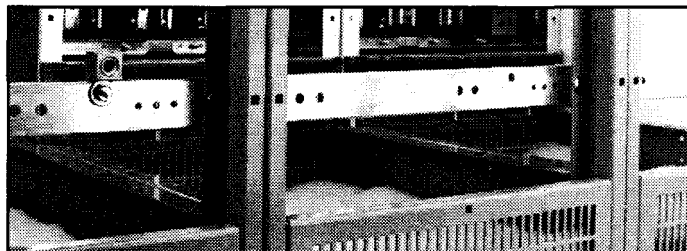
Figure 3-11 Ground Bus in Cable Compartment
