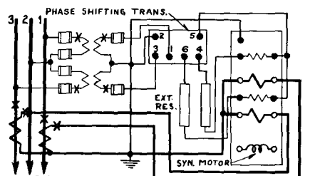
2 ELEMENT METER 2PH-3W CORRECT PH. SEQUENCE 1-2-3 CONNECTIONS ARE FOR LAG-0-LEAD SCALE REVERSE CUR. COIL CONN FOR LEAD-0-LAG. STD. WATTMETER CALIBRATION. FIG. 55—THREE-PHASE, 3-WIRE VAR METER, FLUSH TYPE ONLY
