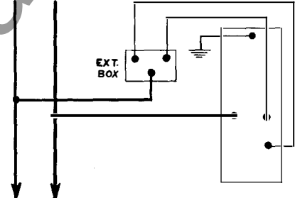
FIG. 53—FREQUENCY METER, FLUSH TYPE ONLY
