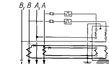
FIG. 37—TYPE GY-40 2 PHASE—4 WIRE POLYPHASE WATTMETER WITH C.T. AND WITHOUT P.T. PROJECTION TYPE ONLY
