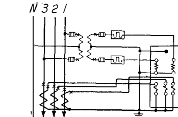
FIG. 44—TYPE GY-40 3 C.C. POLYPHASE WATTMETER WITH C.T. AND WITH P.T. PROJECTION TYPE ONLY
