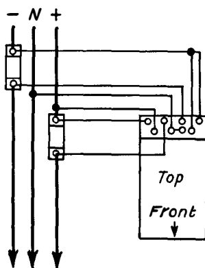
FIG. 74—THREE-WIRE D-C.
