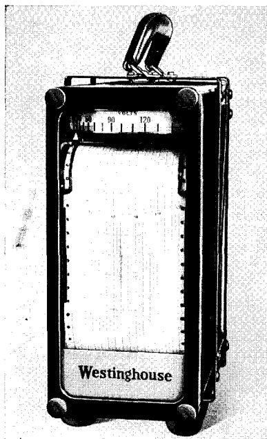
FIG. 8—PORTABLE TYPE GY-40 RECORDING A-C. VOLTMETER
