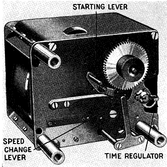
FIG. 1—SPRING DRIVEN HAND WOUND EIGHT-DAY CLOCK
