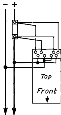
FIG. 73—TWO-WIRE D-C.
