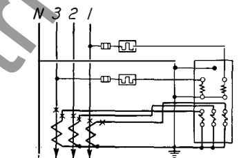
FIG. 43—TYPE GY-40 3 C.C. POLYPHASE WATTMETER WITH C.T. AND WITHOUT P.T. PROJECTION TYPE ONLY
