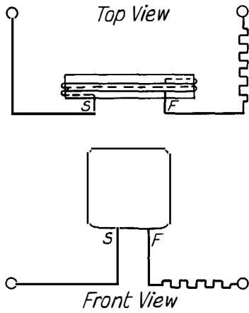
FIG. 10—TYPE GX-40 D-C. RECORDING VOLTMETERS OR MILLIVOLTMETER WITH SERIES RESISTANCE
