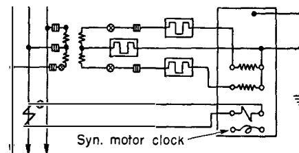
FIG. 57—POLYPHASE POWER FACTOR METER WITH ONE CURRENT TRANSFORMER, FLUSH TYPE ONLY
