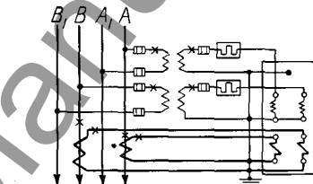
FIG. 38—TYPE GY-40 2 PHASE—4 WIRE POLYPHASE WATTMETER WITH C.T. AND WITH P.T. PROJECTION TYPE ONLY
