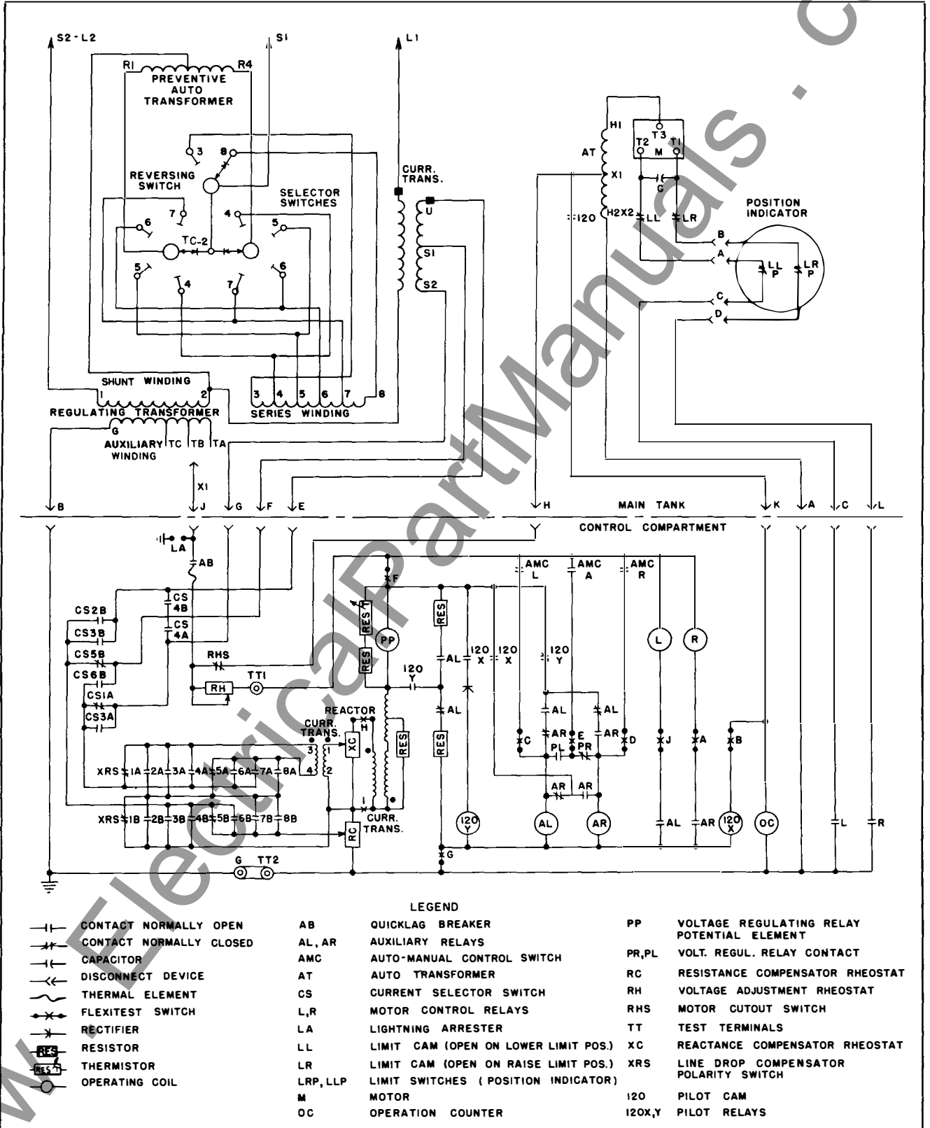
Fig. 15 - Schematic Diagram of Typical URF Regulator
