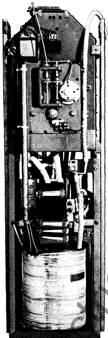
Fig. 16 - URF Internal Assembly Removed from Tank
