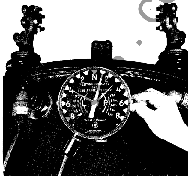
Fig. 14 - Position Indicator with Load Range Selector
