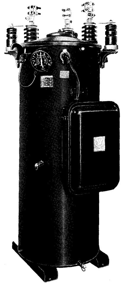
Fig. 1 - External View of URF Regulator
