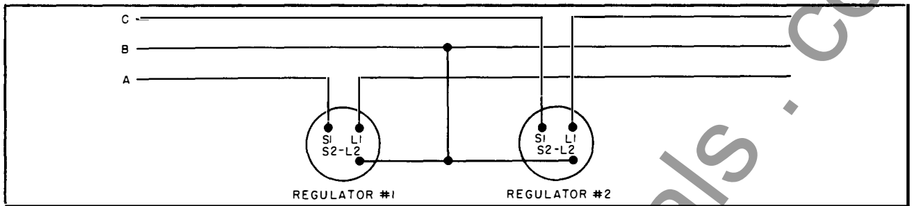
Fig. 9 - Two Units, Open Delta Connected on a Three Phase, Three Wire Circuit - Phase Sequence ABC
