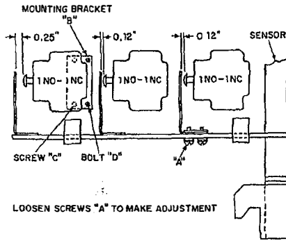
Fig. 41. Adjustments of interlock assembly
