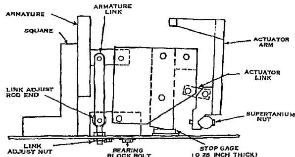
Fig. 57. Armature linkage assembly
