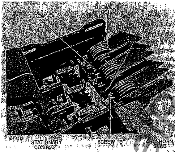
Fig. 36. Blowout base and main shaft assembly
