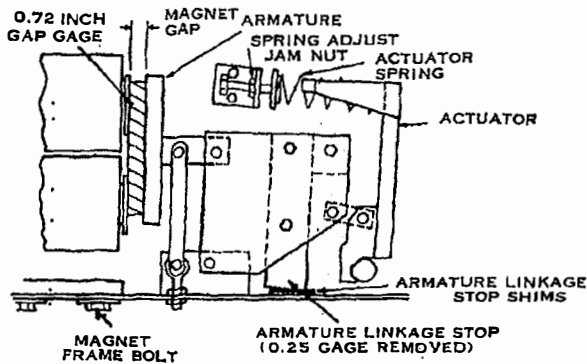
Fig. 58. Magnet and return-spring assembly
