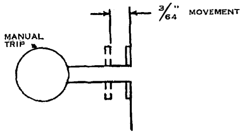
Fig. 51. Hand-release mechanism
