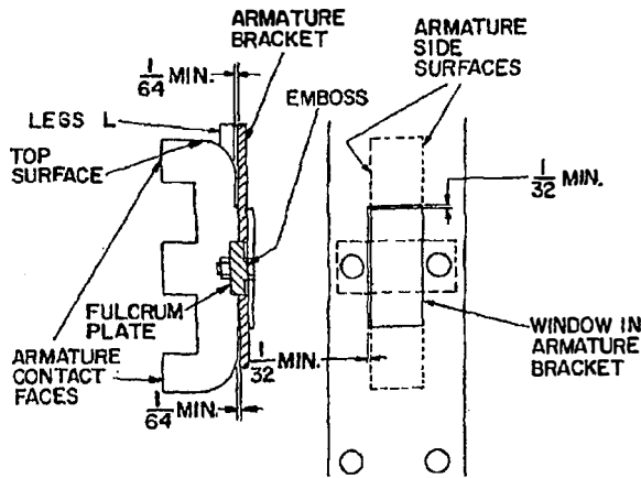
Fig. 29. Ac magnet assembly shown with contactor closed
