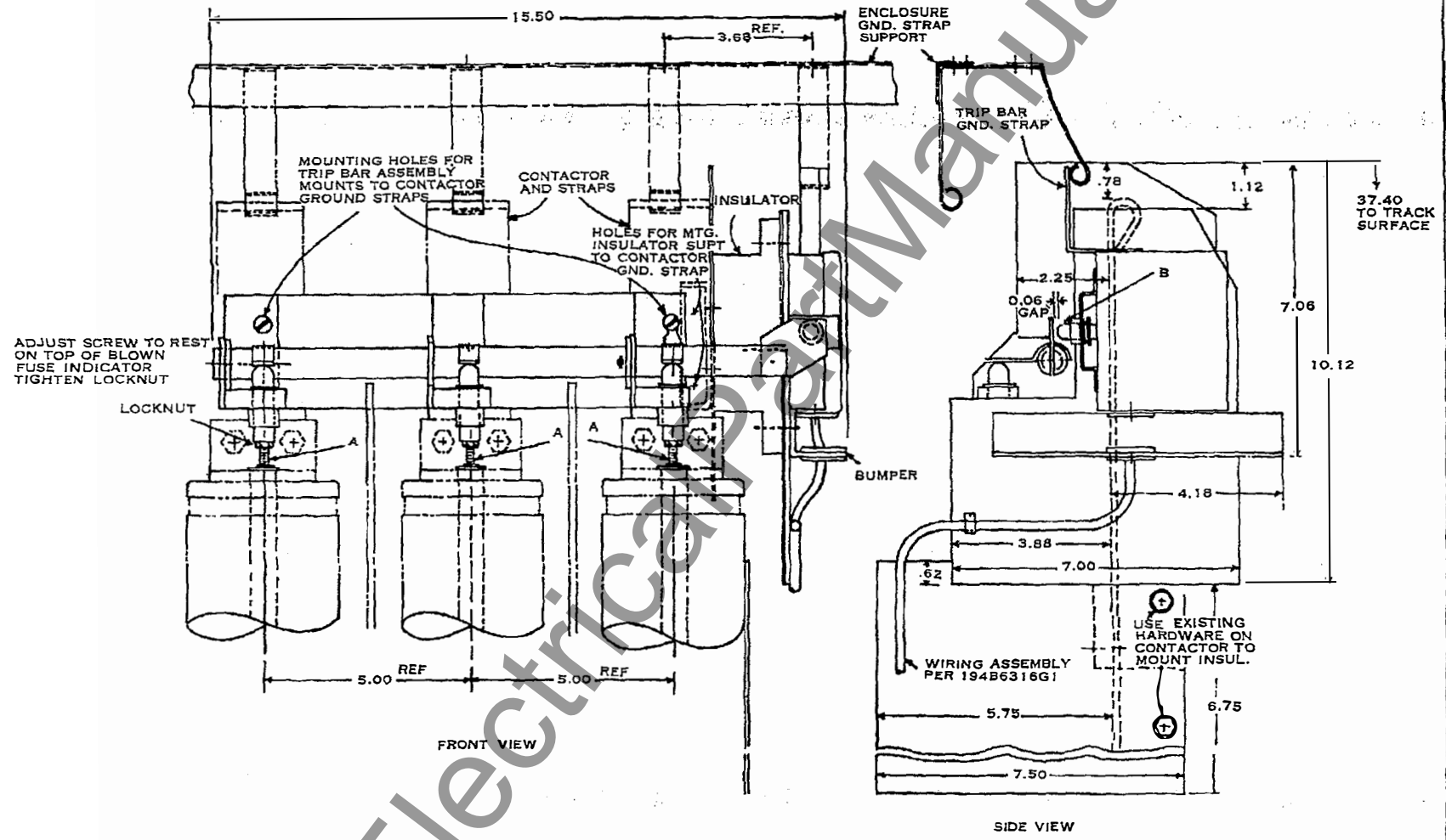
Fig. 54. Anti-single-phase mechanism
