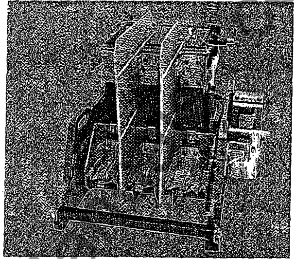
Fig. 2B. IC2814E220 three-high contactor for Limitamp that meets Underwriters Standard 347
