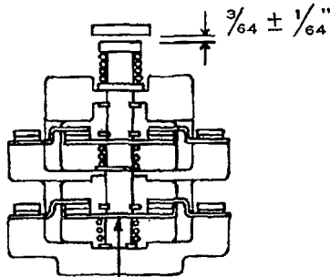
Fig. 52. Trip contact block
