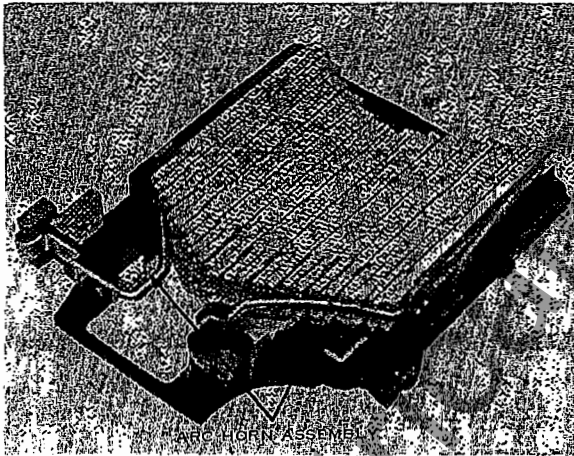
Fig. 9. Open view of arc chute showing vanes and arc horns
