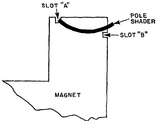
Fig. 31. Curved pole shaper
