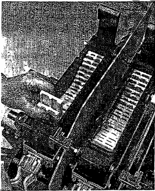
Fig. 24. Removal of arc barrier
