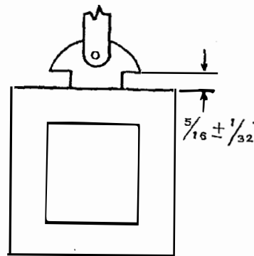
Fig. 50. Trip-solenoid armature
