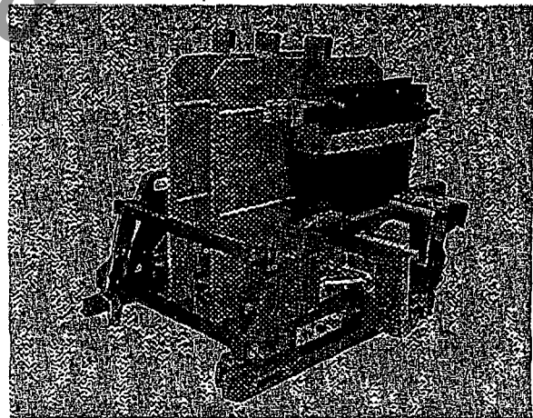
Fig. 1B. IC2814E220 three-high contactor less power fuses
