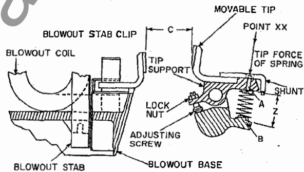
Fig 14. Movable and stationary contact structures
