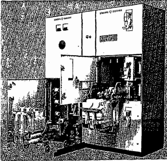
Fig. 8. One-high and three-high contactors in service position
