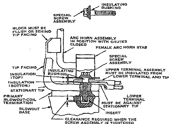
Fig. 47. Blowout-coil connection assembly
