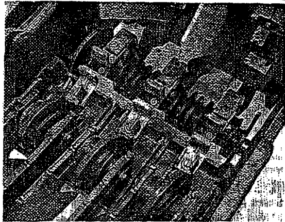
Fig. 46. Blowout assembly of 700-ampere contactor
