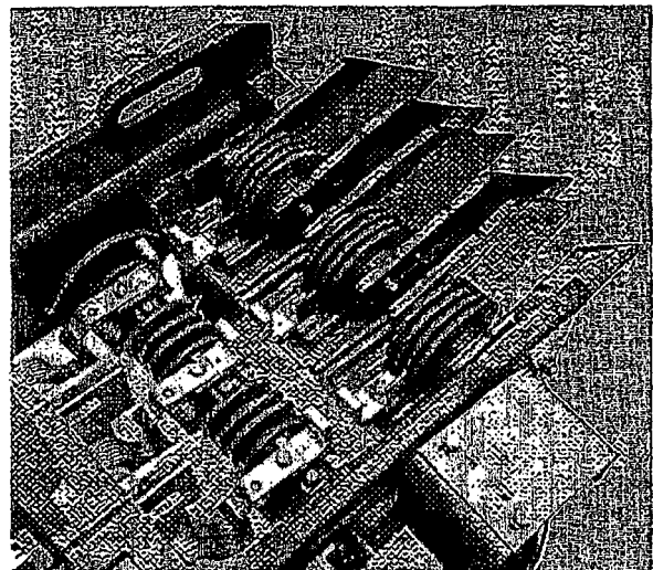
Fig. 18. Contactor open with pole pieces rotated out of position
