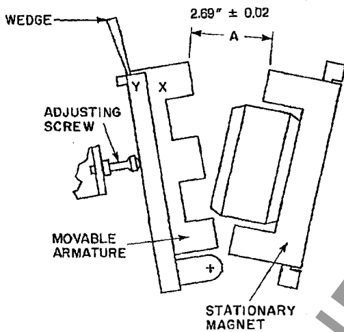
Fig. 15. Magnet structure (ac and dc)
