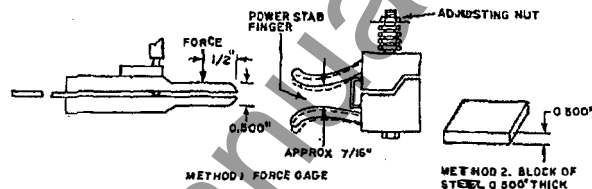
Fig. 36A. Adjustment of force on power stabs
