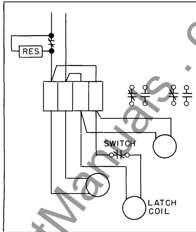
FIG. 15. Connections for 5 pole D-C Magnet Coils
