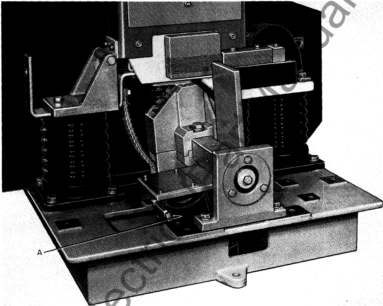
FIG. 8. D-C Holding Magnet
