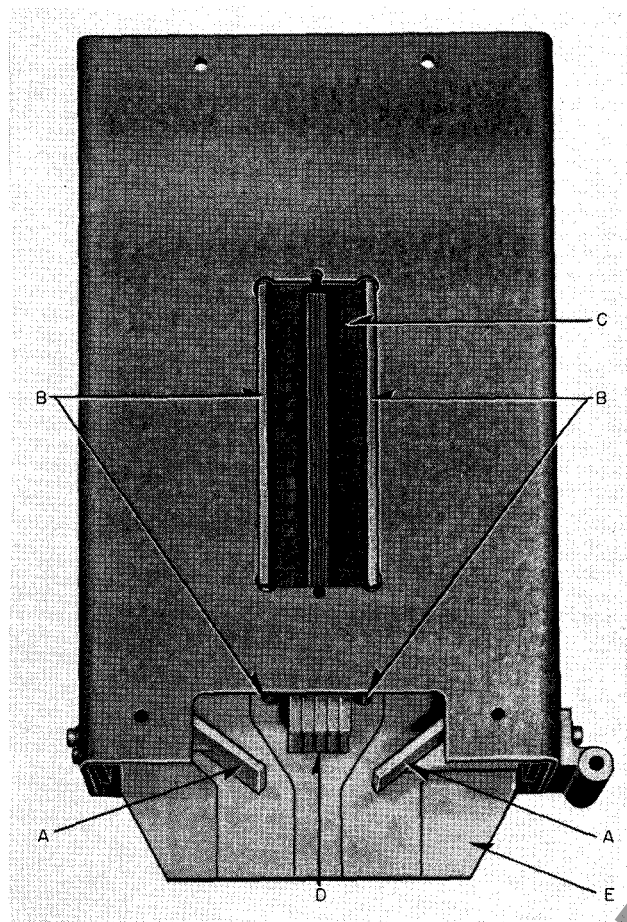
FIG. 6. Arc Chute—Partial Assembly
