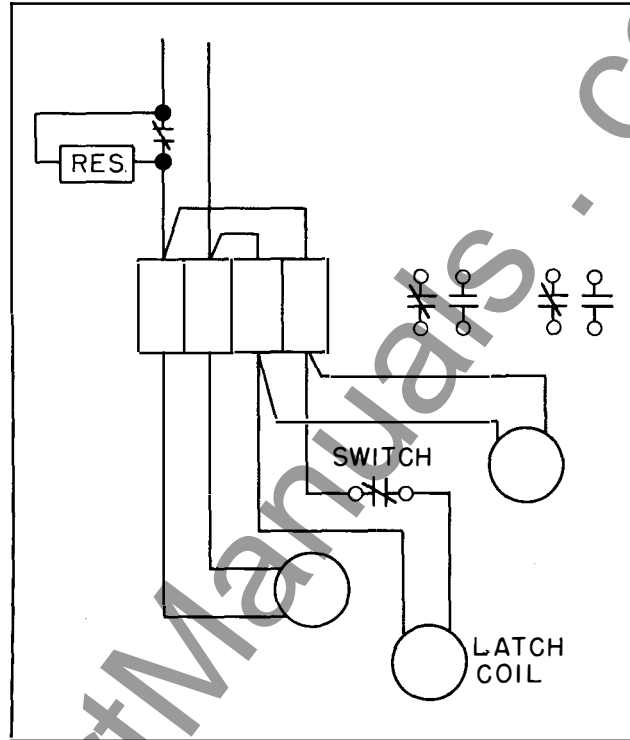
FIG. 15. Connections for 5 pole D-C Magnet Coils
