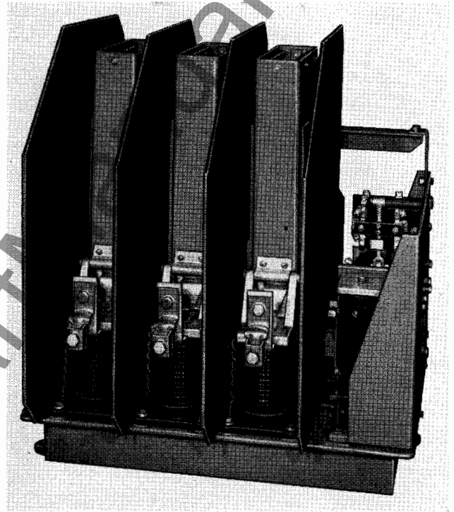
FIG. 2. Type H-430D—3 poles—D-C Magnet
