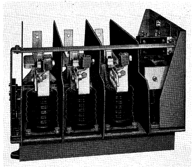
FIG. 4. Type H-403D—3 poles—Spring Closed
