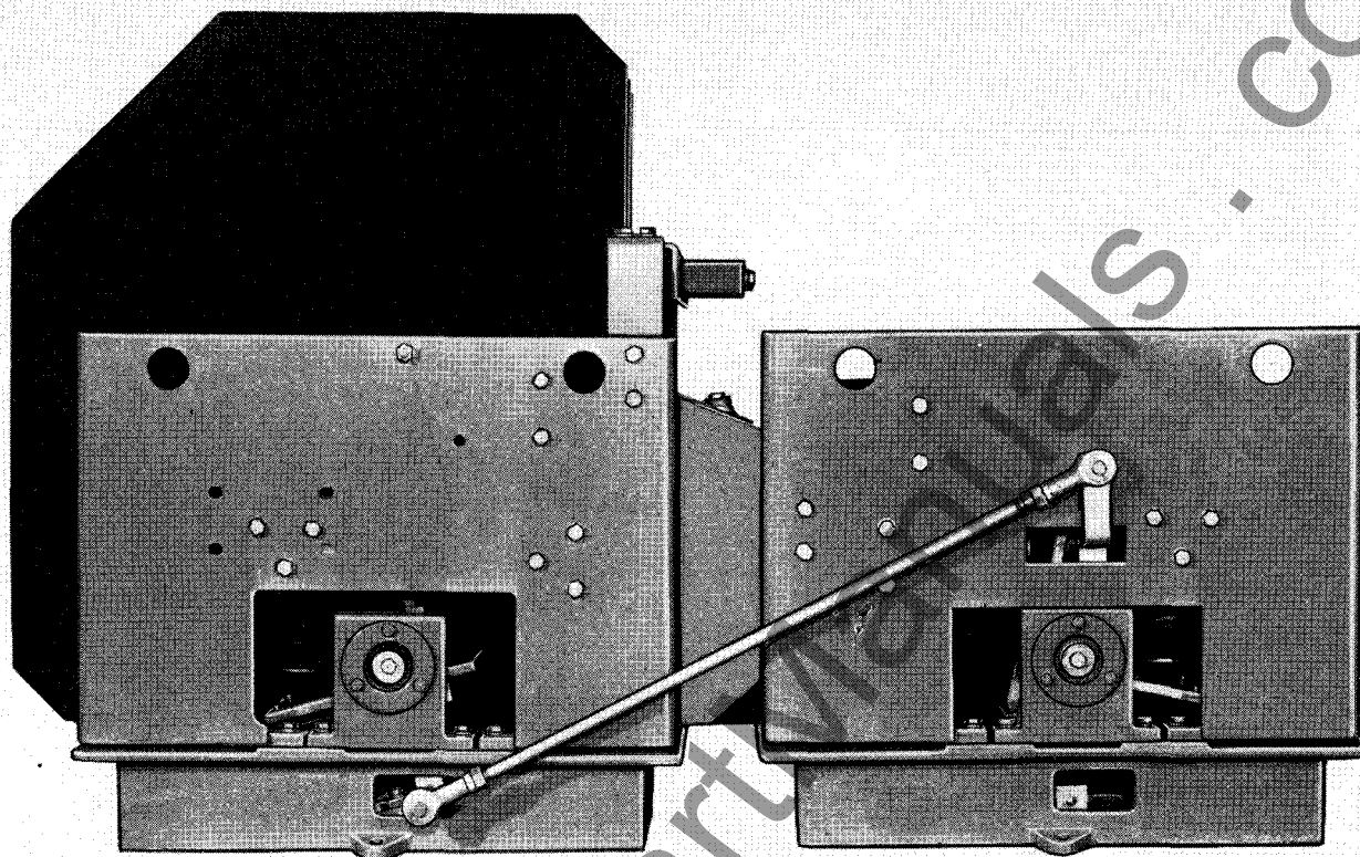
FIG. 9. Mechanical Interlock
