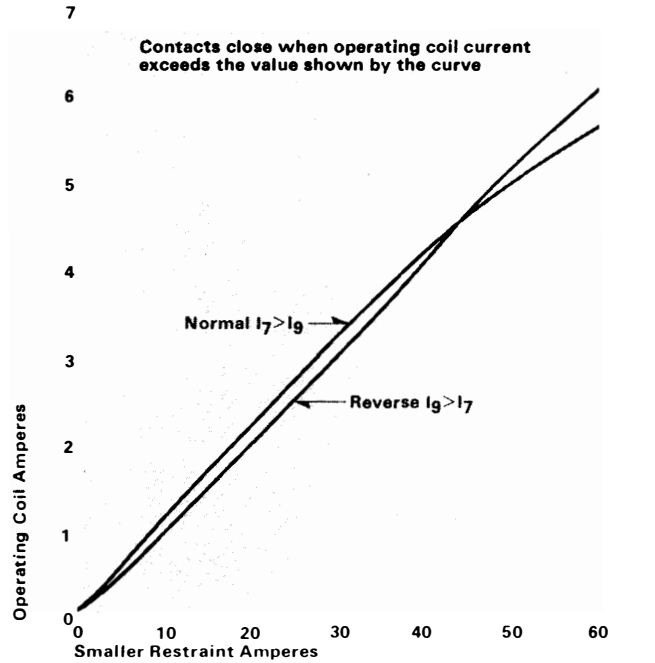
Figure 2 Curve 260208
