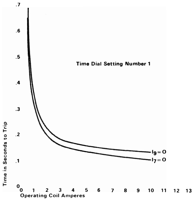
Figure 5 Curve 187A776
