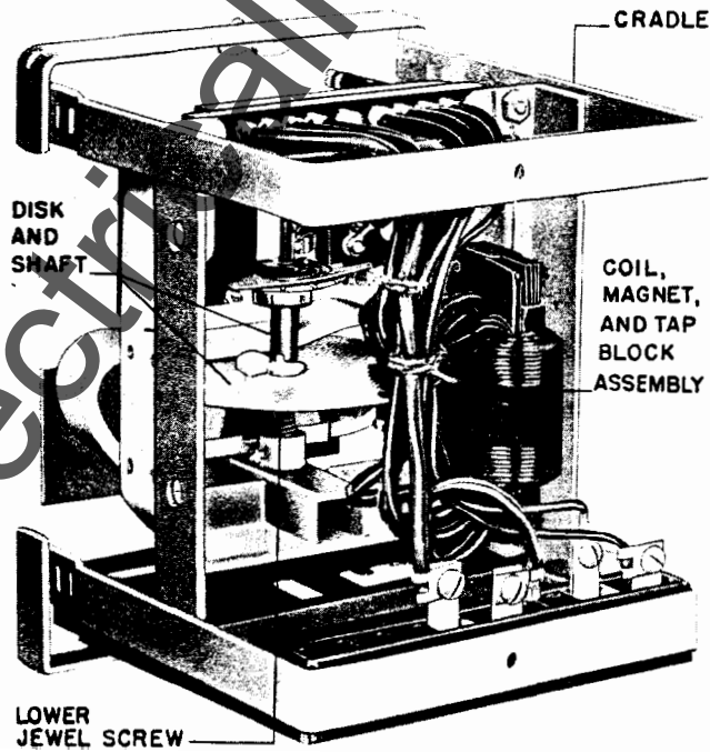
Fig. 1 The Induction Unit for Type IAC Relays B - (Rear View)
