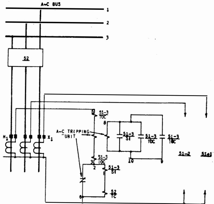
Fig. 6 External Connections of Three Type IAC51R Relays Used for 3-Phase Circuit Protection
