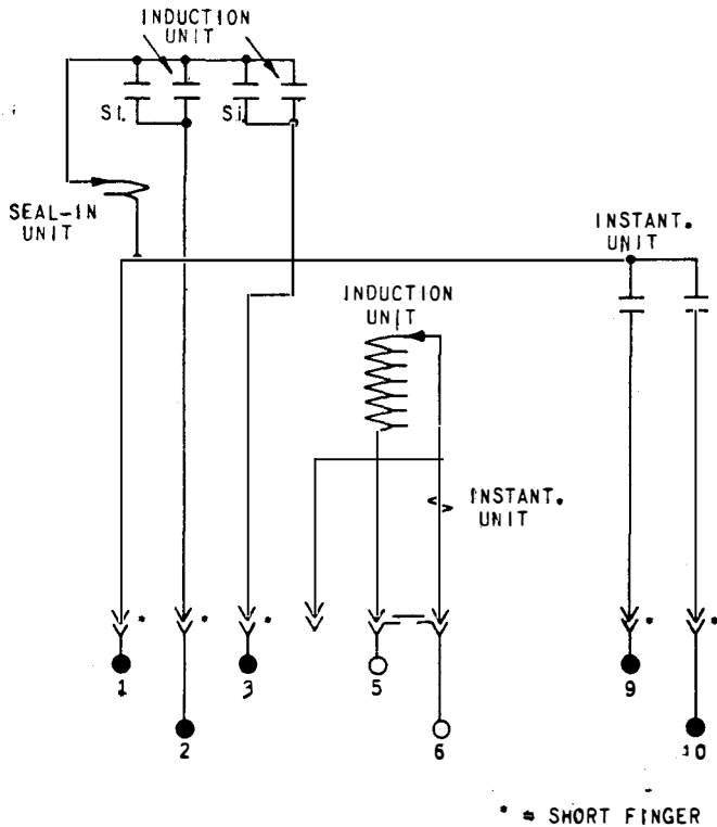
Fig. 17 Internal Connections for the Type IAC52B Relay (Front View)
