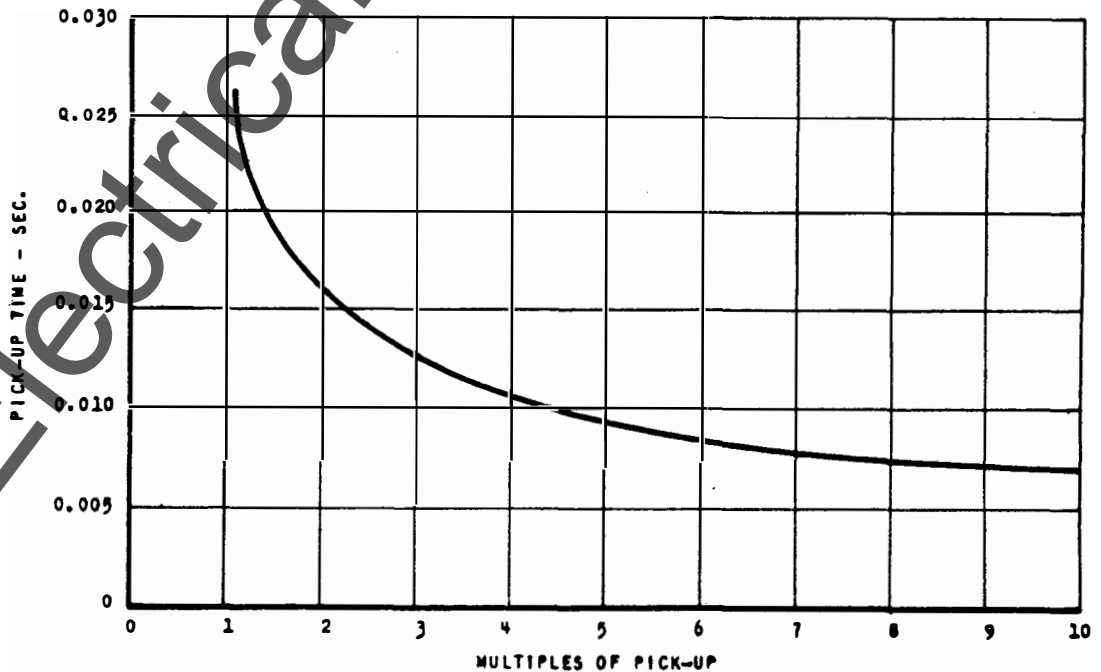
Fig. 10 Time-current Characteristics of Instantaneous Unit
