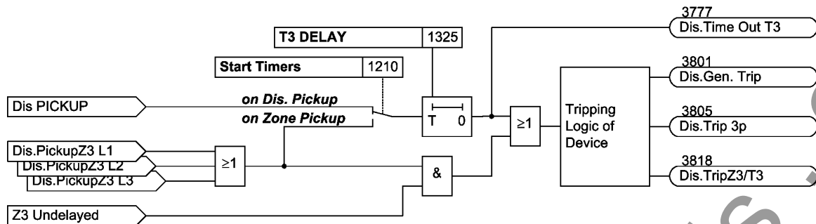
Figure 2-30 Tripping logic for the 3rd zone
