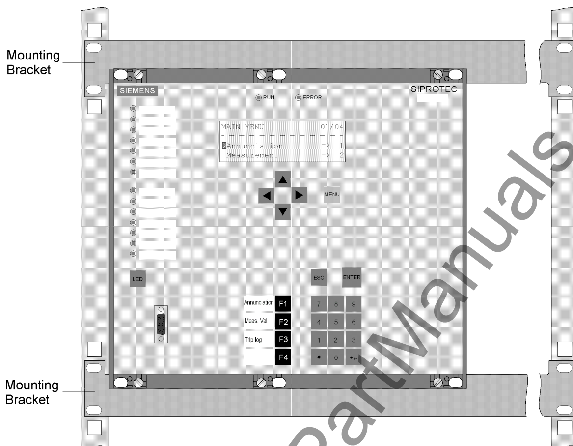
Figure 3-26 Mounting device in a rack or cubicle (housing size 2\frac{2}{3} ), as an example
