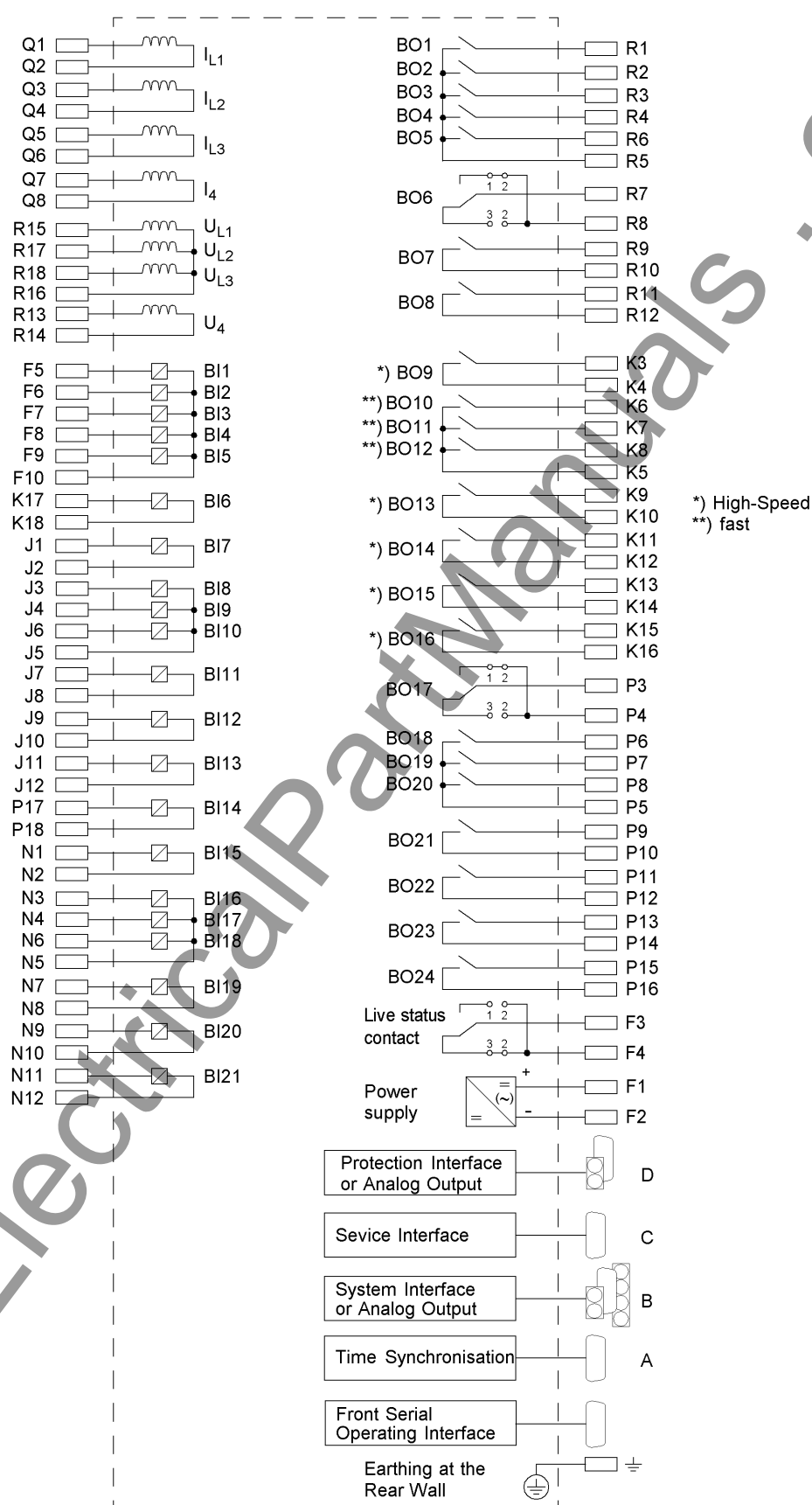
Figure A-12 General diagram for 7SA613*-M (panel flush mounting or cubicle mounting)
