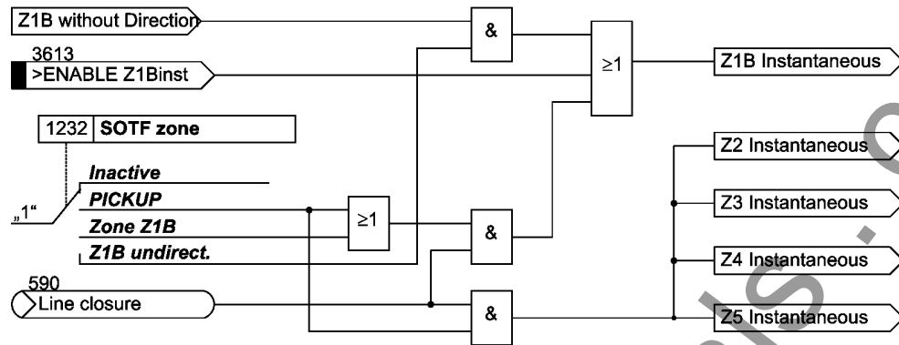
Figure 2-19 Circuit breaker closure onto a fault
