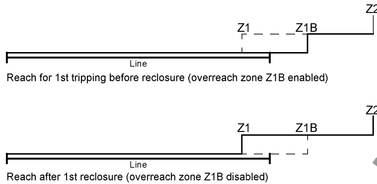
Figure 2-108 Reach control before first reclosure, using distance protection
