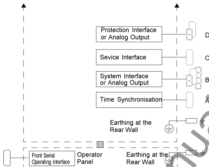
Figure A-30 General diagram 7SA642*-*N/S (panel surface mounting with detached operator panel)
