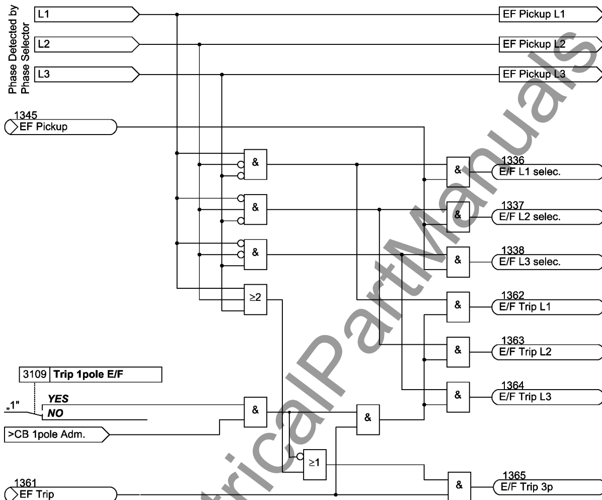
Figure 2-75 Logic diagram of single-pole tripping with phase selector
