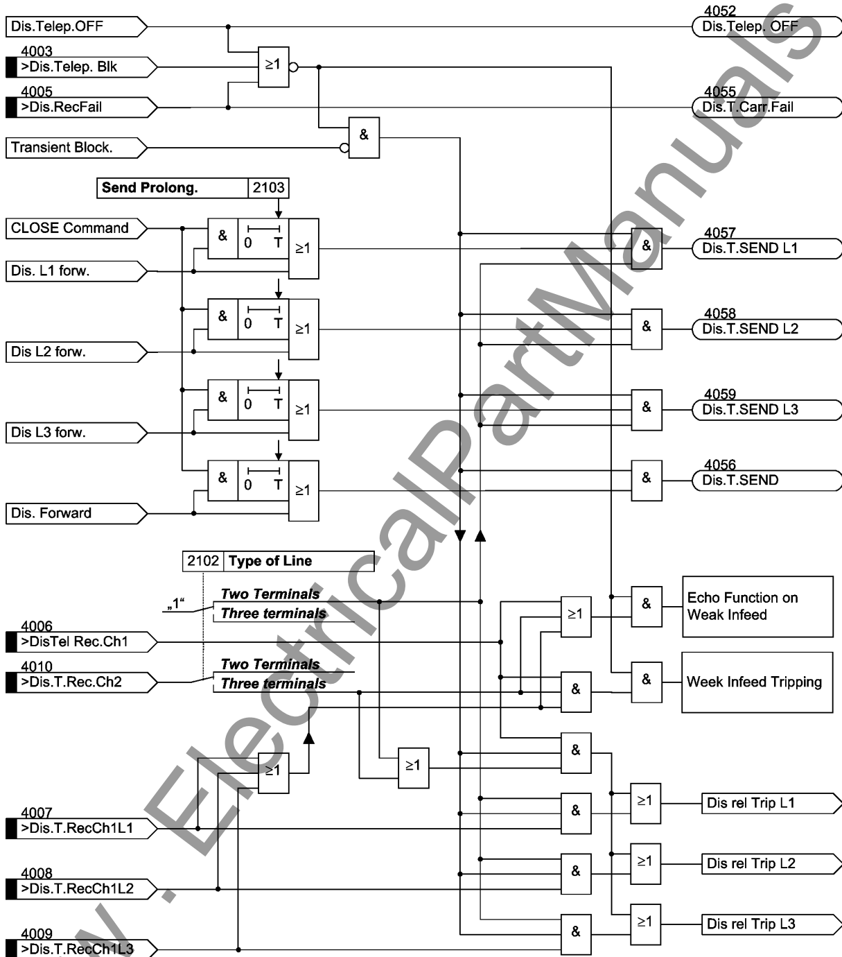
Figure 2-54 Logic diagram of the directional comparison scheme (one line end)
