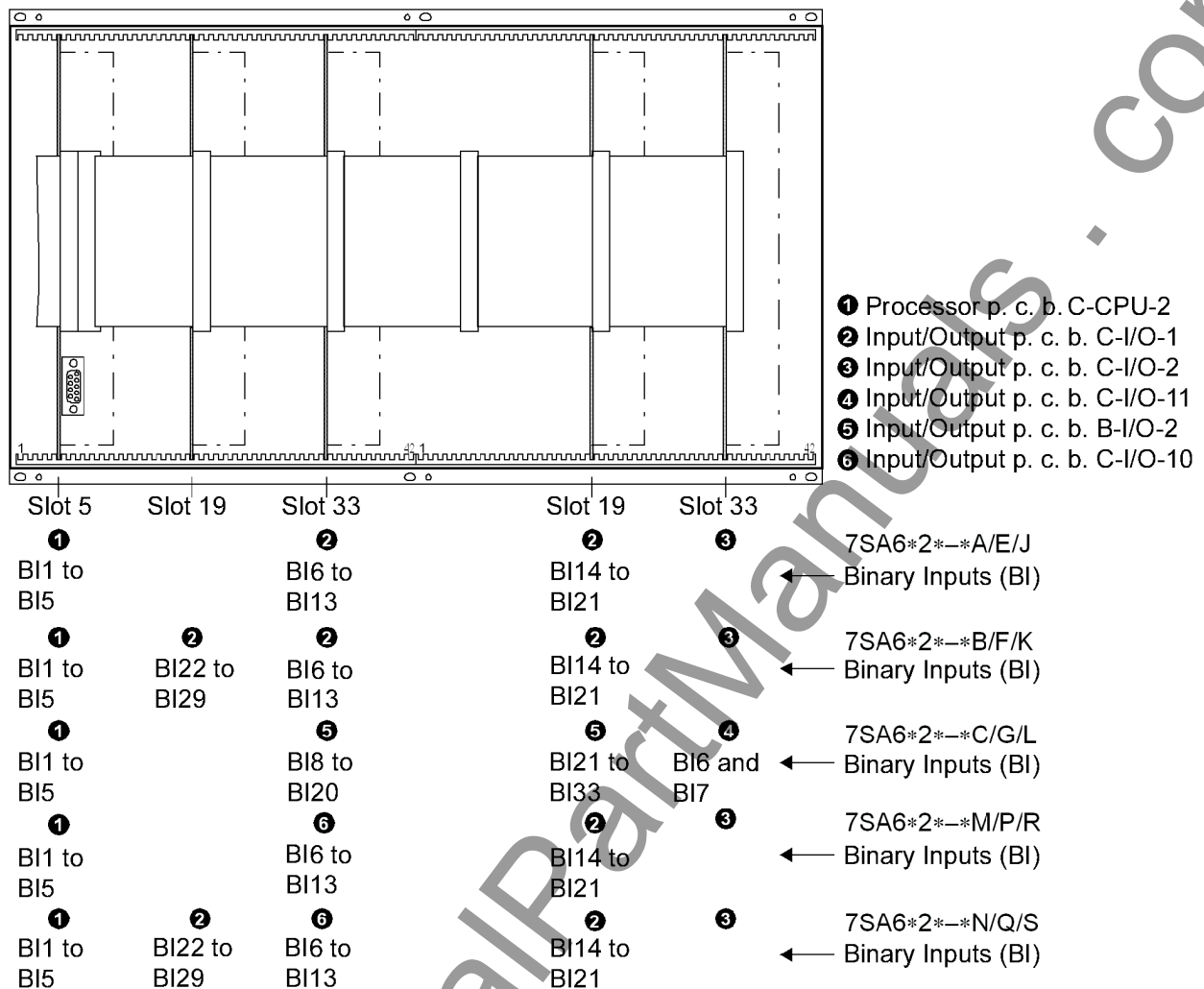
Figure 3-6 Front view with housing size \frac{1}{4} after removal of the front cover (simplified and scaled down)
