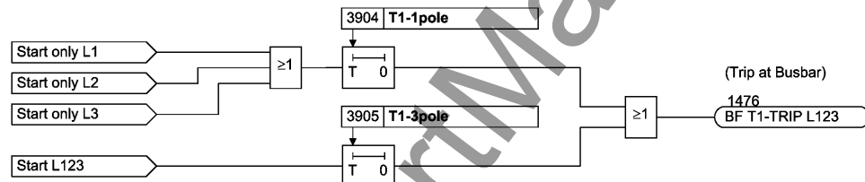
Figure 2-139 Single-stage breaker failure protection with different delay timers
