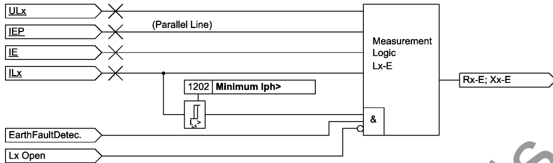
Figure 2-16 Logic of the phase-earth measuring system
