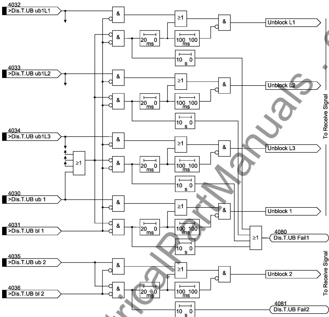
Figure 2-57 Unblock logic
