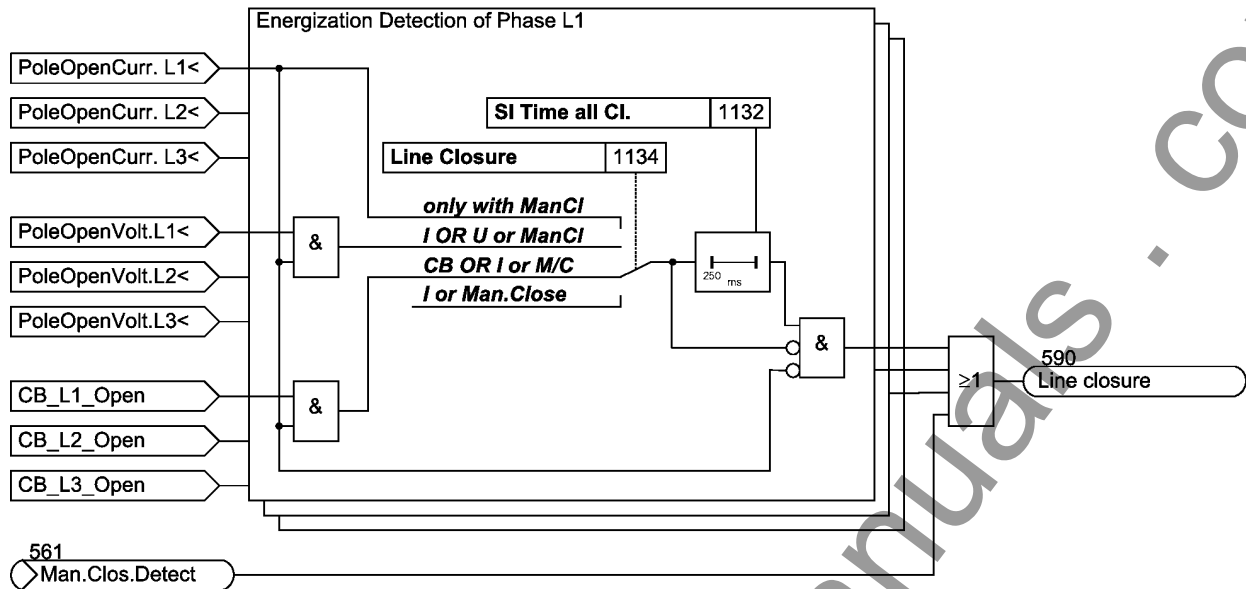
Figure 2-160 Generation of the energisation signal
