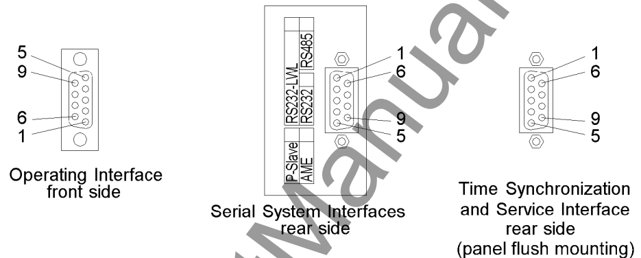
Figure 3-28 9-pin D-subminiature female connectors
