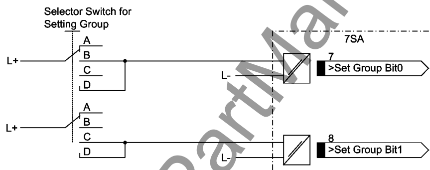
Figure 3-1 Connection diagram (example) for setting group switching with binary inputs
