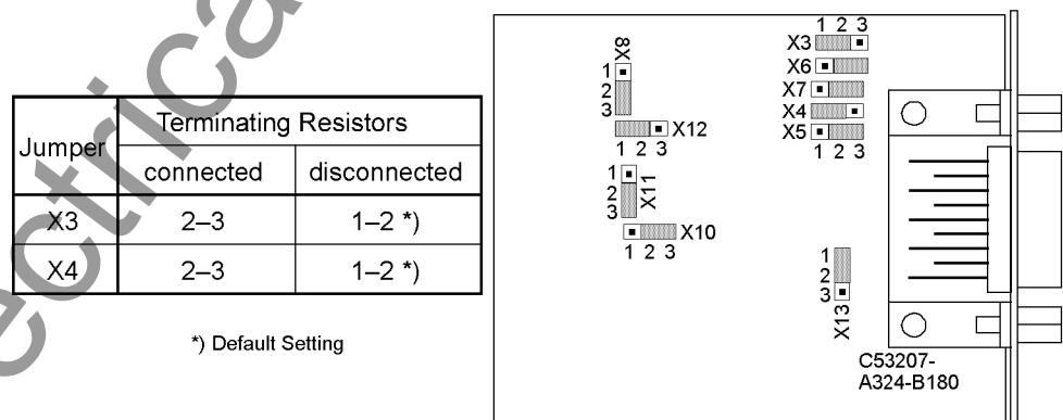
Figure 3-16 Position of terminating resistors and the plug-in jumpers for configuration of the RS485 interface
