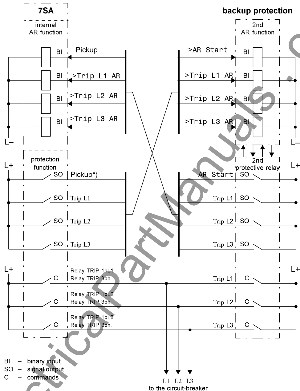
Figure 2-117 Connection example for 2 protection devices with 2 automatic reclosure functions
