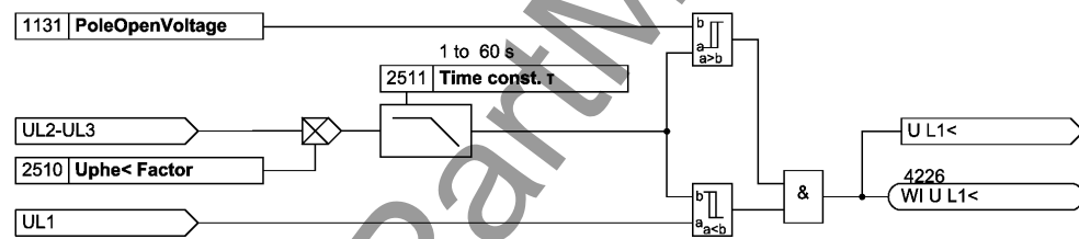
Figure 2-95 Undervoltage Detection for U_{L1-E}
