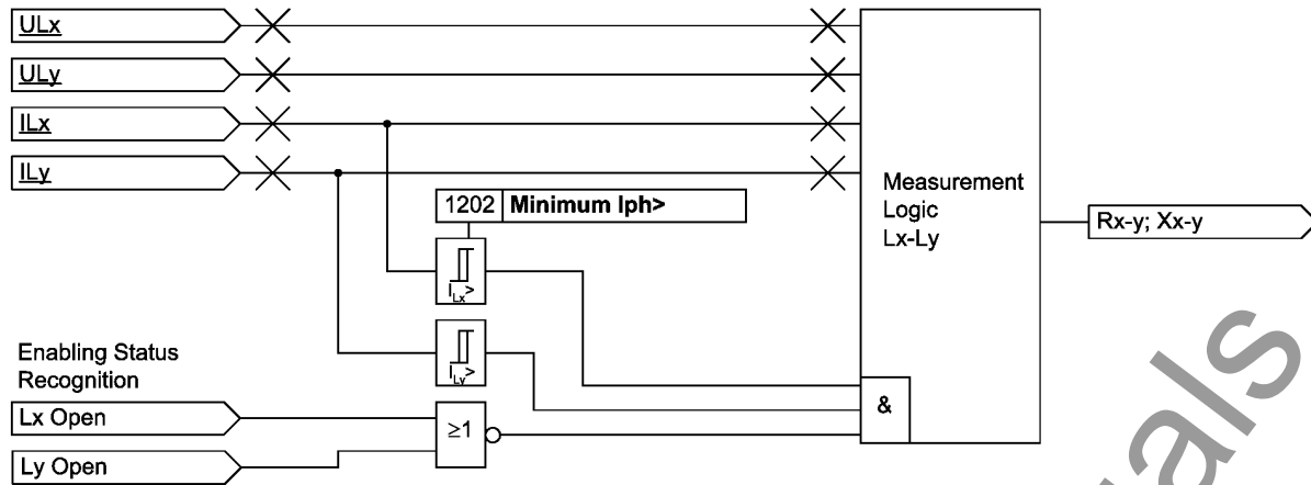
Figure 2-14 Logic of the phase-phase measuring system
