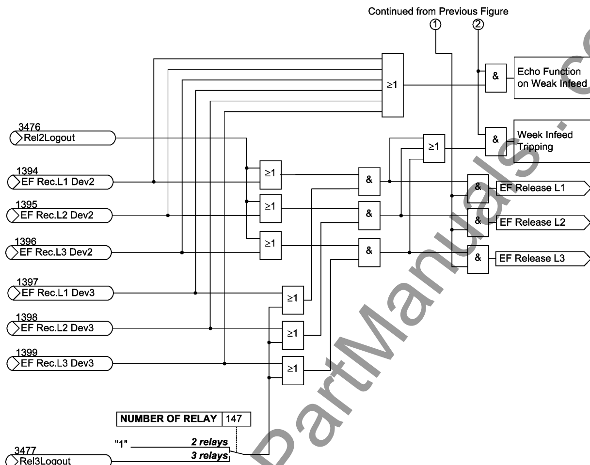
Figure 2-82 Logic diagram of the directional comparison scheme with protection data interface (for one device) — continued
