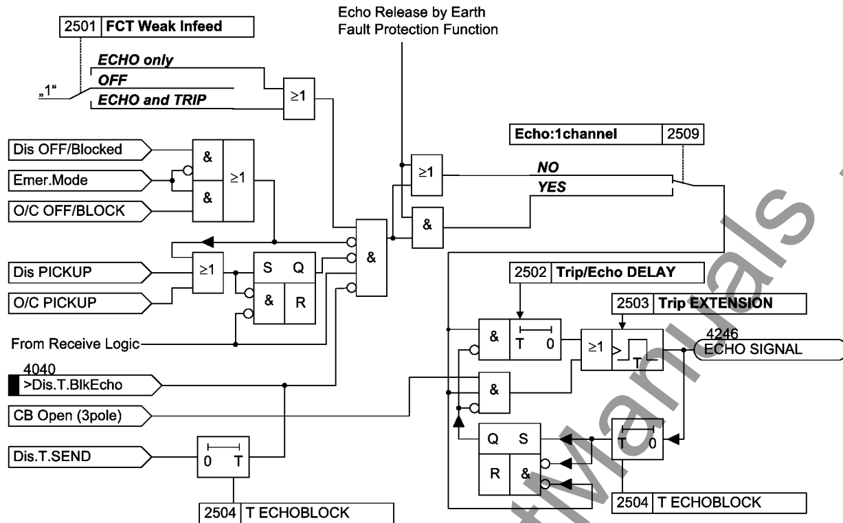
Figure 2-65 Logic diagram of the echo function with distance protection with teleprotection
