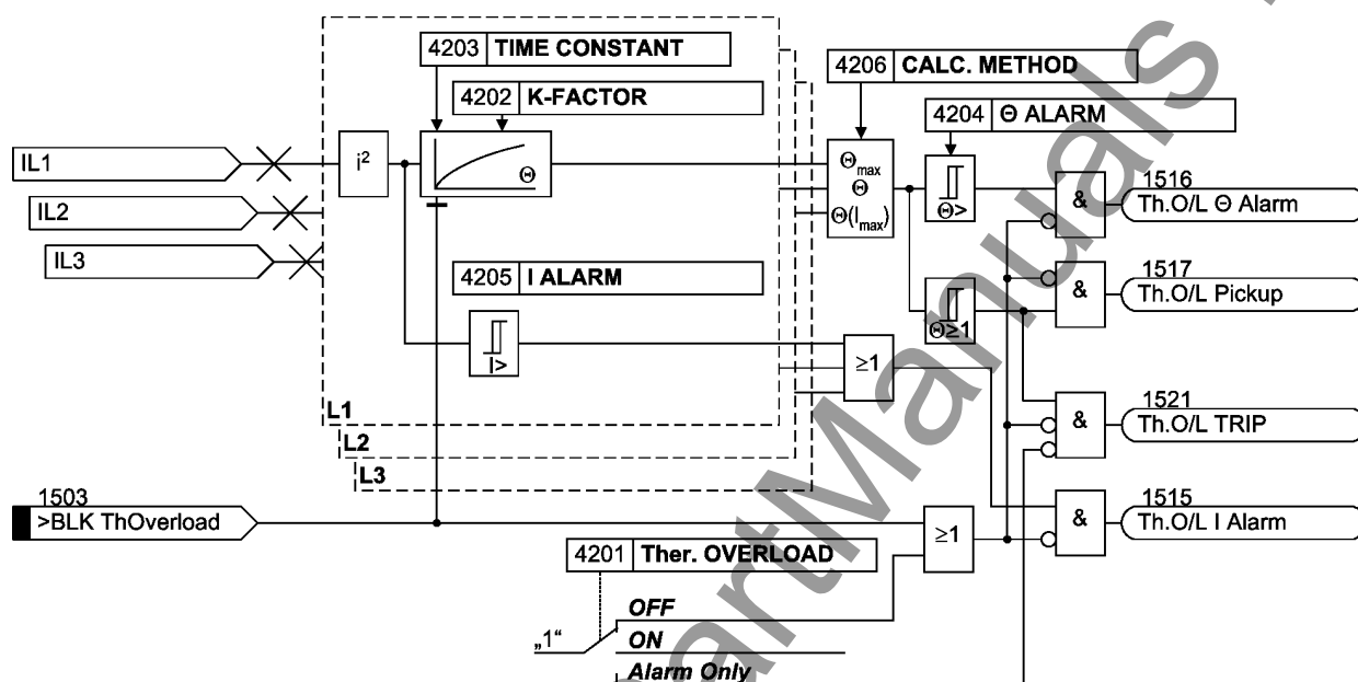
Figure 2-147 Logic diagram of the thermal overload protection
