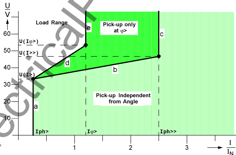
Figure 2-20 Parameters of the U/I/ \varphi pickup
