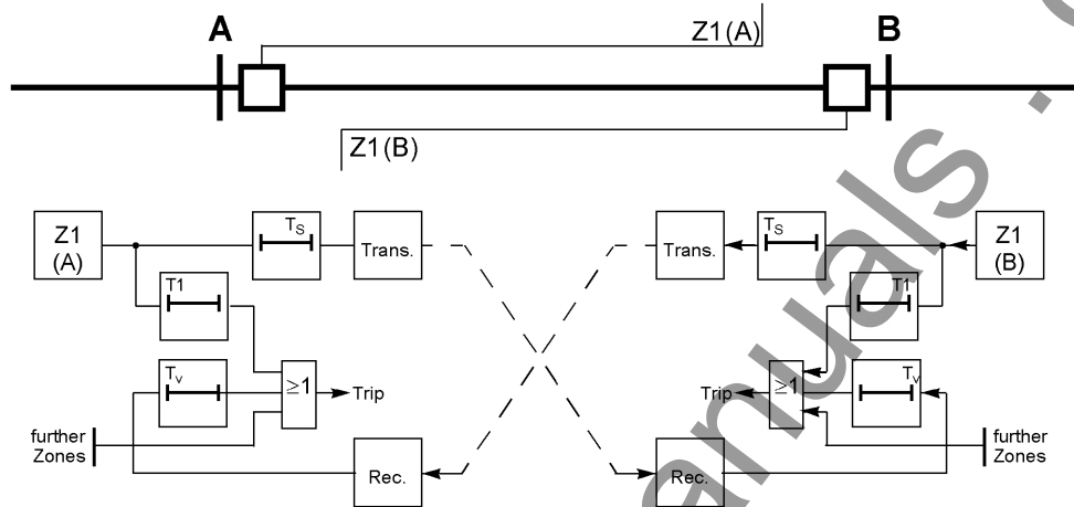
Figure 2-48 Function diagram of the direct underreach transfer trip scheme
