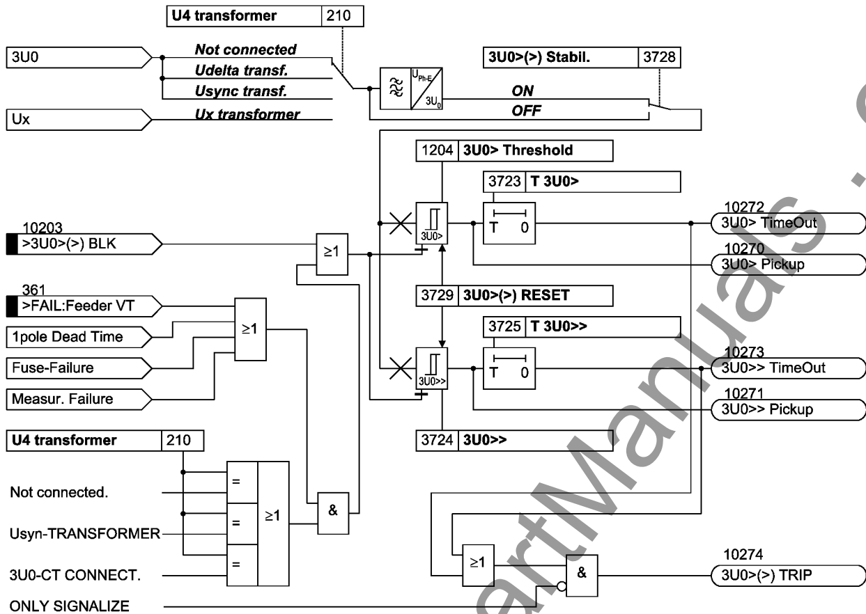
Figure 2-124 Logic diagram of the overvoltage protection for zero sequence voltage
