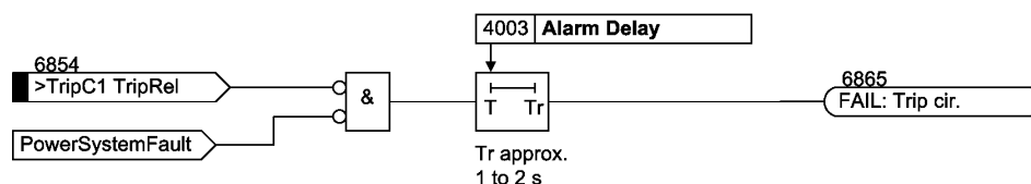
Figure 2-156 Logic diagram for trip circuit monitoring with one binary input
