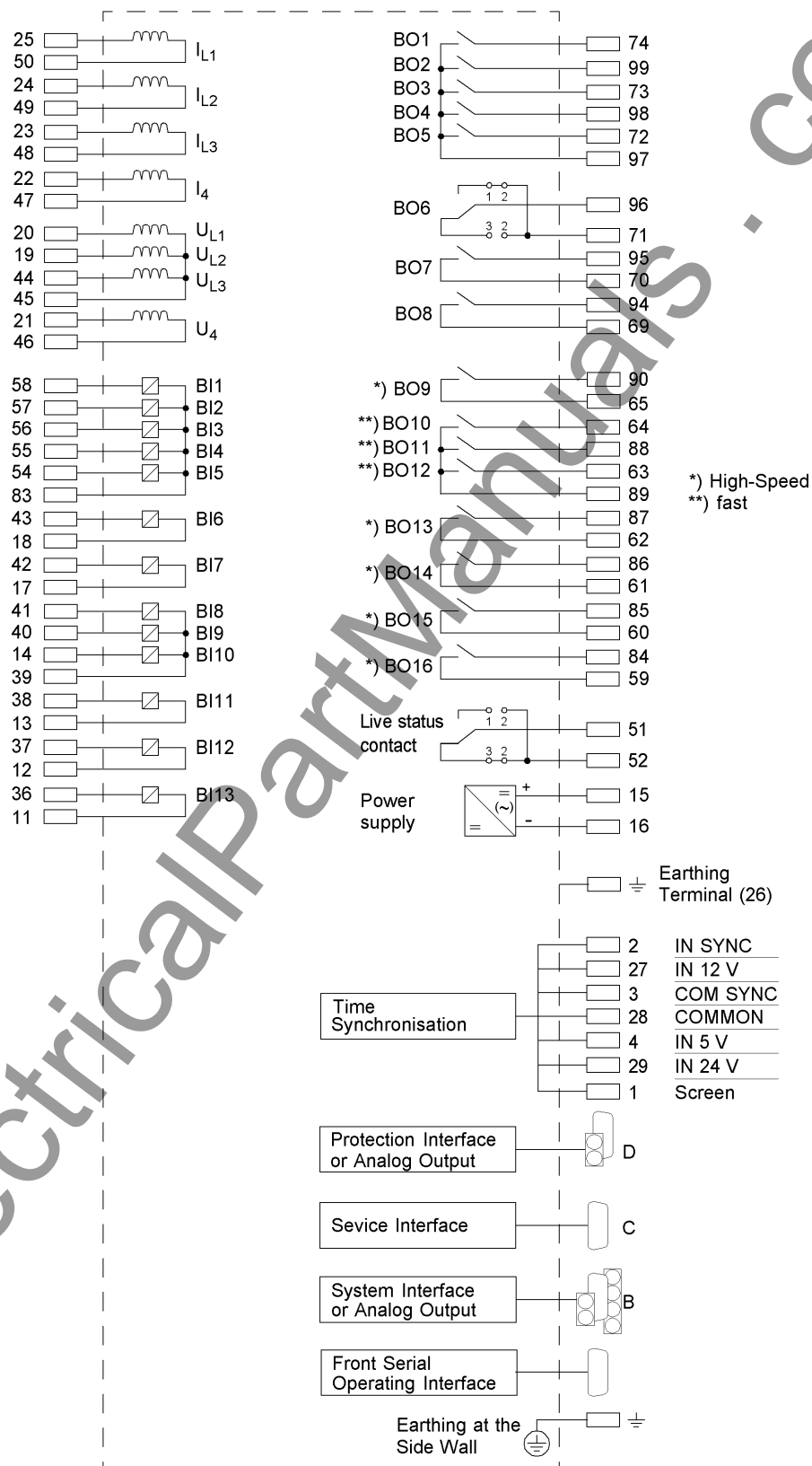
Figure A-17 General diagram for 7SA6*1*-*N (panel surface mounting)
