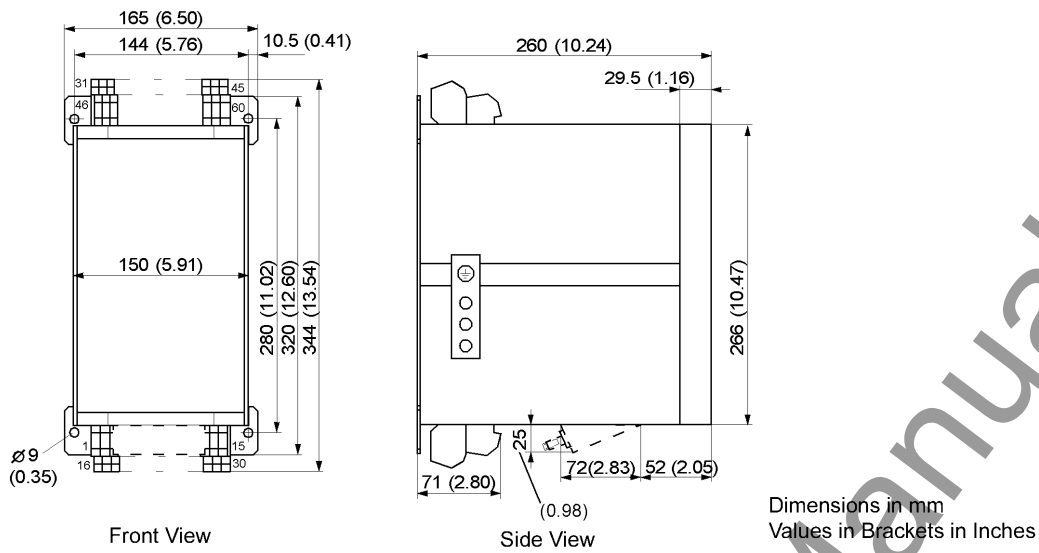
Figure 4-12 Dimensions of a device for panel surface mounting (size \frac{1}{3} )
