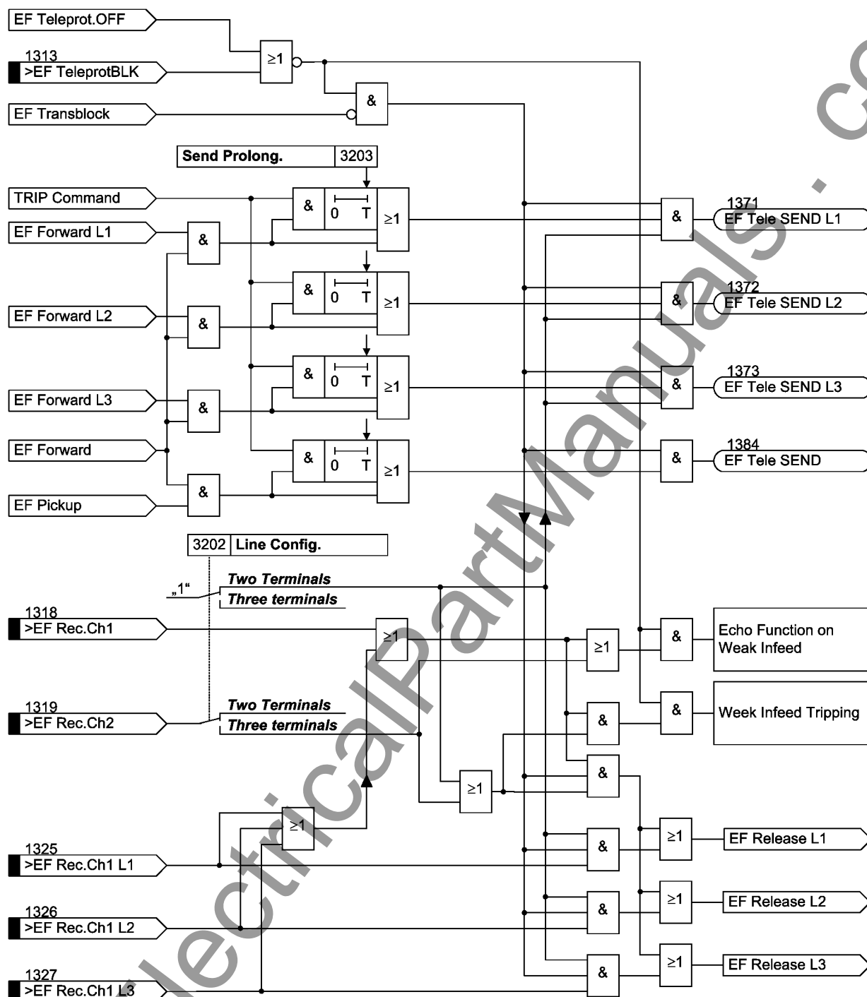
Figure 2-80 Logic diagram of the directional comparison scheme (one line end)
