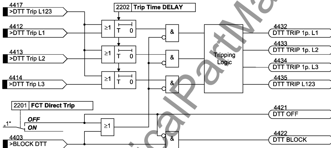
Figure 2-96 Logic diagram of the local external tripping
