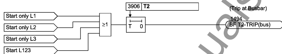
Figure 2-138 Single-stage breaker failure protection with common phase initiation
