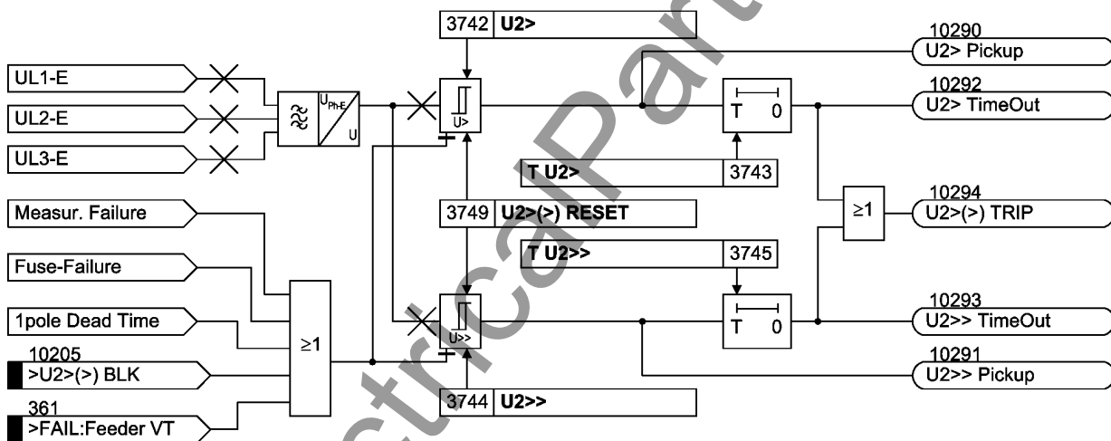
Figure 2-123 Logic diagram of the overvoltage protection for the negative sequence voltage system U_2
