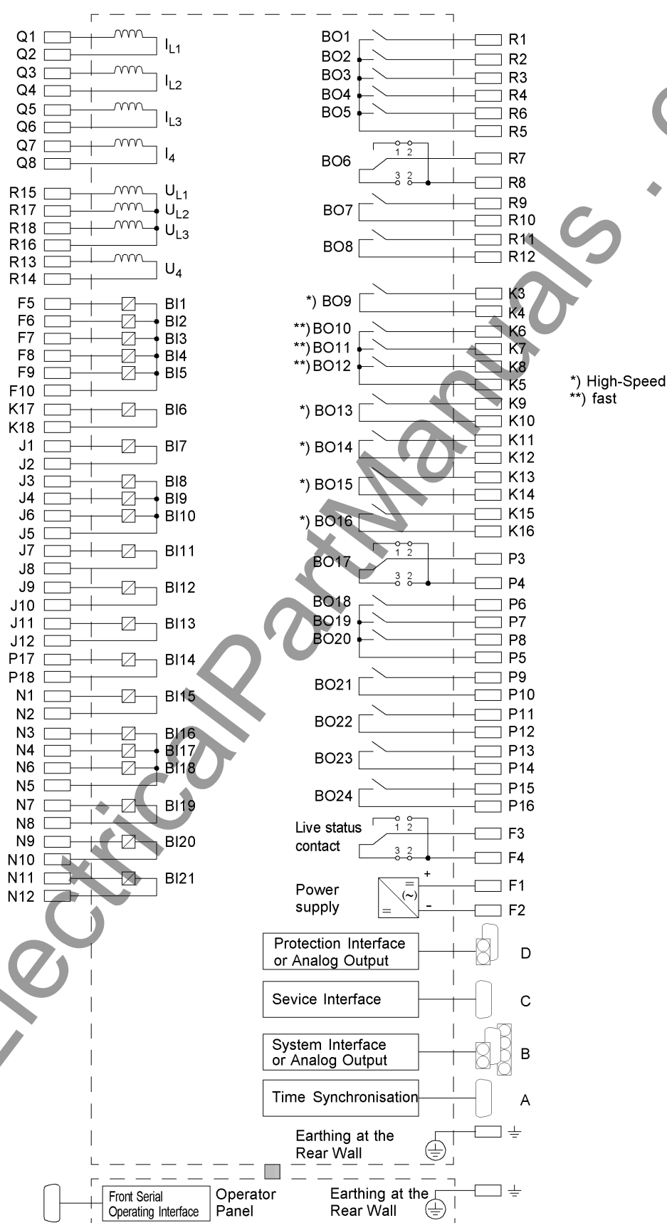
Figure A-29 General diagram 7SA642*-*M/R (panel surface mounting with detached operator panel)
