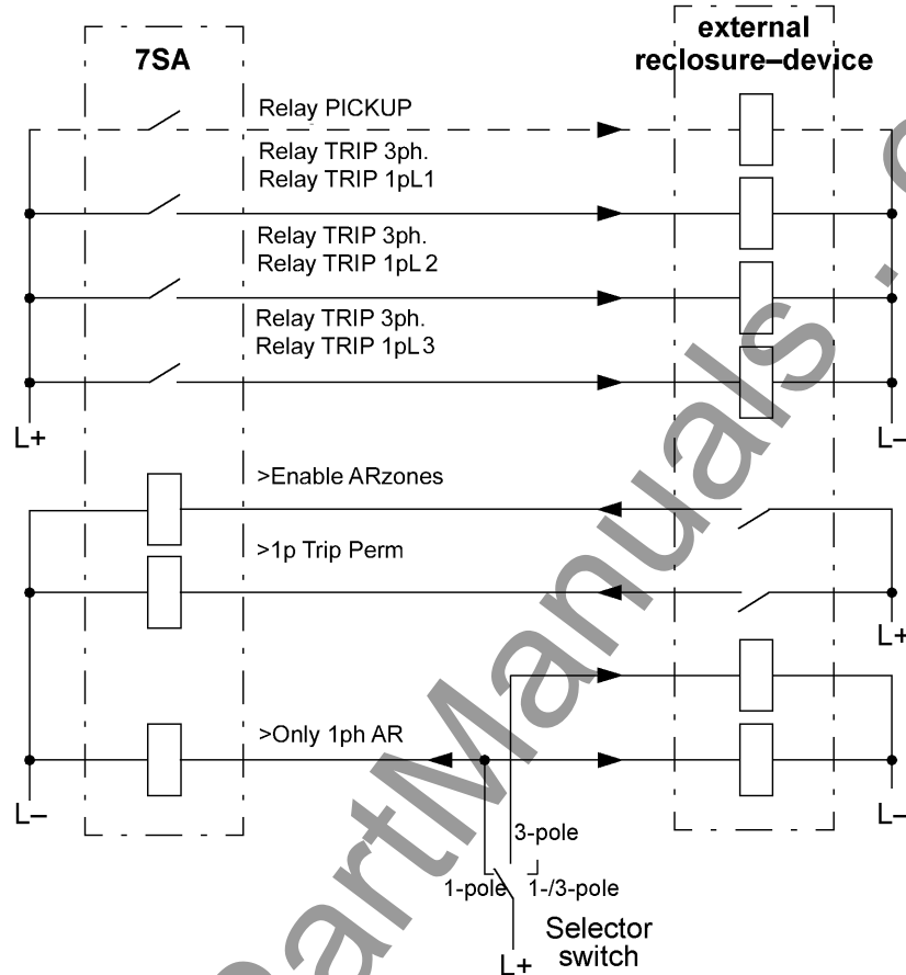
Figure 2-112 Connection example with external auto-reclosure device for 1-/3-pole AR with mode selector switch
