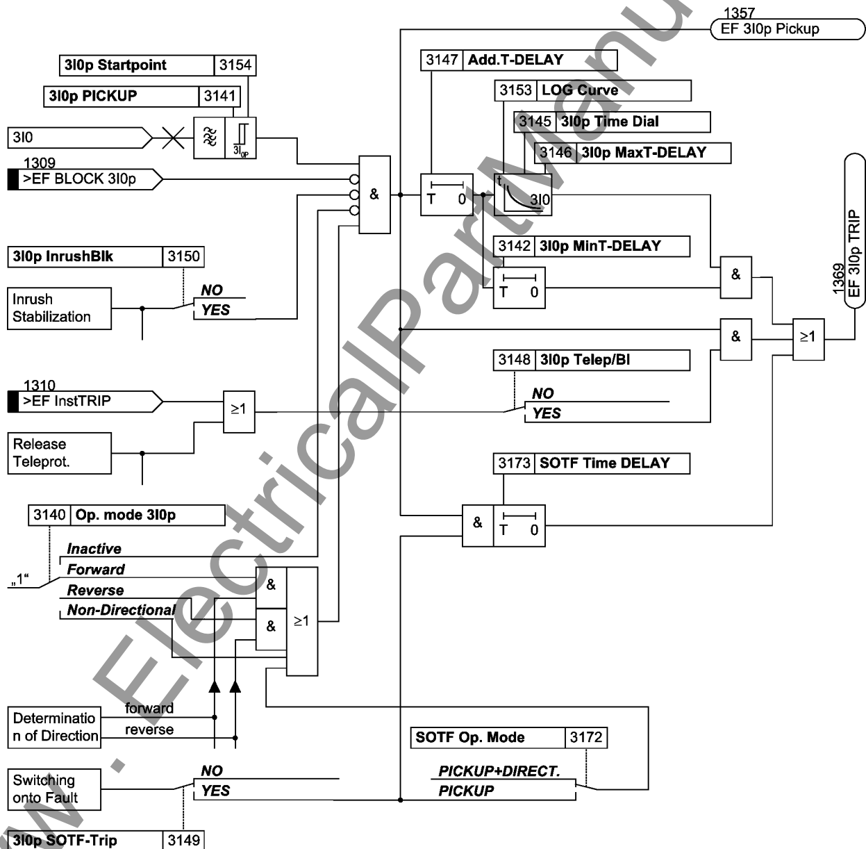
Figure 2-69 Logic diagram of the 3I 0p -stage for the inverse logarithmic characteristic
