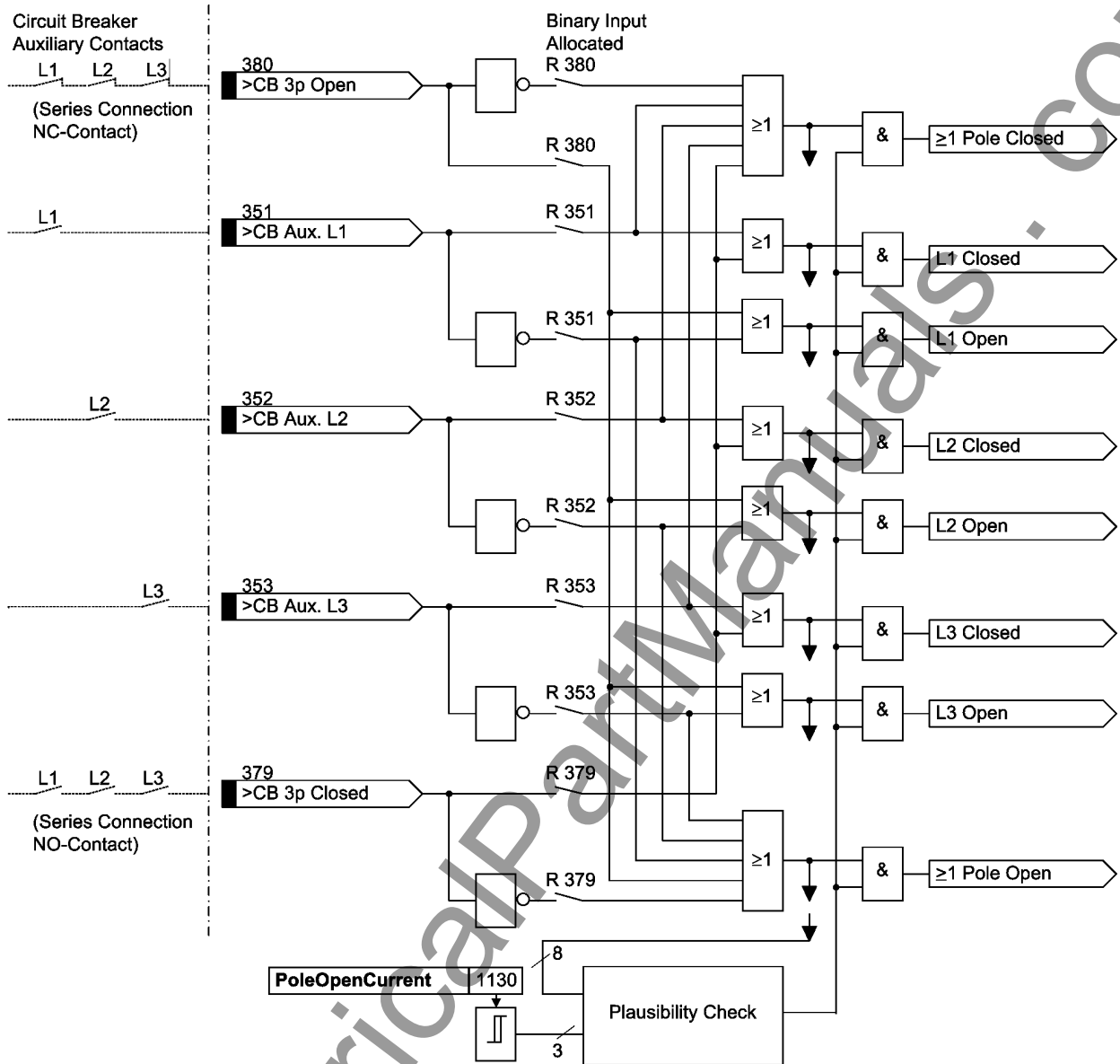
Figure 2-161 Circuit breaker position logic
