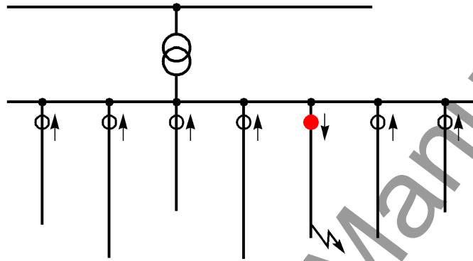
Figure 2-104 Earth fault location in a radial network
