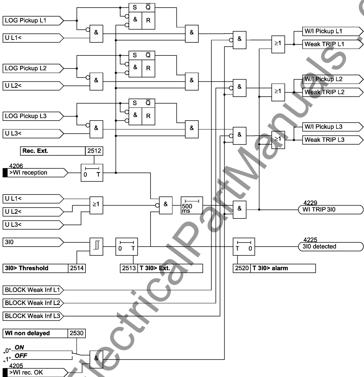
Figure 2-93 Logic diagram for non-delayed tripping
