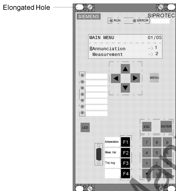
Figure 3-20 Example of panel flush mounting of a unit (housing size \frac{1}{3} )
