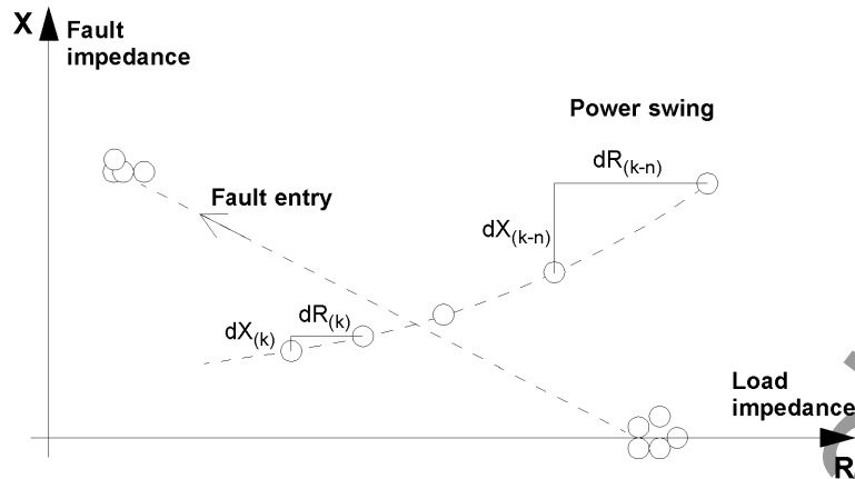
Figure 2-35 Impedance vector during power swing
