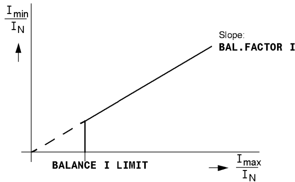
Figure 2-149 Current symmetry monitoring
