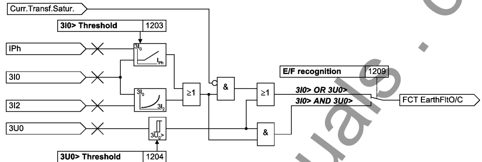
Figure 2-9 Logic of the earth fault detection
