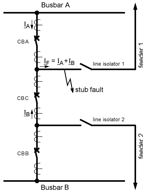
Figure 2-99 Stub fault at an 1½ circuit breaker arrangement
