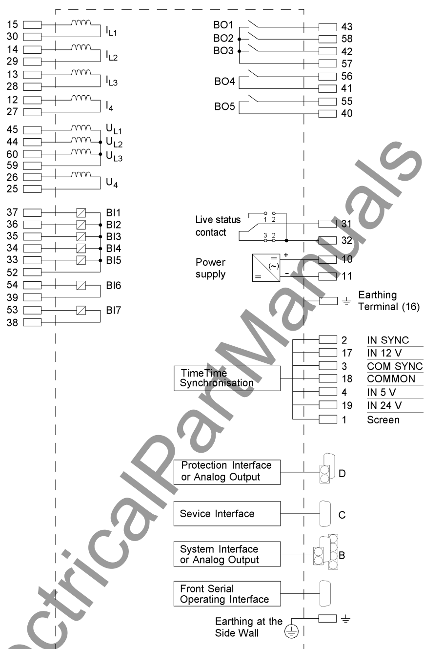
Figure A-14 General diagram for 7SA610*-*F (panel surface mounting)
