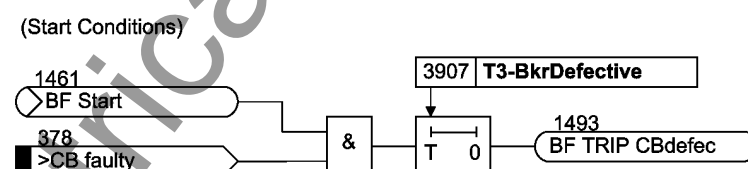
Figure 2-141 Circuit breaker faulty
