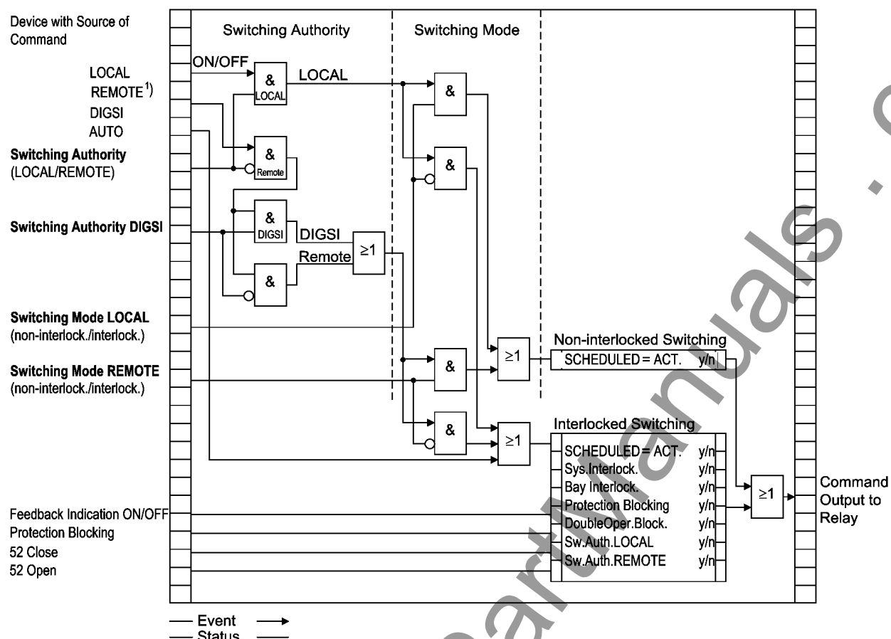
Figure 2-173 Standard interlockings
