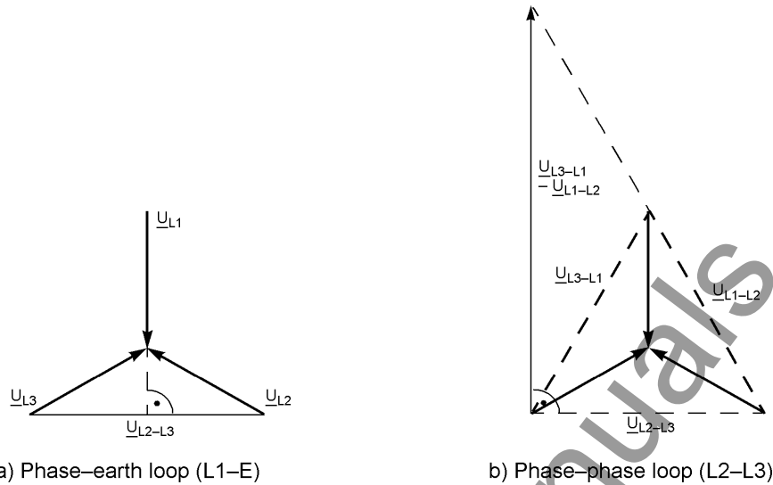
Figure 2-22 Direction determination with quadrature voltages
