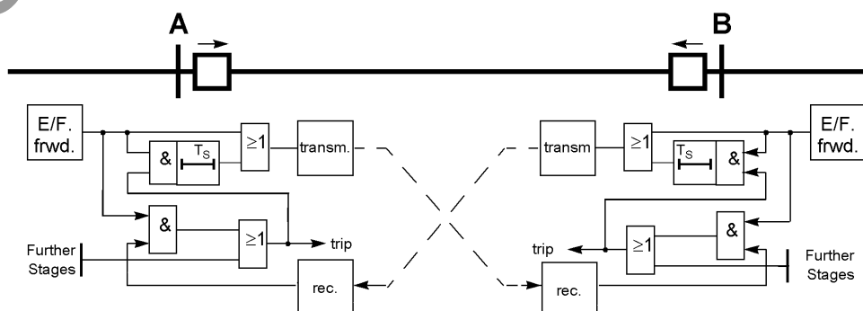
Figure 2-79 Operation scheme of the directional comparison pickup
