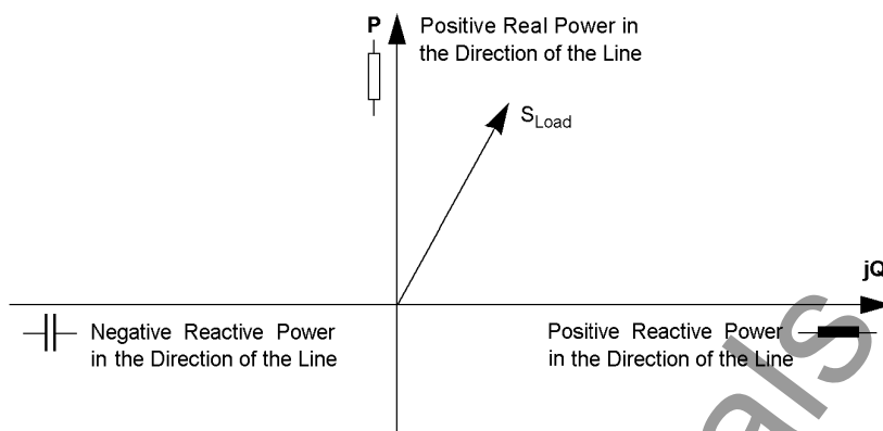
Figure 3-34 Apparent Load Power
