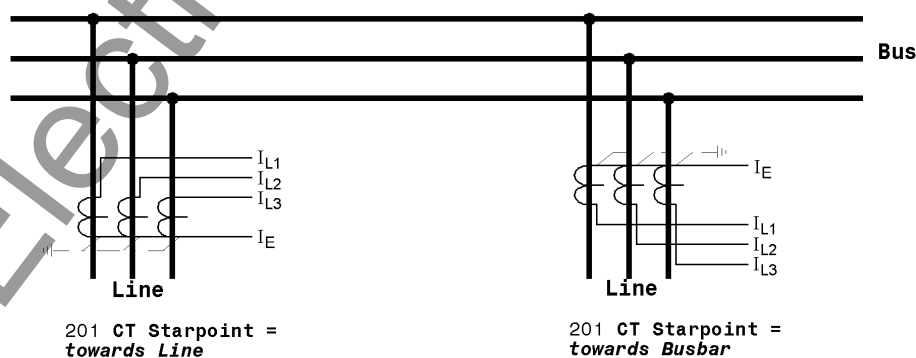
Figure 2-2 Polarity of Current Transformers
