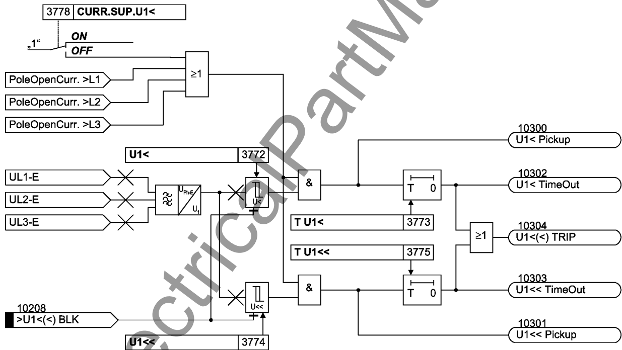
Figure 2-126 Logic diagram of the undervoltage protection for positive sequence voltage system
