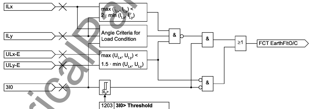
Figure 2-10 Earth fault detection during single-pole open condition
