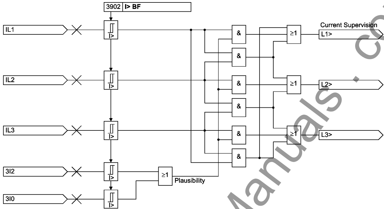
Figure 2-131 Current flow monitoring with plausibility currents 3 \cdot I_0 and 3 \cdot I_2
