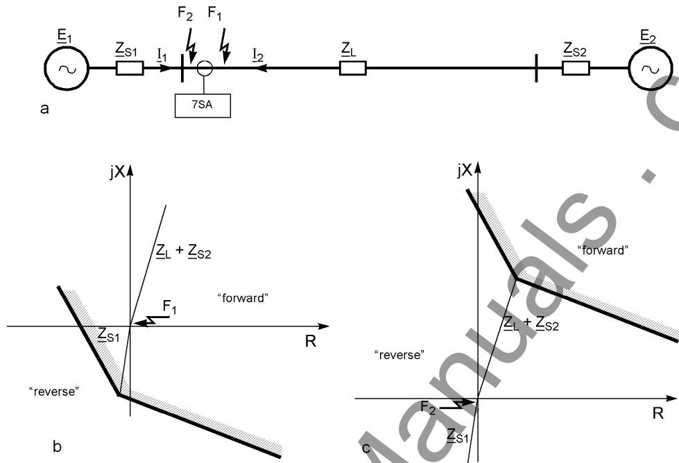
Figure 2-24 Directional characteristic with quadrature or memorized voltages
