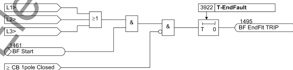
Figure 2-143 Operation scheme of end fault protection
