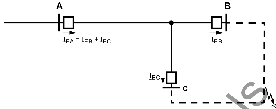
Figure 2-91 Possible unfavourable current distribution on a three terminal line during an external earth fault
