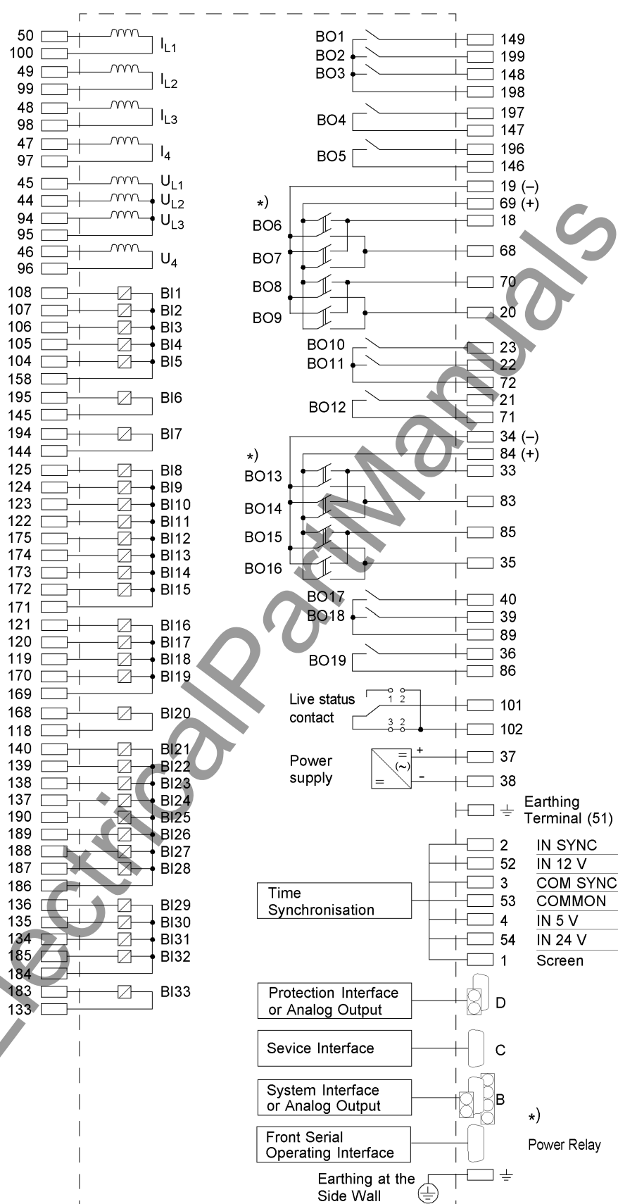
Figure A-20 General diagram for 7SA6*2*-*G (panel surface mounting)
