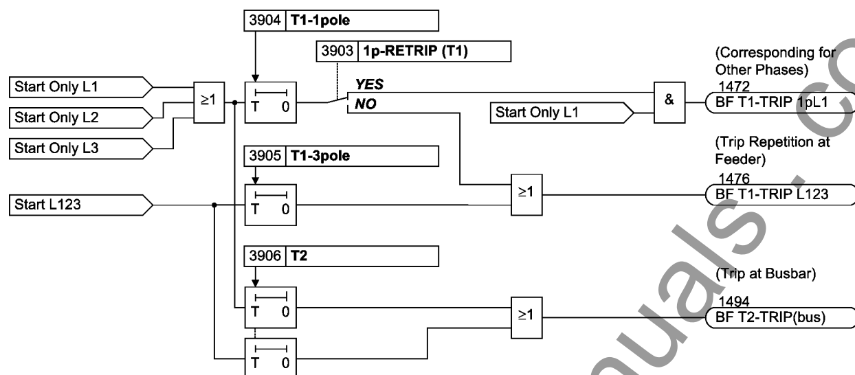
Figure 2-140 Two-stage breaker failure protection with phase segregated initiation
