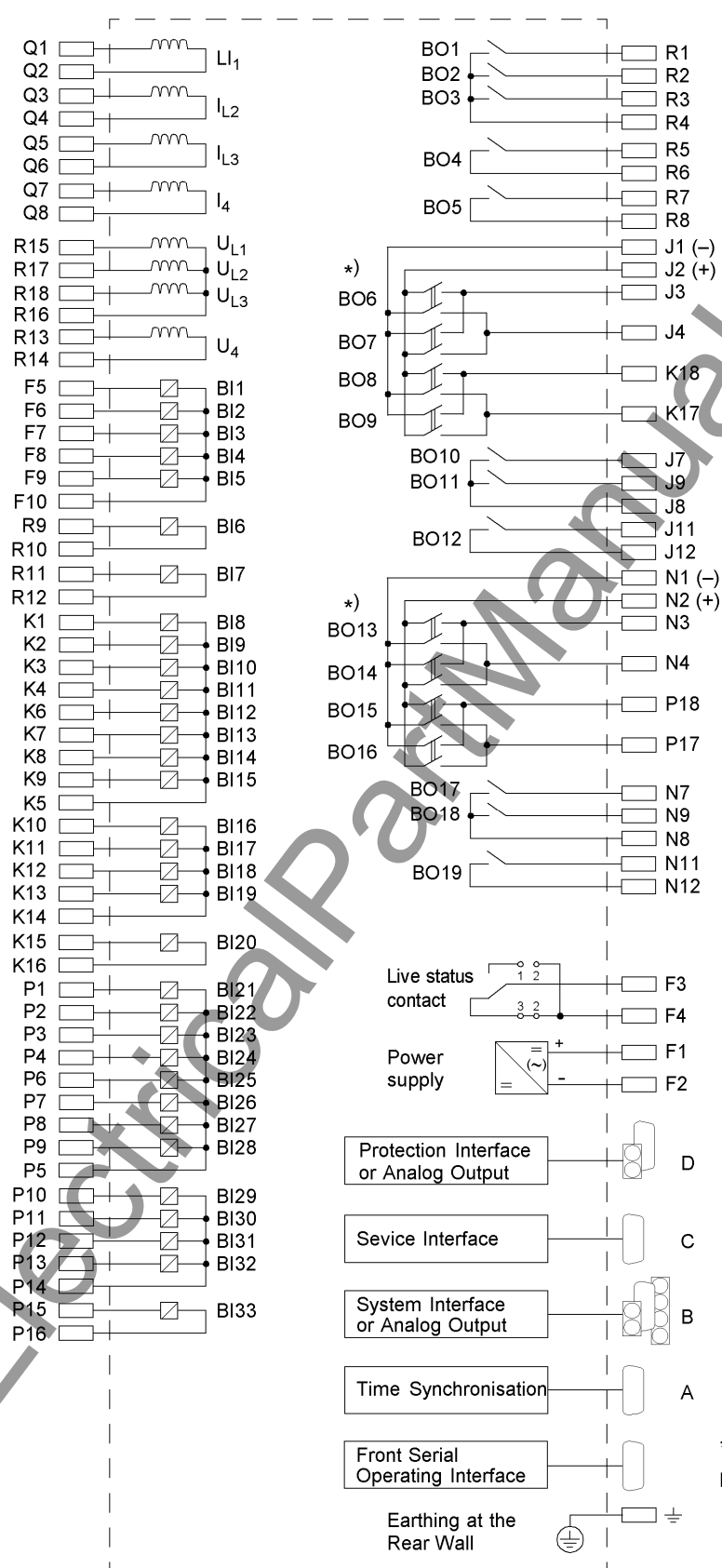
Figure A-10 General diagram for 7SA6*2*-*C/L (panel flush mounting or cubicle mounting)
