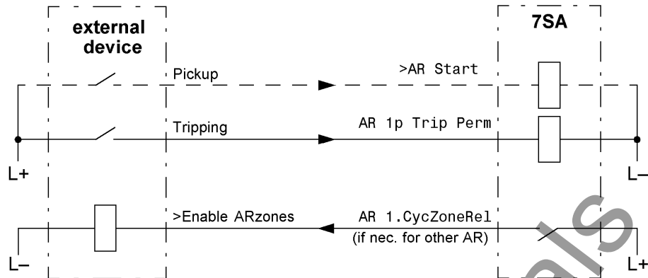
Figure 2-115 Connection example with external protection device for 3-pole reclosure; AR control mode = with TRIP
