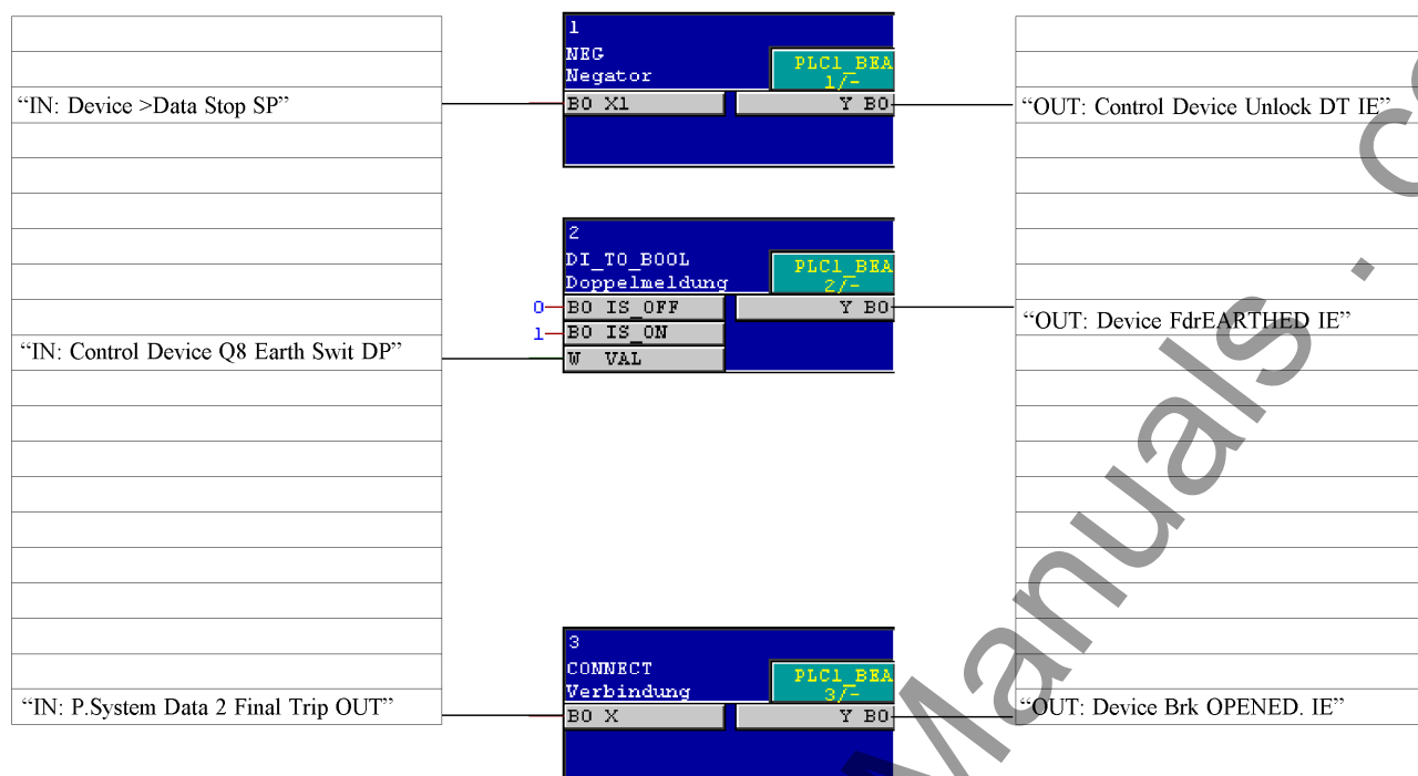
Figure A-51 Allocation of input and output with blocks of priority class System Logic
