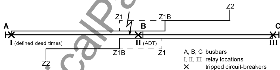
Figure 2-110 Example of adaptive dead time (ADT)
