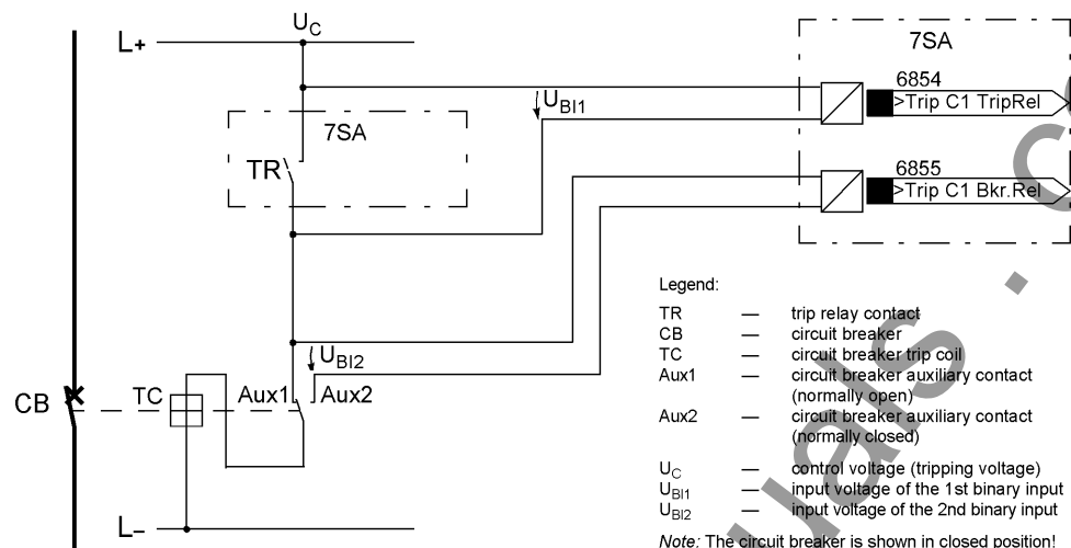
Figure 2-153 Principle of the trip circuit monitoring with two binary inputs
