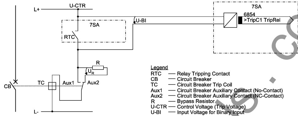
Figure 3-2 Trip circuit supervision with one binary input — Example for trip circuit 1
