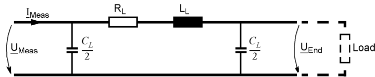
Figure 2-122 PI equivalent diagram for compounding
