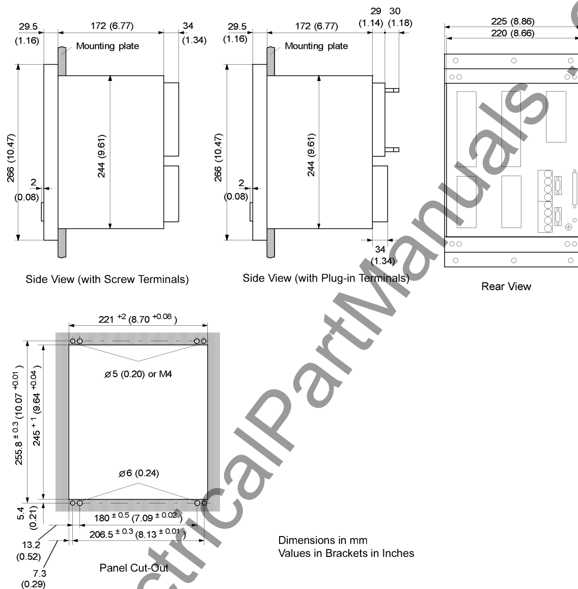
Figure 4-9 Dimensions of a device for panel flush or cubicle mounting (size 1\frac{1}{2} )
