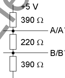
Figure 3-18 Termination of the RS485 interface (external)
