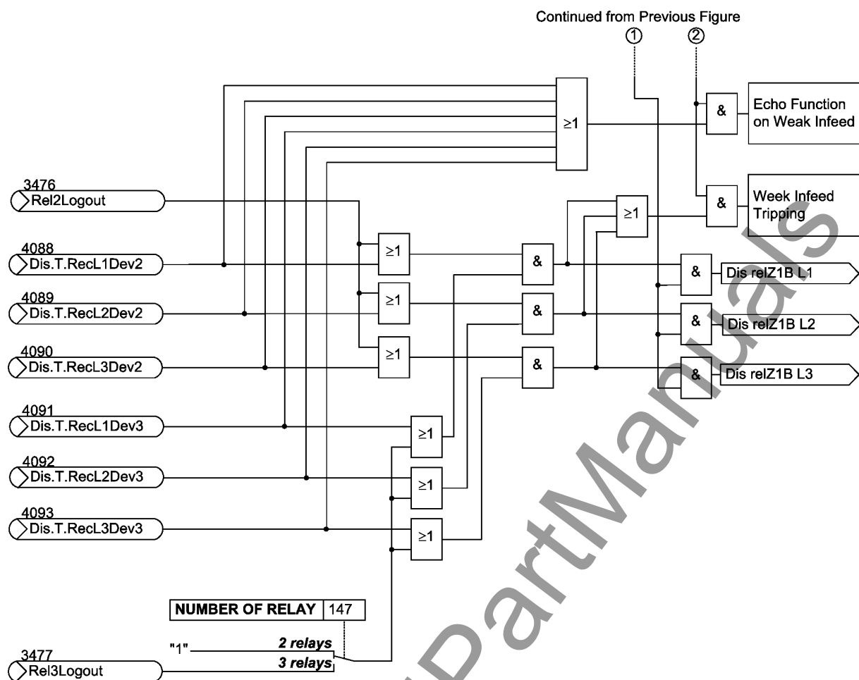
Figure 2-52 Logic diagram of the permissive overreach transfer trip (POTT) scheme with protection data interface - continued
