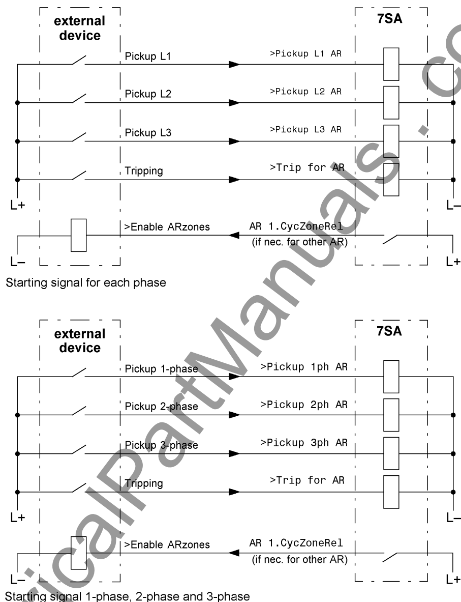
Figure 2-116 Connection example with external protection device for fault detection dependent dead time — dead time control by pickup signals of the protection device; AR control mode = with PICKUP
