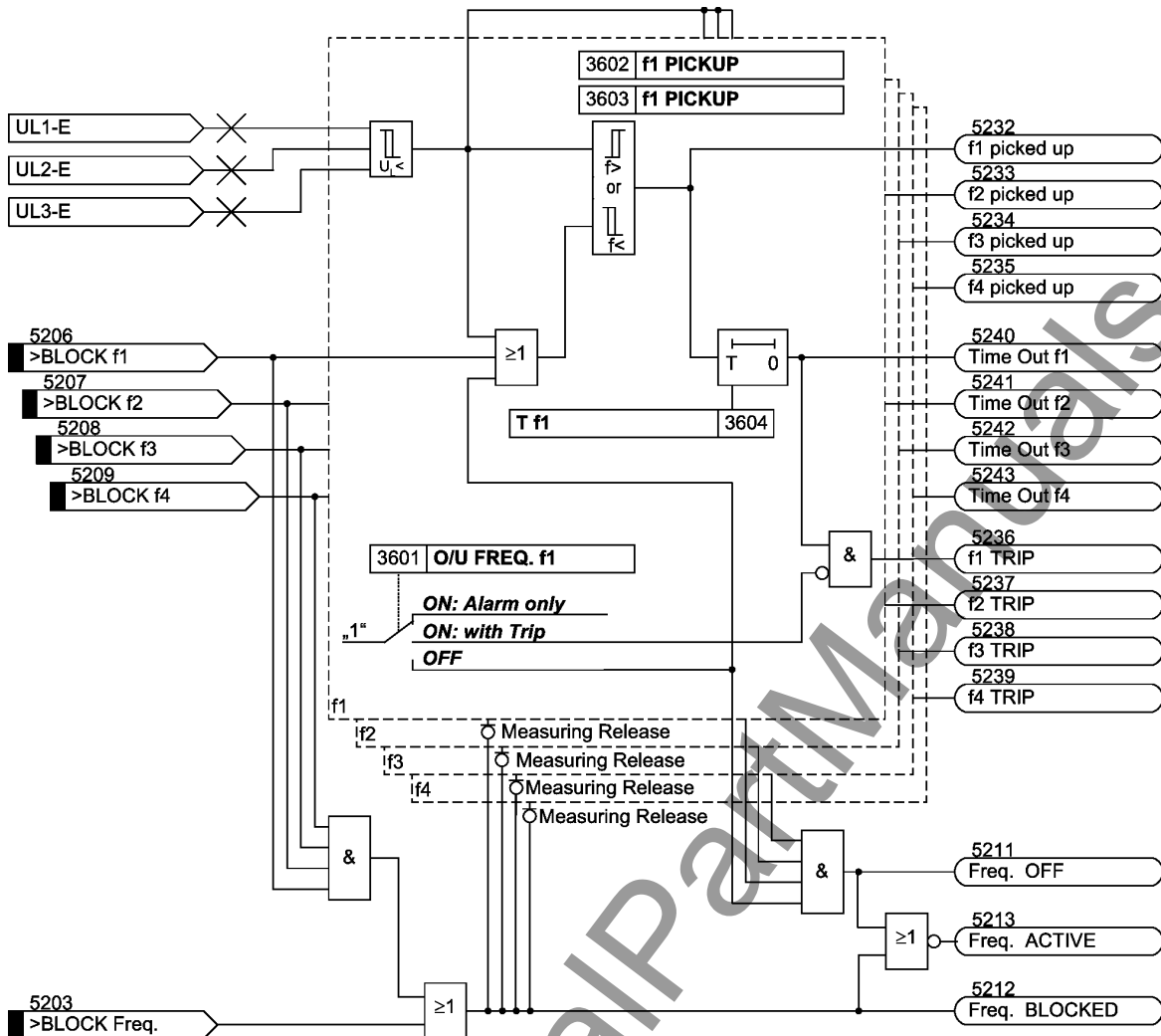
Figure 2-127 Logic diagram of frequency protection for 50 Hz rated frequency
