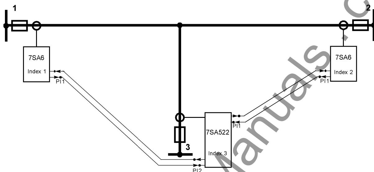
Figure 2-39 Distance protection for three ends with two 7SA6 and one 7SA522, chain topology
