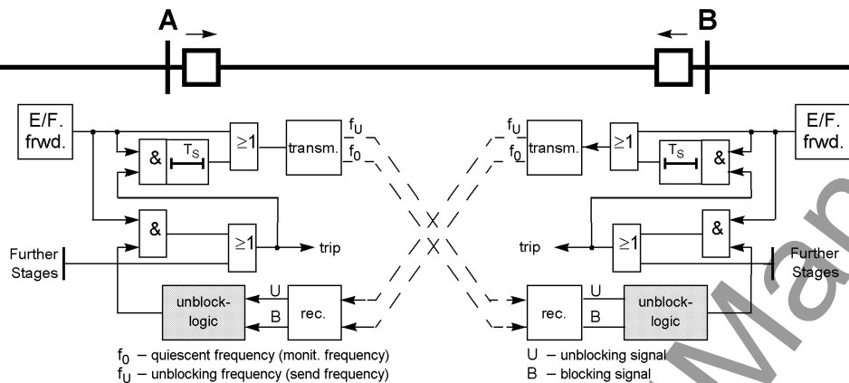
Figure 2-83 Operation scheme of the directional unblocking scheme
