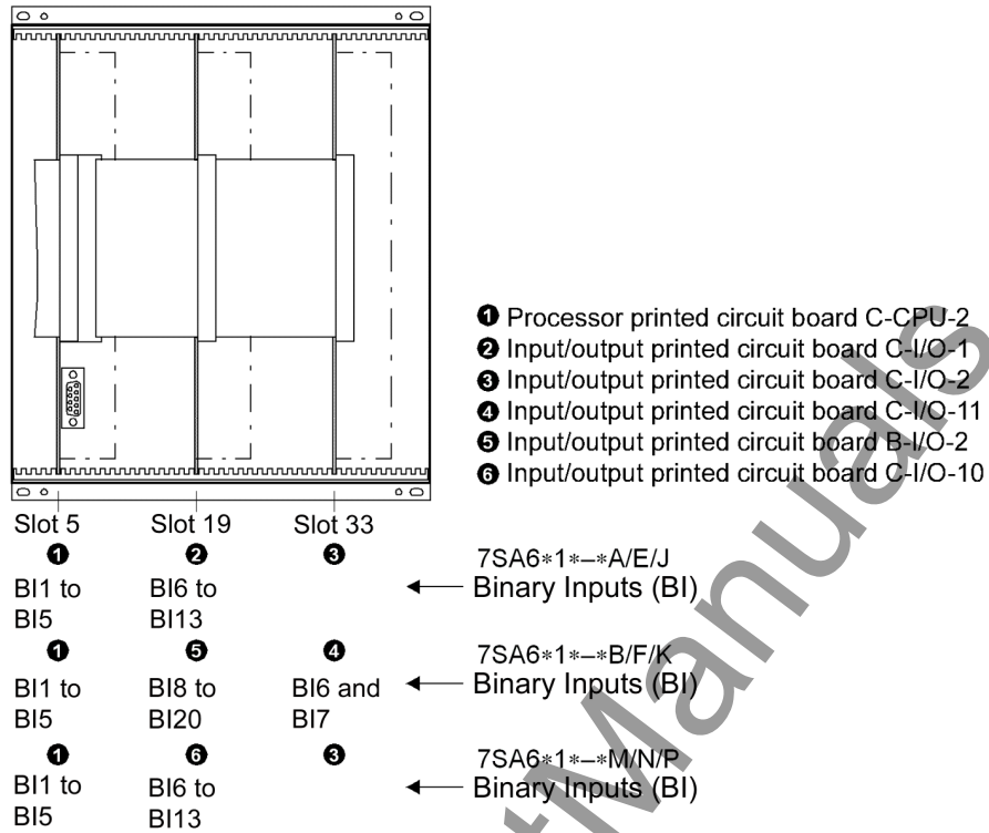
Figure 3-4 Front view with housing size \frac{1}{2} after removal of the front cover (simplified and scaled down)
