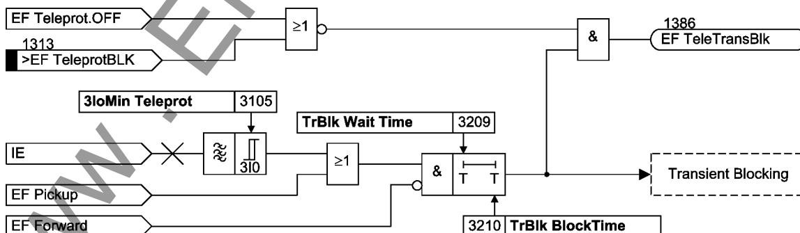
Figure 2-88 Transient blocking for a directional comparison and directional unblocking schemes
