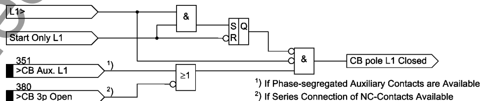
Figure 2-132 Interlock of the auxiliary contact criterion - example for phase L1
