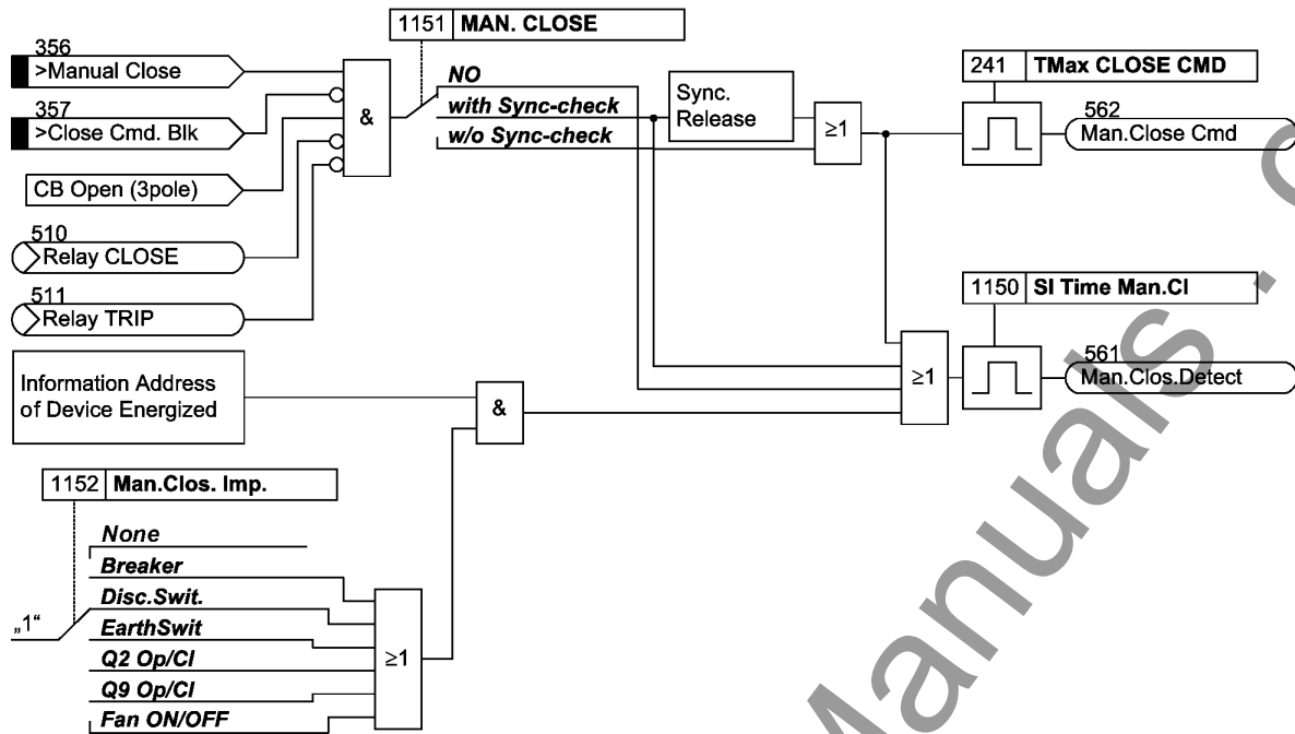
Figure 2-157 Logic diagram of the manual closing procedure
