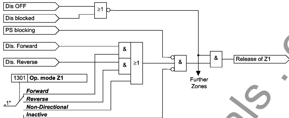
Figure 2-27 Release logic for one zone (example for Z1)
