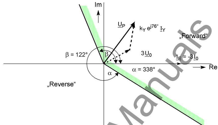
Figure 2-73 Directional characteristic of the earth fault protection
