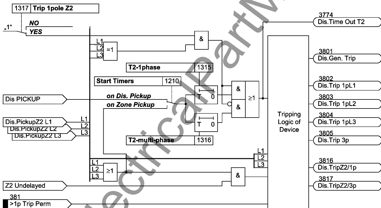
Figure 2-29 Tripping logic for the 2nd zone
