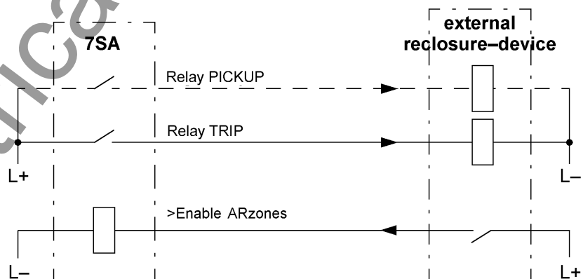
Figure 2-113 Connection example with external reclosure device for 3-pole AR
