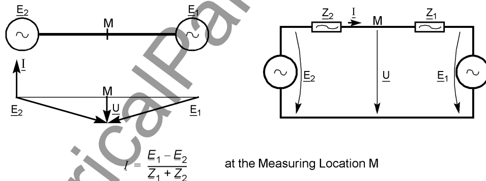
Figure 2-33 Power swing
