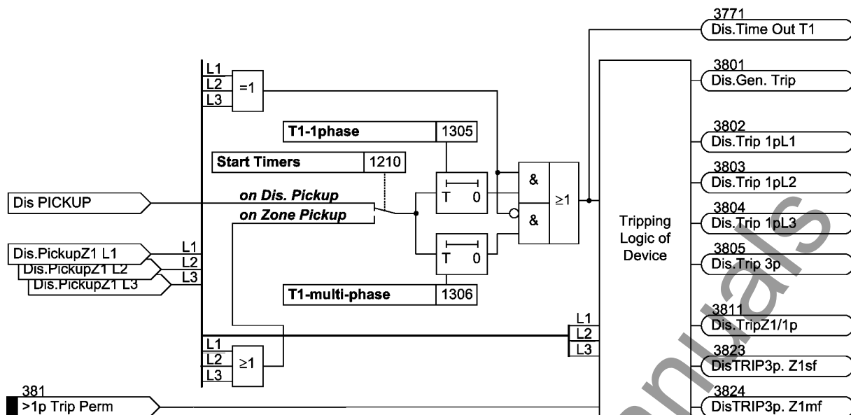
Figure 2-28 Tripping logic for the 1st zone
