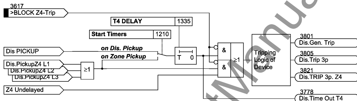
Figure 2-31 Tripping logic for the 4th and 5th zone, shown for Z4
