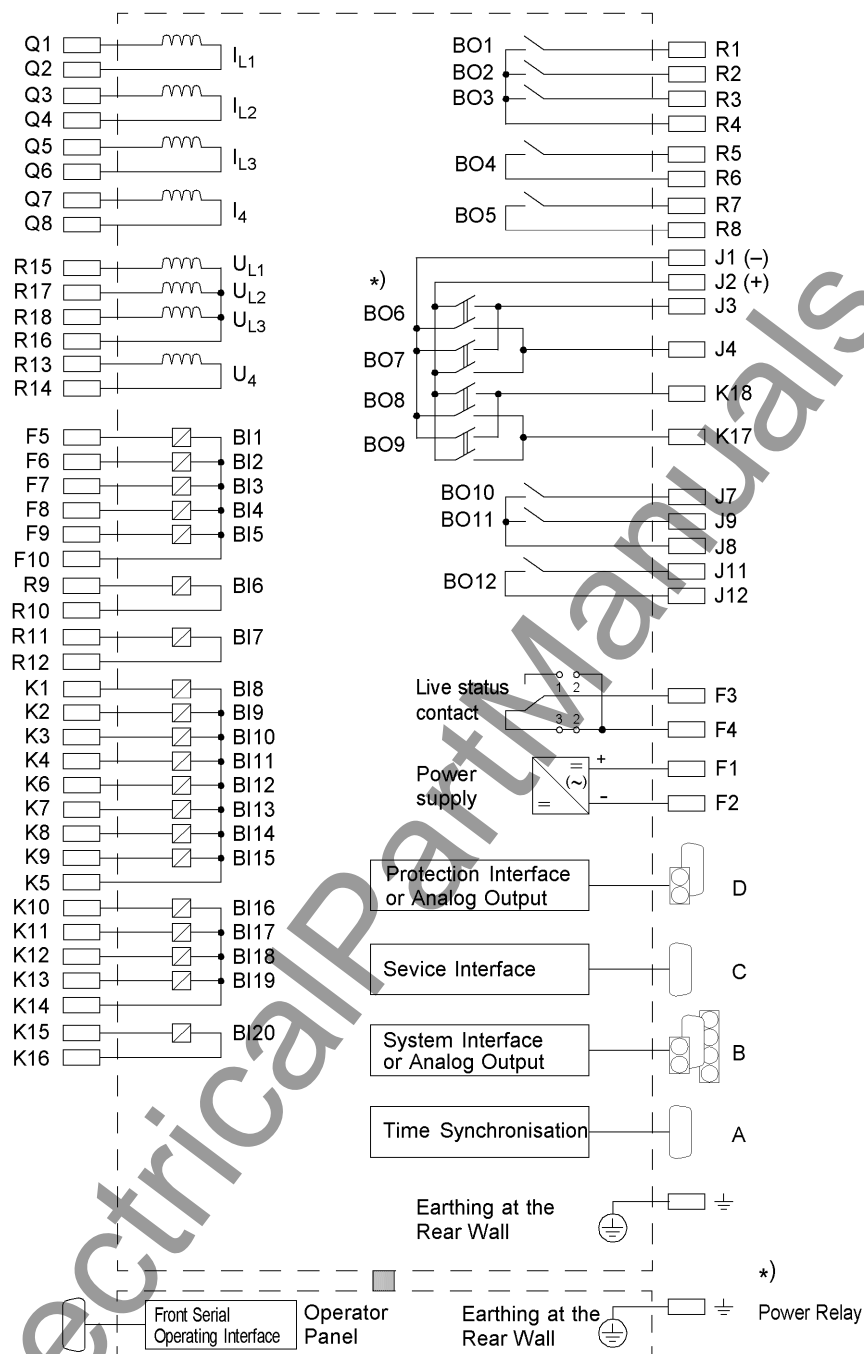
Figure A-24 General diagram 7SA641*-*B/K (panel surface mounting with detached operator panel)
