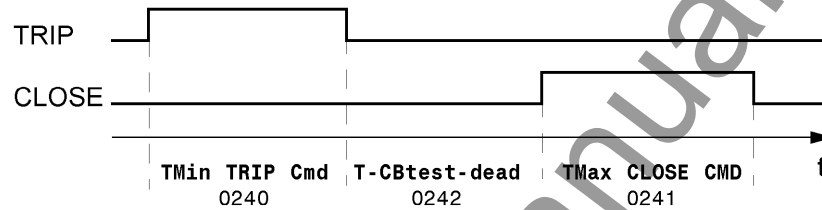
Figure 2-168 TRIP-CLOSE test cycle
