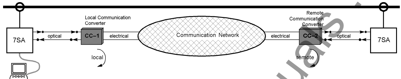
Figure 3-33 Distance protection communication via communication converter and communication network - example
