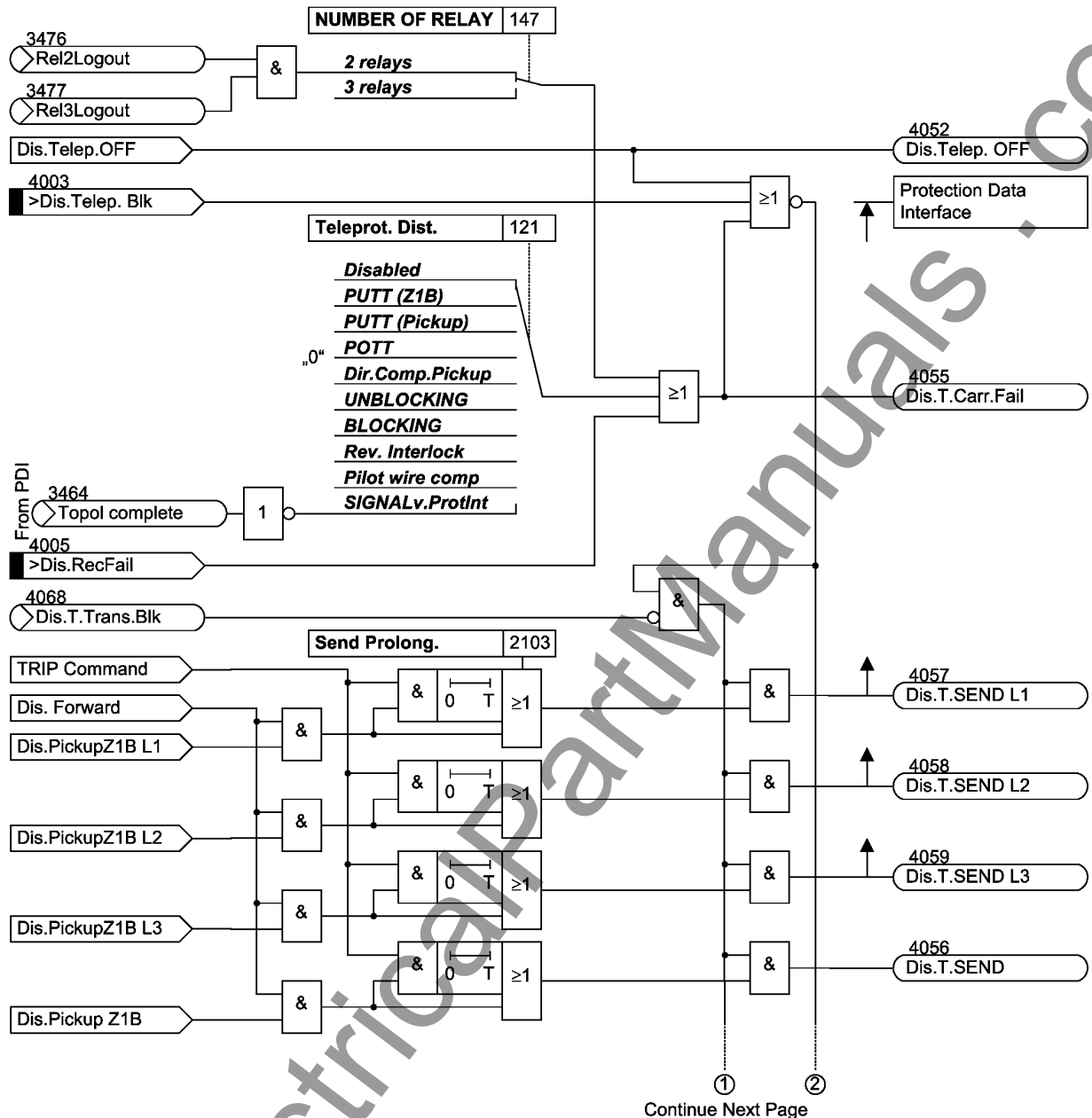
Figure 2-51 Logic diagram of the permissive overreach transfer trip (POTT) scheme (one line end, with protection data interface)
