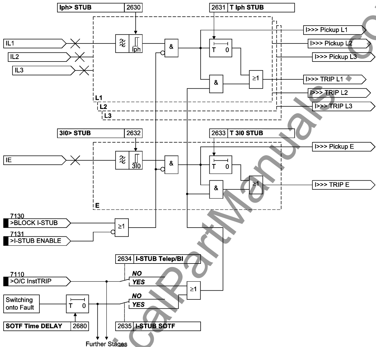
Figure 2-100 Logic diagram of stub fault protection
