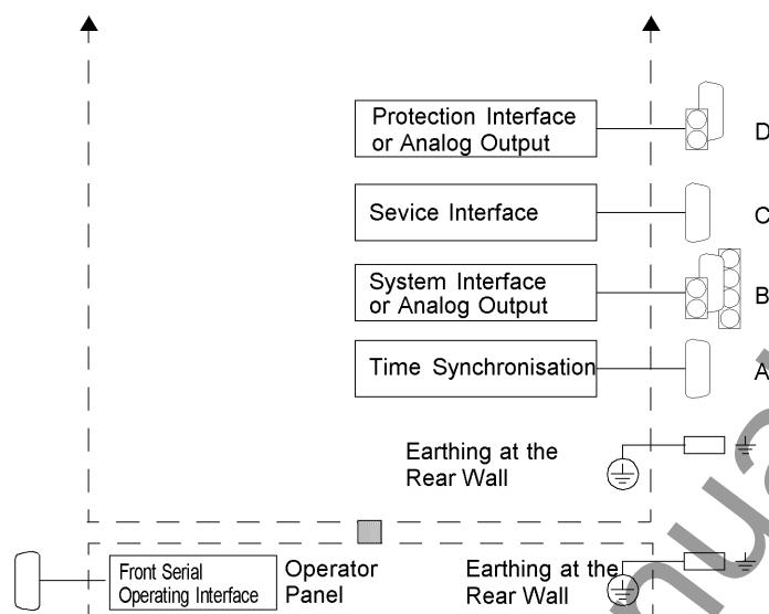
Figure A-27 General diagram 7SA642*-B/K (panel surface mounting with detached operator panel)
