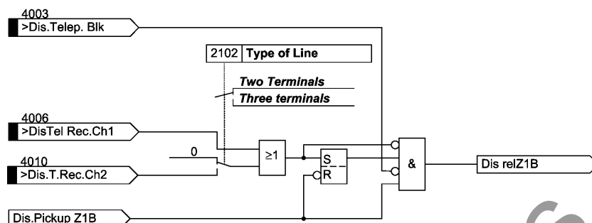
Figure 2-61 Receive circuit of pilot wire comparison logic
