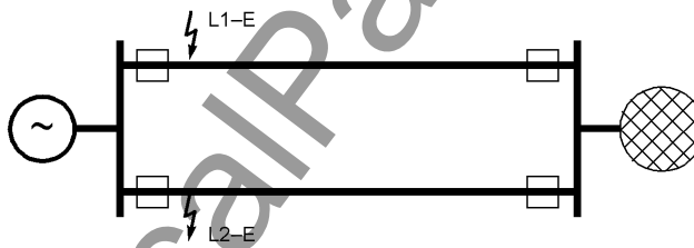
Figure 2-6 Multiple fault on a double-circuit line next to a generator
