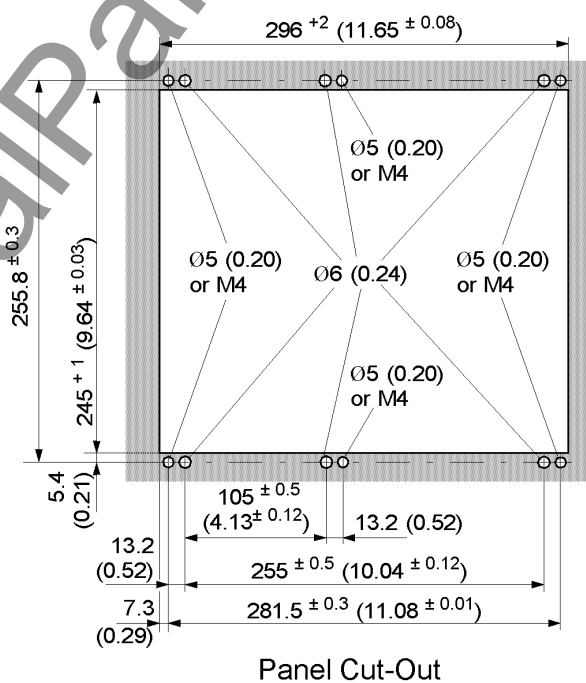
Figure 4-10 Dimensions of a device for panel flush mounting or cubicle installation (size 2\frac{2}{3} )
