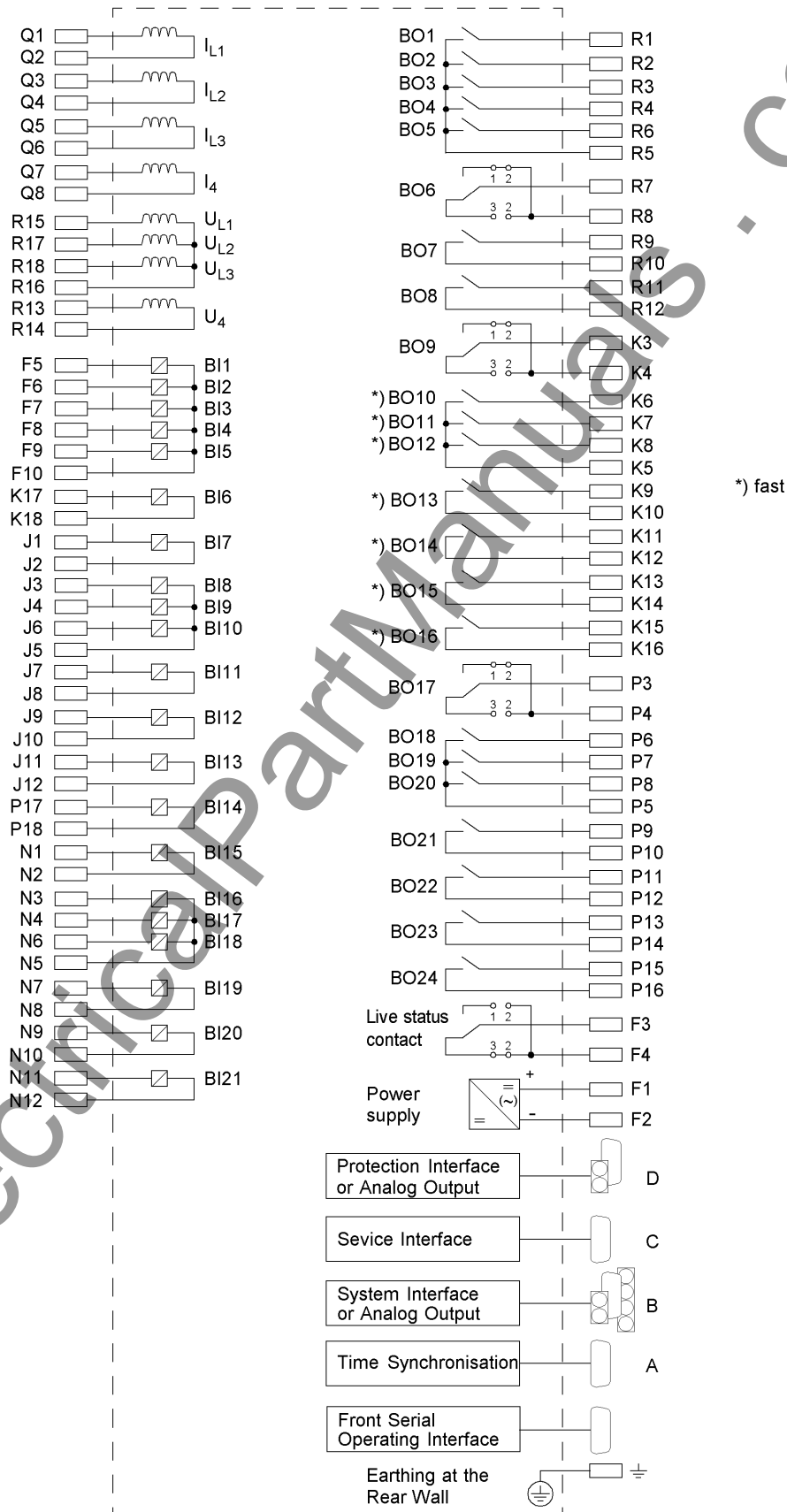
Figure A-11 General diagram for 7SA613*-A (panel flush mounting or cubicle mounting)
