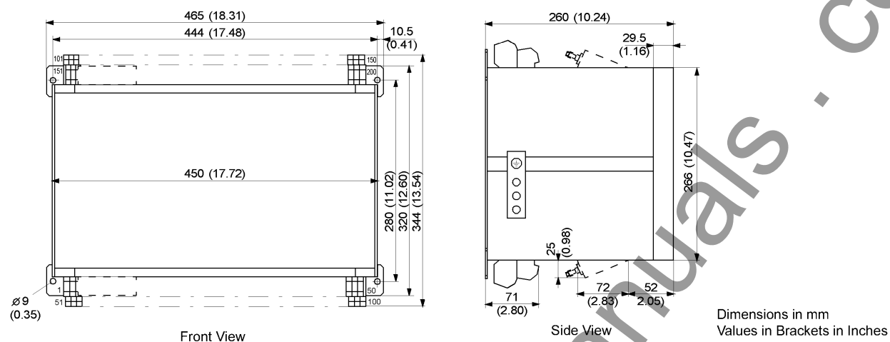
Figure 4-14 Dimensions of a device for panel surface mounting (size 1/1 )
