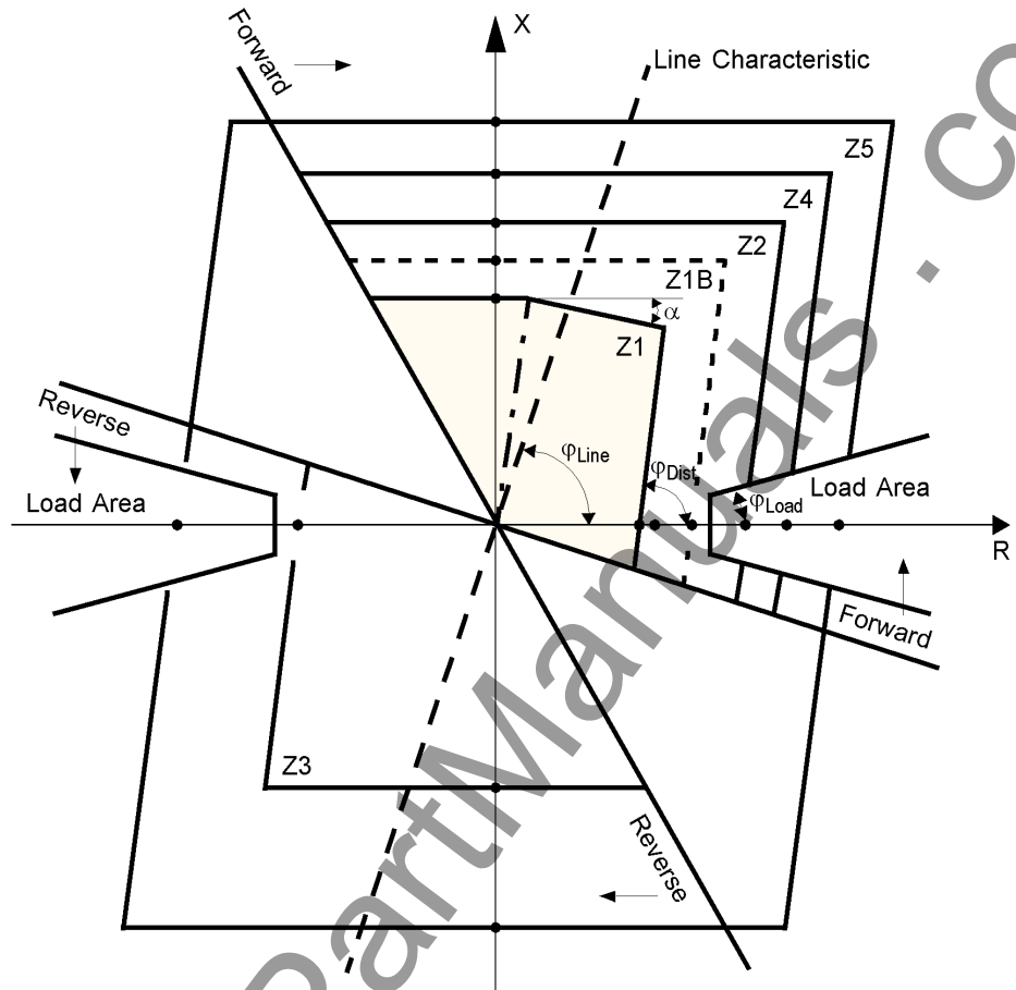
Figure 2-21 Polygonal characteristic (setting values are marked by dots)
