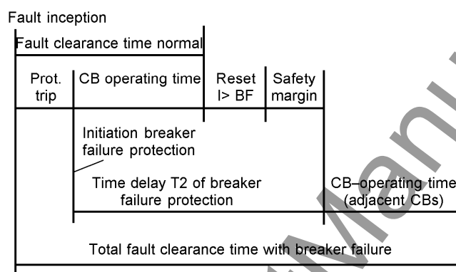
Figure 2-146 Time sequence example for normal clearance of a fault, and with circuit breaker failure, using single-stage breaker failure protection
