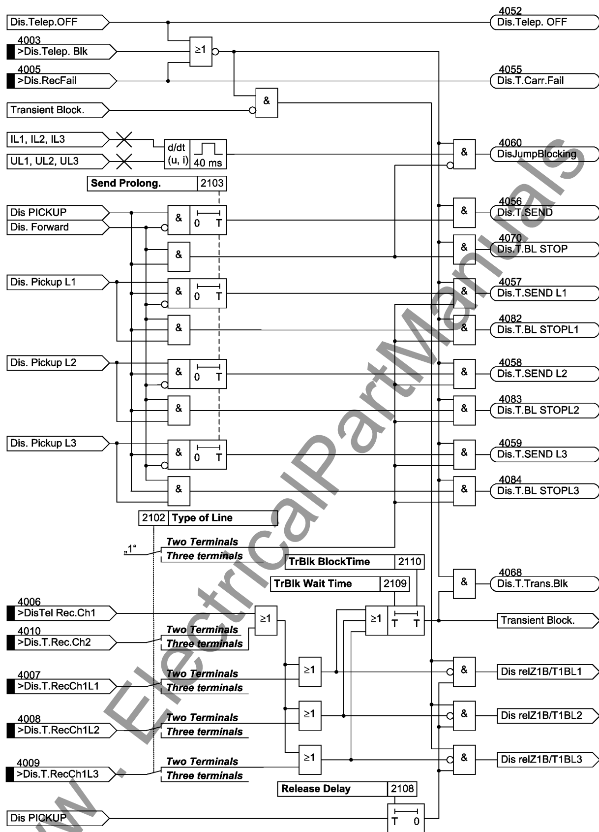
Figure 2-59 Logic diagram of the blocking scheme (one line end)
