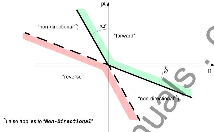
Figure 2-23 Directional characteristic in the R-X-diagram
