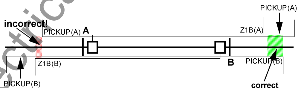
Figure 2-66 Distance protection setting with permissive overreach schemes
