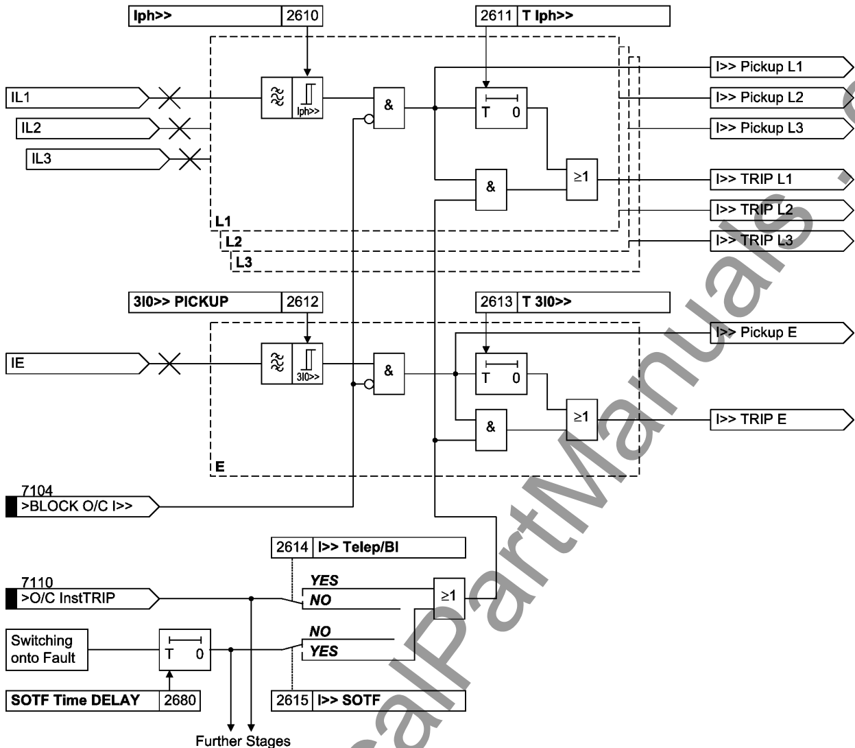
Figure 2-97 Logic diagram of the I&gt;&gt; stage
