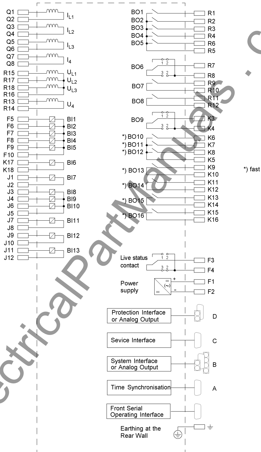
Figure A-3 General diagram for 7SA6*1*-*A/J (panel flush mounting or cubicle mounting)
