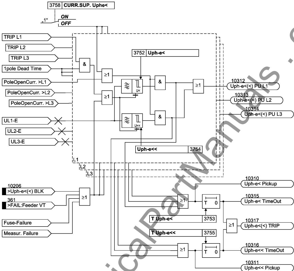
Figure 2-125 Logic diagram of the undervoltage protection for phase voltages
