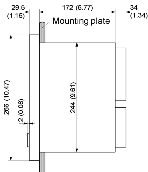
Side View (with Screw Terminals)
