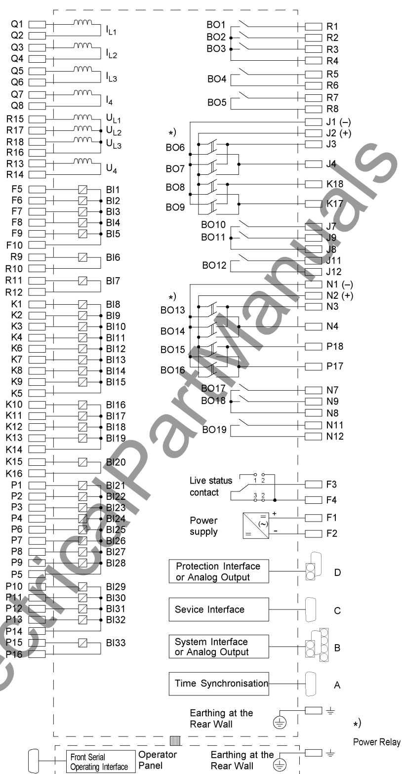
Figure A-28 General diagram 7SA642*-*C/L (panel surface mounting with detached operator panel)
