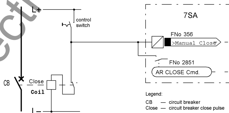
Figure 2-158 Manual closure with internal automatic reclosure
