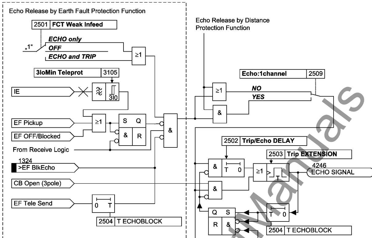
Figure 2-89 Logic diagram of the echo function for the earth fault protection with teleprotection
