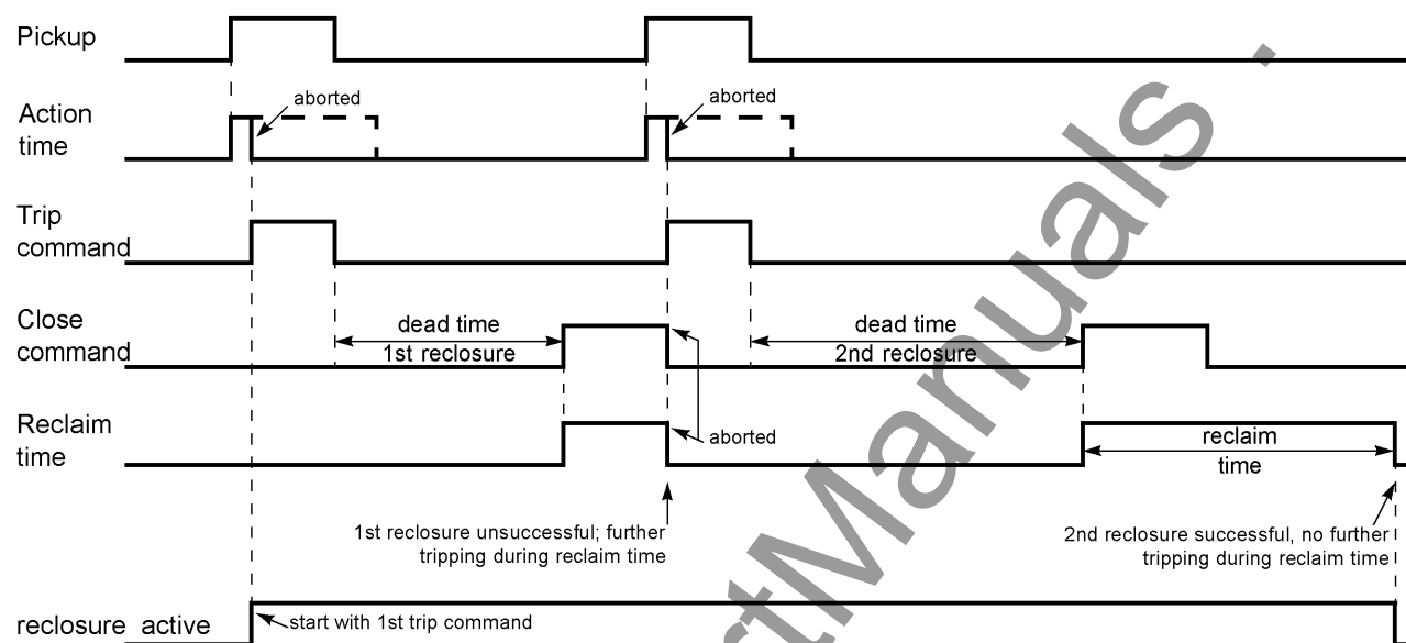
Figure 2-107 Timing diagram of a double-shot reclosure with action time (2nd reclosure successful)
