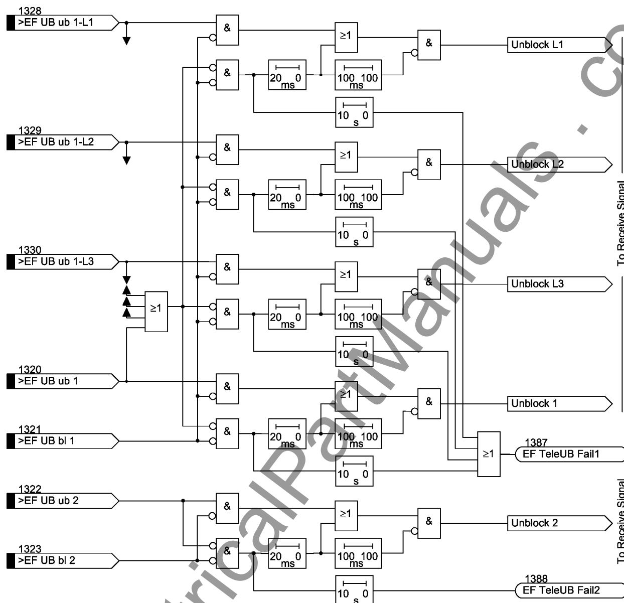
Figure 2-85 Unblock logic
