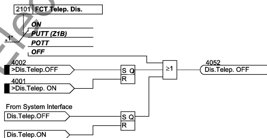
Figure 2-43 Activation and deactivation of the signal transmission logic
