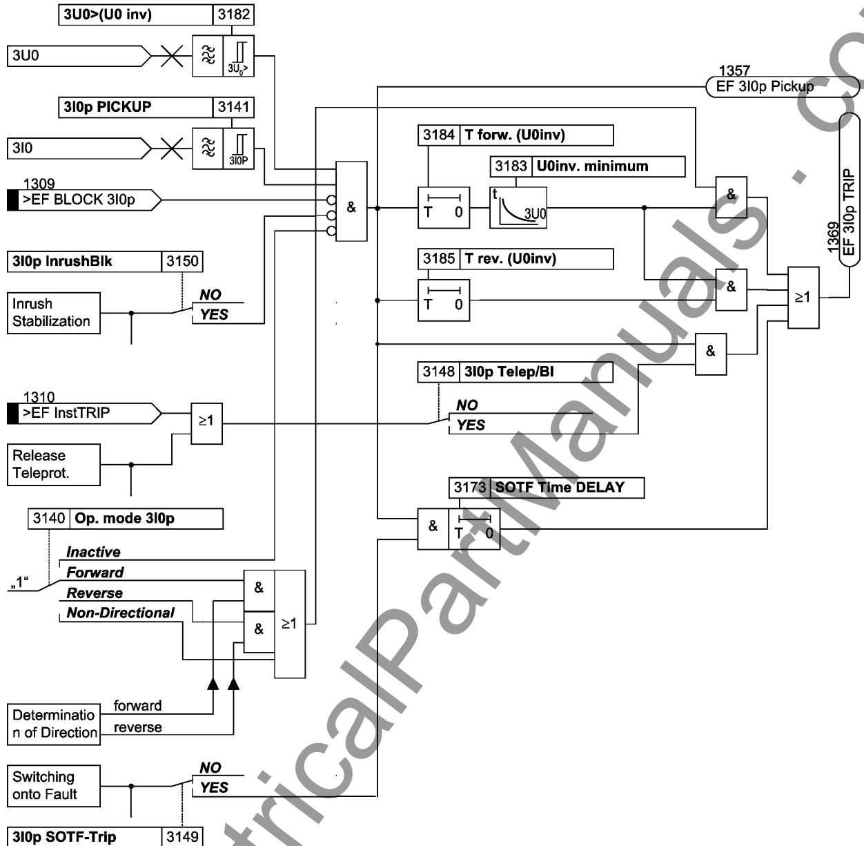
Figure 2-70 Directional zero-sequence voltage time protection with non-directional backup stage
