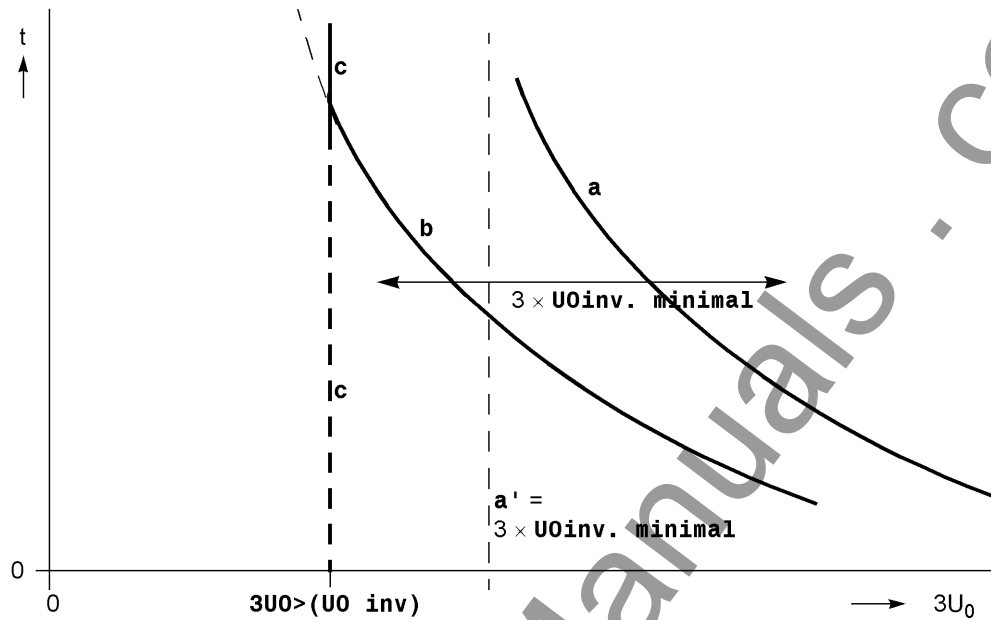
Figure 2-77 Characteristic settings of the zero-sequence voltage time dependent stage — without additional times
