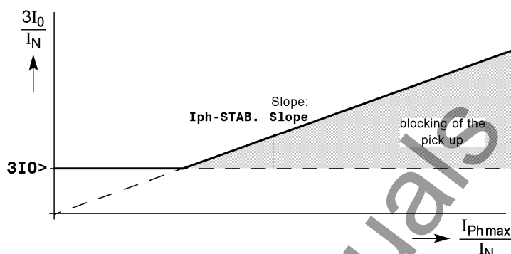
Figure 2-72 Phase current stabilization
