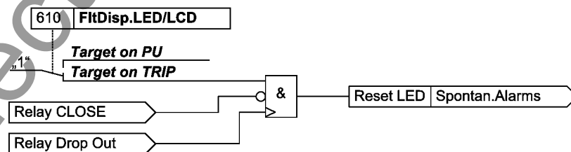
Figure 2-167 Logic diagram of the no-trip-no-flag feature (command-dependent alarms)
