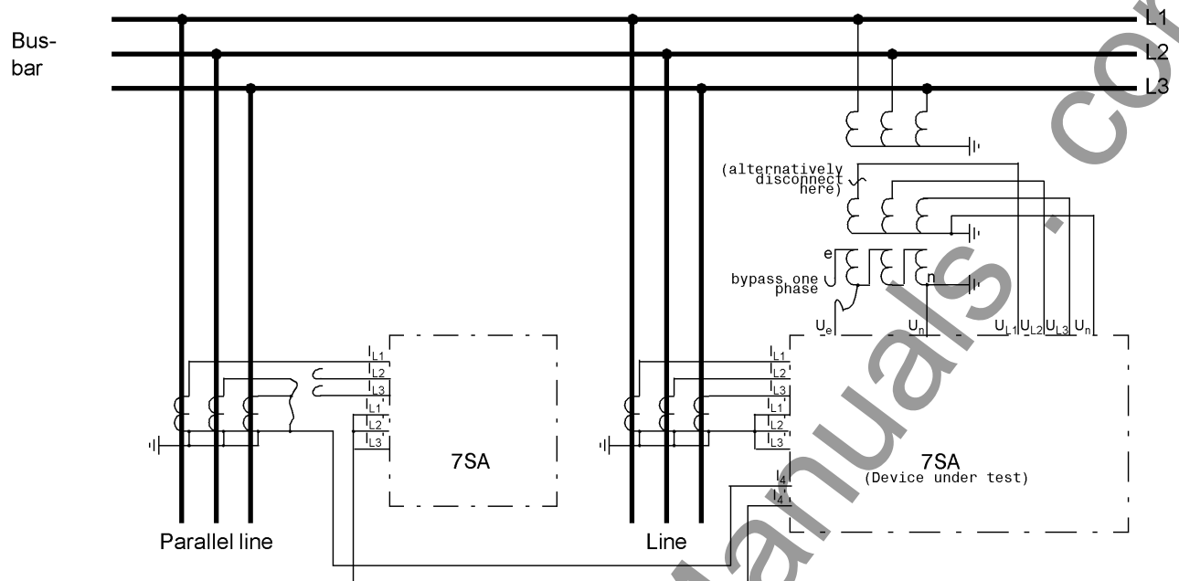
Figure 3-37 Polarity check for the current input I_4 , example for earth current of a parallel line
