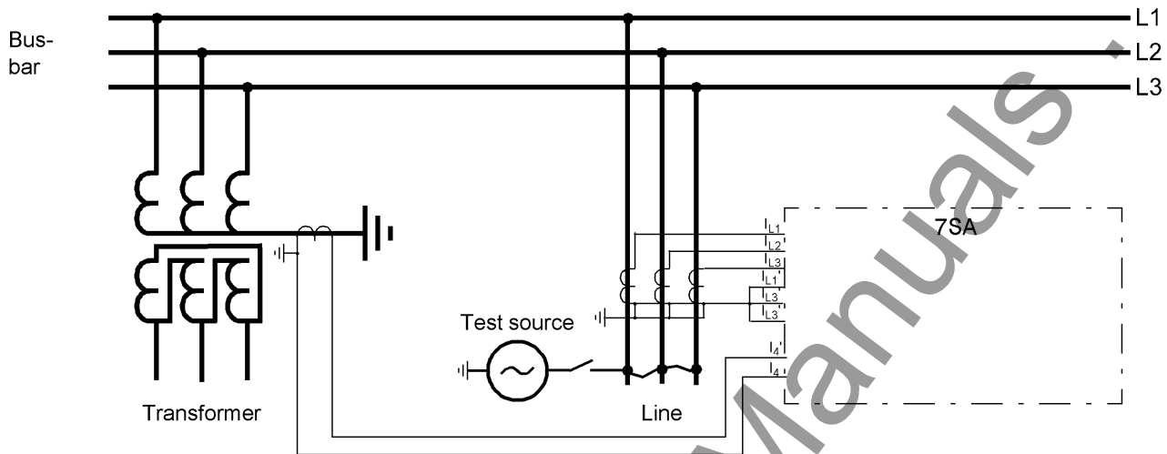
Figure 3-38 Polarity check of I_4 , example with earth current from a power transformer star-point
