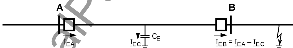
Figure 2-90 Possible current distribution during external earth fault
