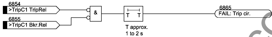
Figure 2-154 Logic diagram of the trip circuit monitoring with two binary inputs
