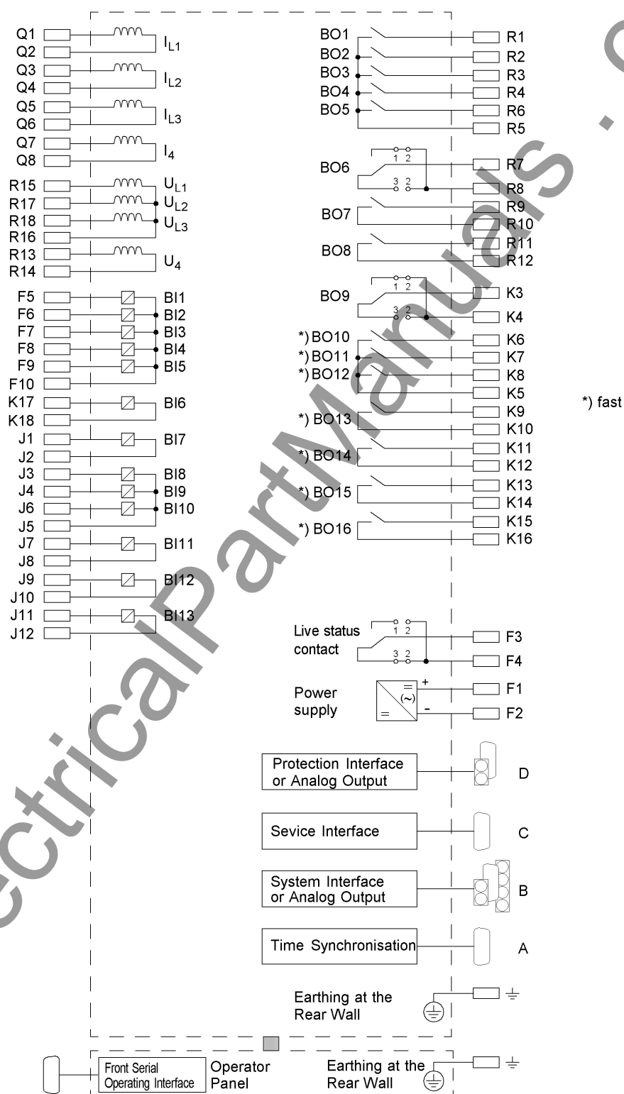
Figure A-23 General diagram 7SA641*-*A/J (panel surface mounting with detached operator panel)
