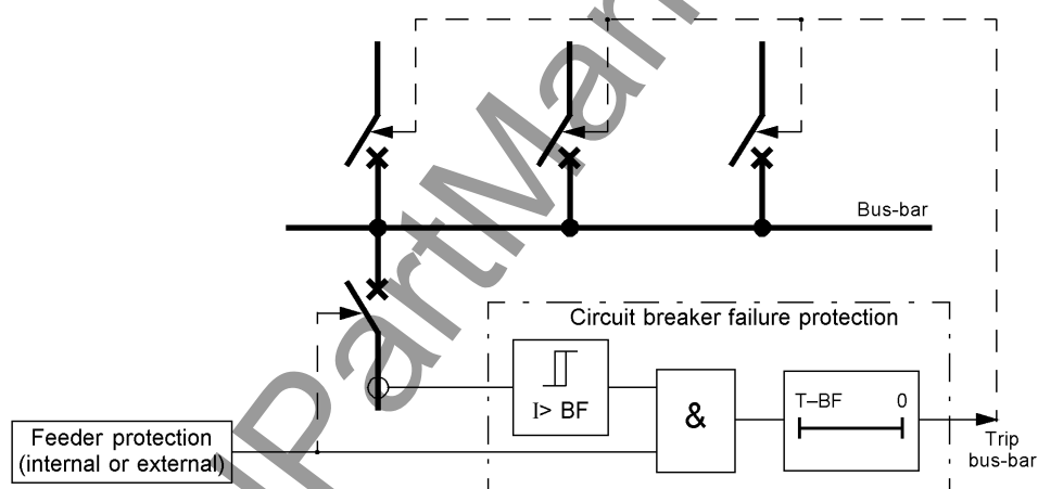
Figure 2-129 Simplified function diagram of circuit breaker failure protection with current flow monitoring
