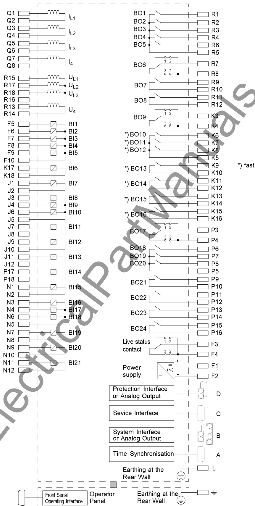
Figure A-26 General diagram 7SA642*-*A/J (panel surface mounting with detached operator panel)
