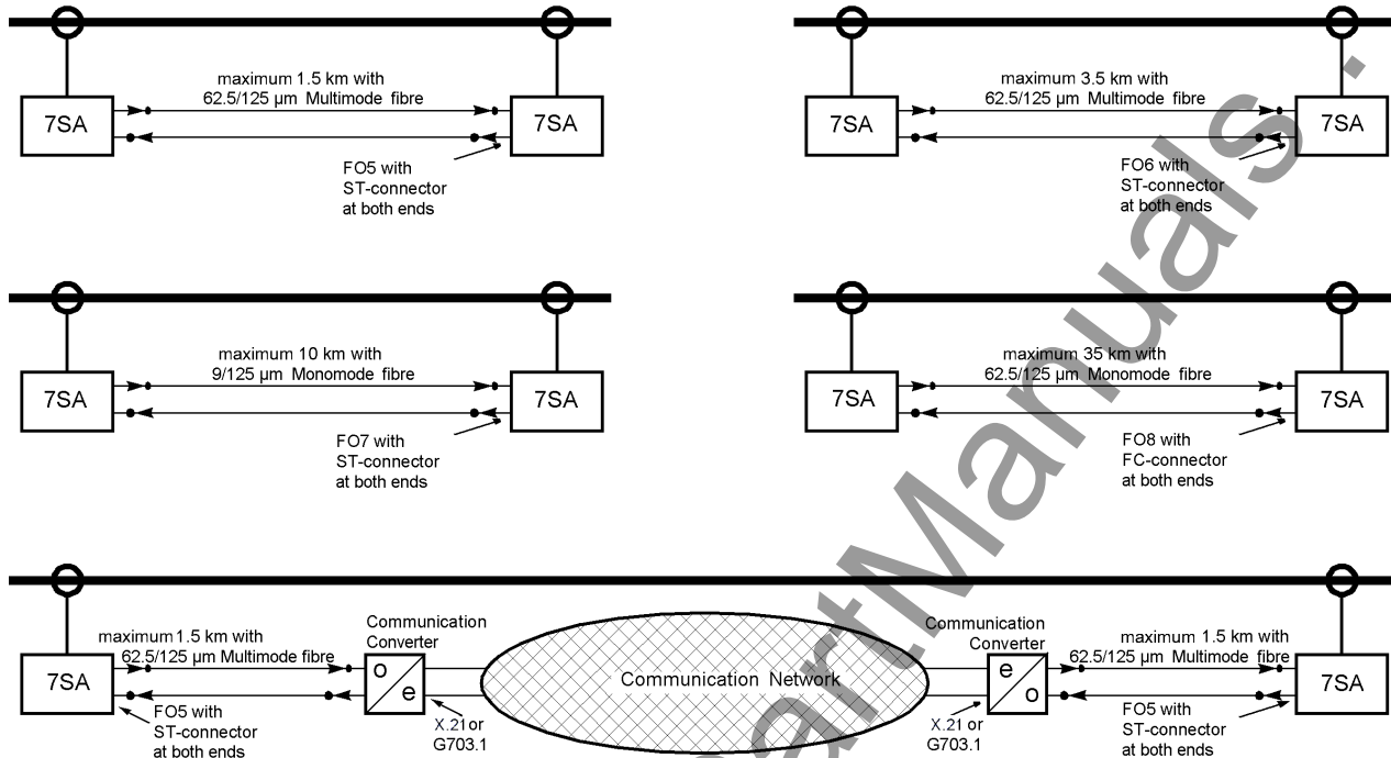
Figure 2-40 Examples for communication connections
