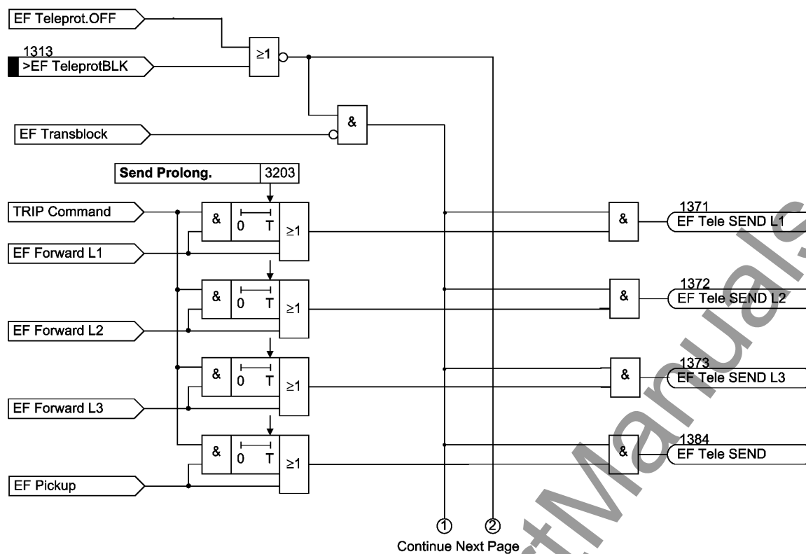
Figure 2-81 Logic diagram of the directional comparison scheme with protection data interface (for one device)
