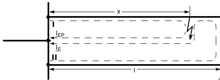
Figure 2-4 Reach with parallel line compensation at II
