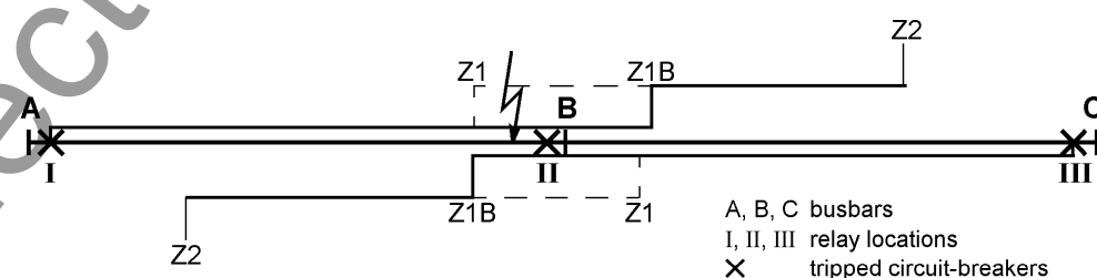
Figure 2-109 Example of a reduced dead time (RDT)
