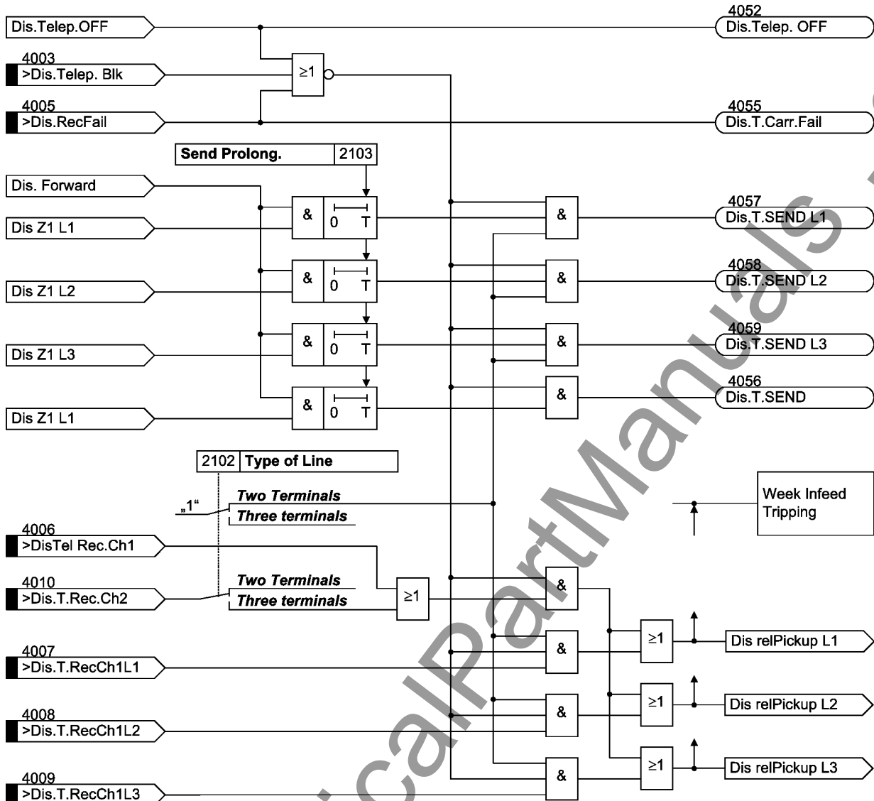
Figure 2-45 Logic diagram of the permissive underreach transfer trip (PUTT) with pickup (one line end)
