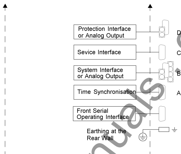
Figure A-9 General diagram for 7SA6*2**N/S (panel flush mounting or cubicle mounting)
