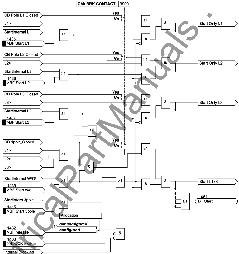
Figure 2-137 Initiation conditions with single-pole trip command
