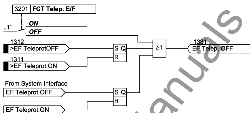
Figure 2-78 Activation and deactivation of the signal transmission logic
