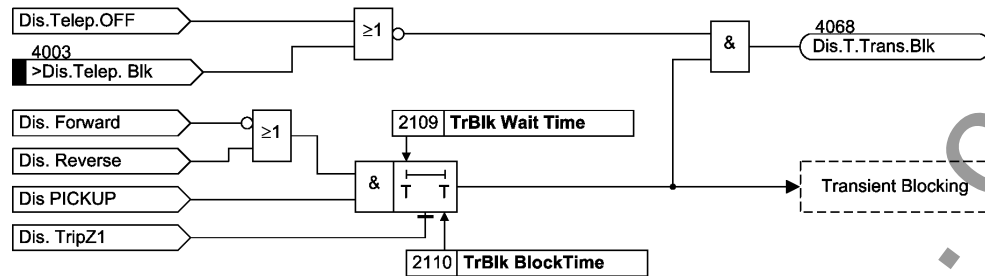
Figure 2-64 Transient blocking for permissive schemes
