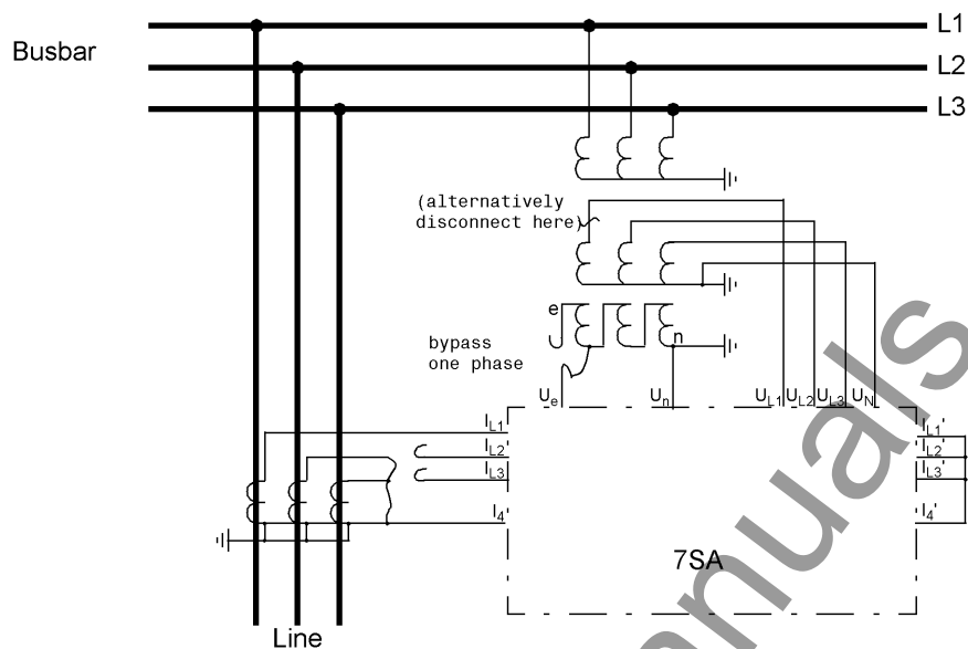
Figure 3-36 Polarity check for the current input I_4 , example for current transformer set in Holmgreen circuit
