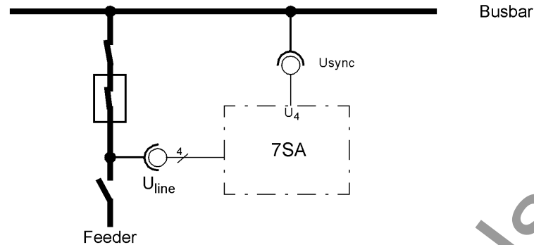
Figure 3-35 Measuring voltages for the synchronism check
