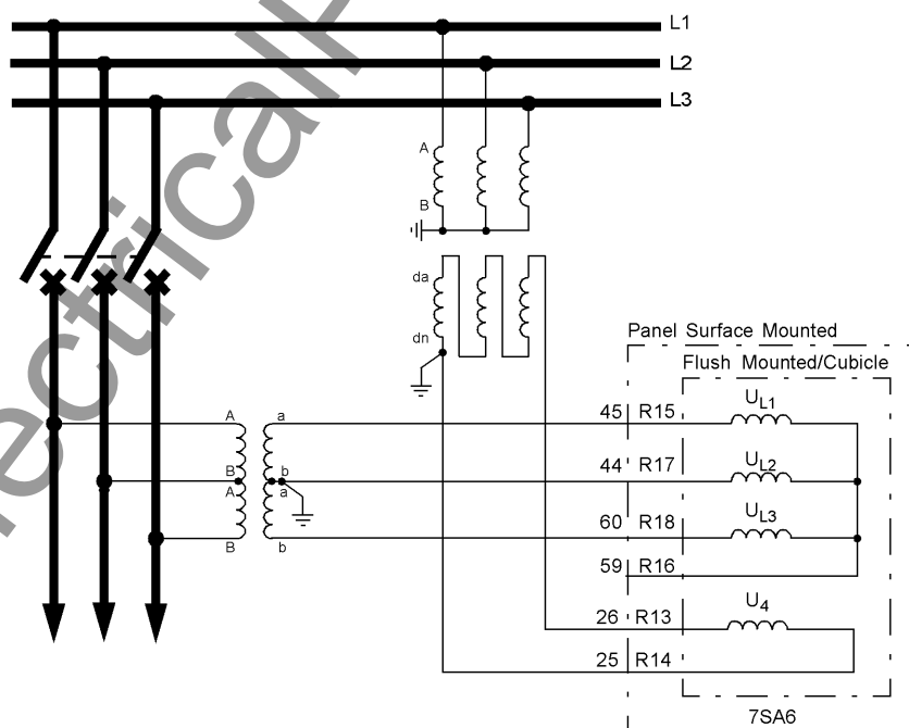
Figure A-44 Voltage connections to two V-connected voltage transformers with additional open-delta windings (da-dn-winding) from the busbar — not permitted for earthed networks
