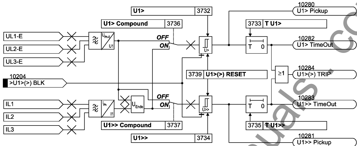
Figure 2-121 Logic diagram of the overvoltage protection for the positive sequence voltage system
