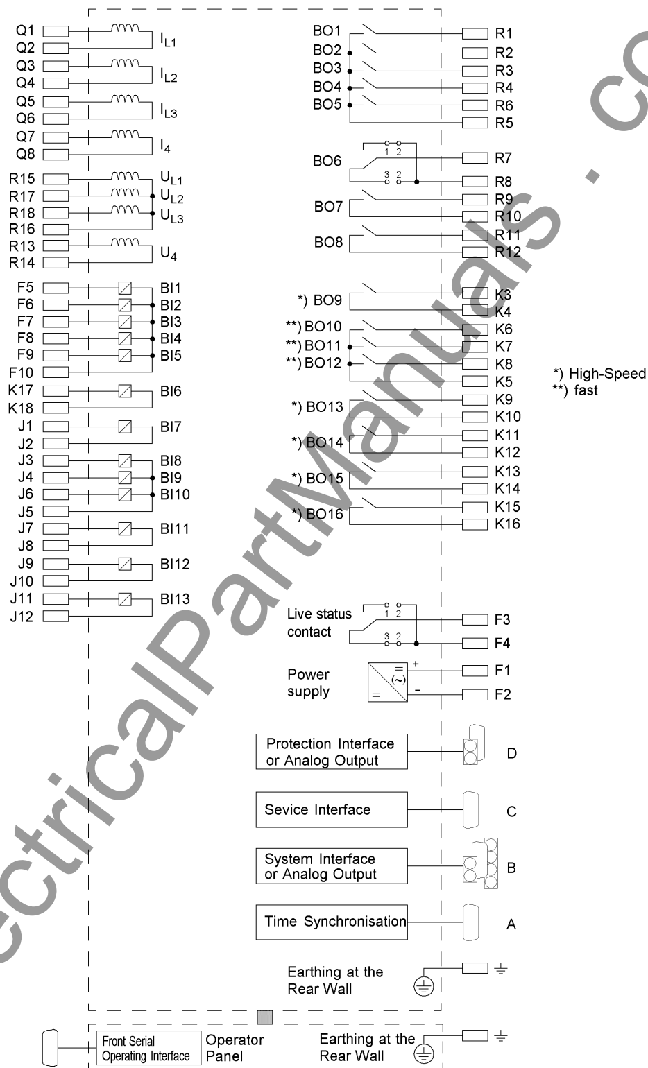
Figure A-25 General diagram 7SA641*-*M/P (panel surface mounting with detached operator panel)
