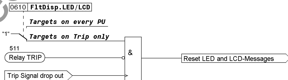
Figure 2-1 Creation of the reset command for the latched LED and LCD messages
