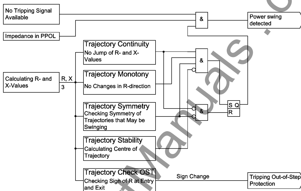
Figure 2-37 Logic diagram of power swing detection
