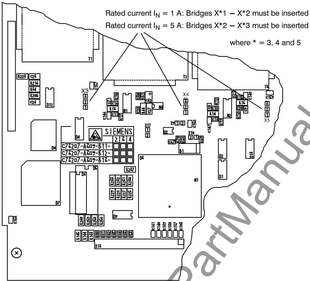
Figure 5.2 Checking for the rated current 1 A/5 A
