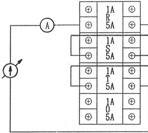
Figure 15 Test Circuit (1)
