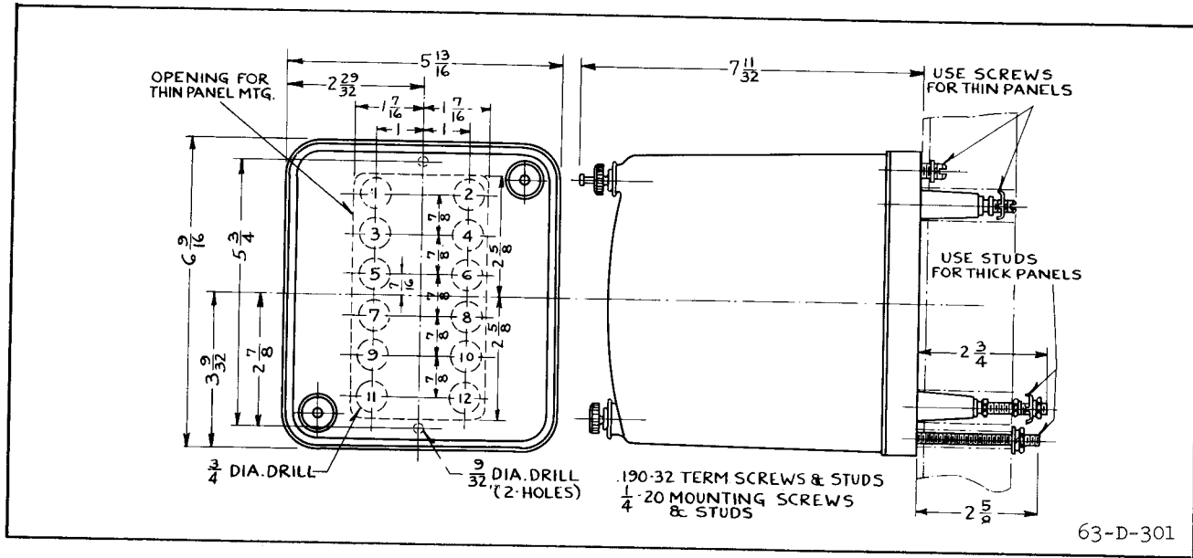
Fig. 5—Outline and Drilling Plan for the Standard Projection Case. See the Internal Schematic for the Terminals Supplied. For Reference Only.
