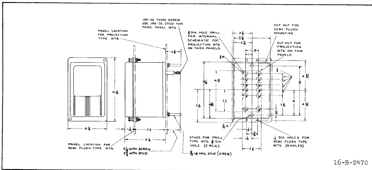
Fig. 6—Outline and Drilling Plan for the S10 Projection or Semi-flush Type FT Flexitest Case. See the Internal Schematic for the Terminals Supplied. For Reference Only.
