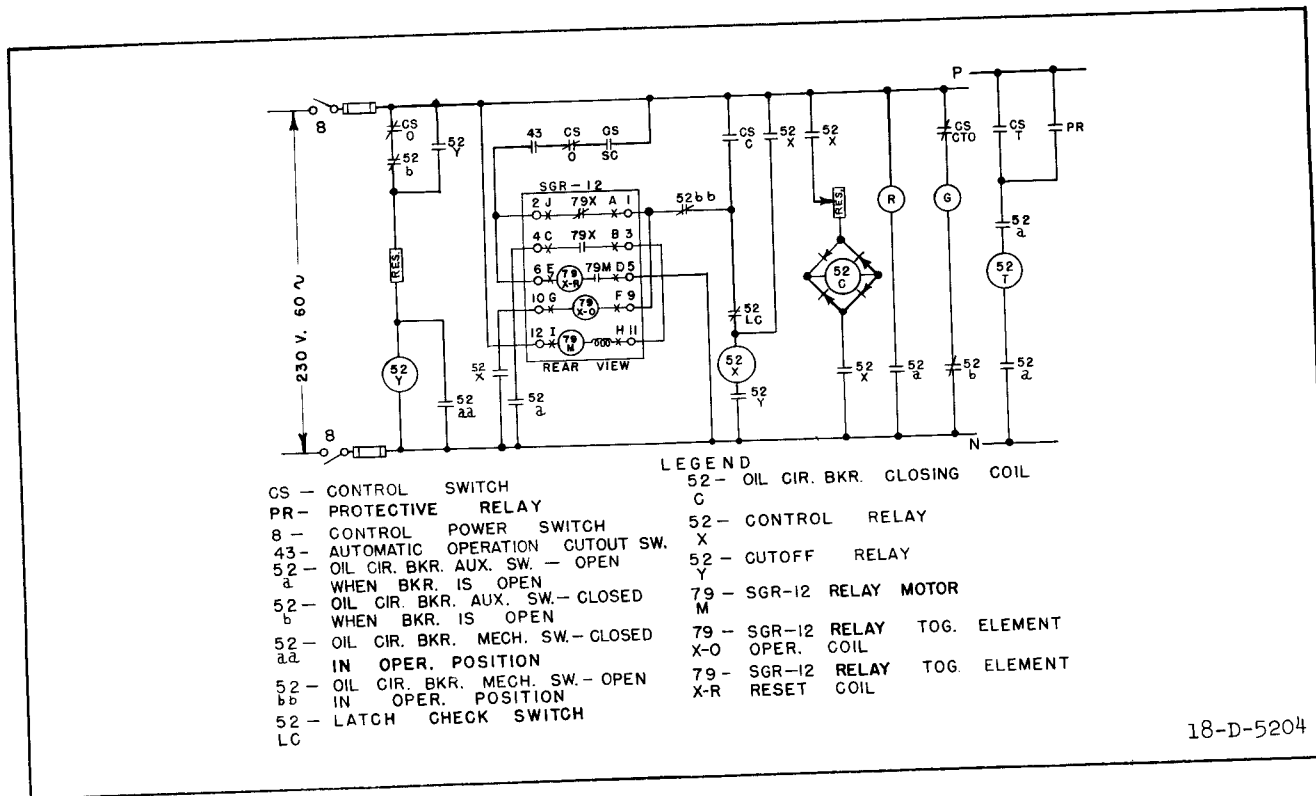
Fig. 4—Typical External Connections of the Type SGR-12 Reclosing Relay in the Type FT Case for Instantaneous Reclosure of a Breaker With a.c. Control.
