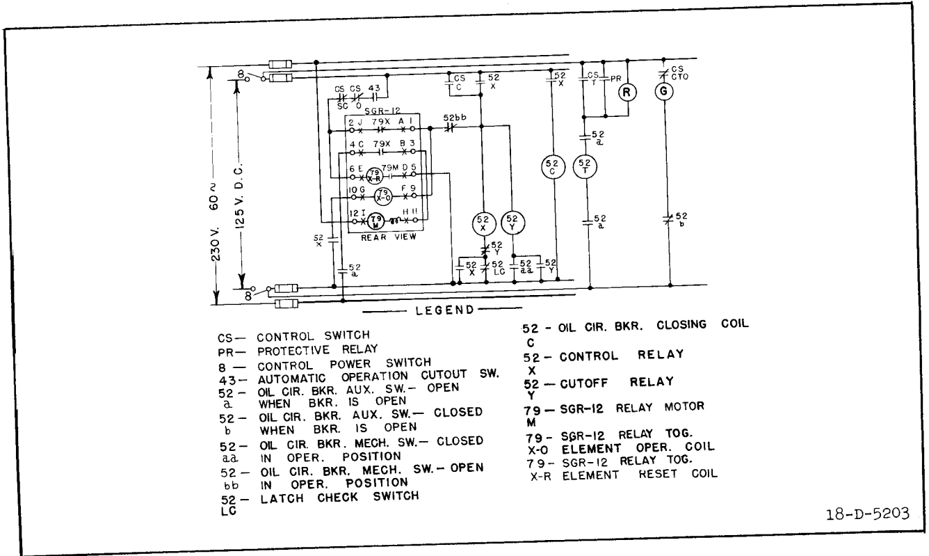
Fig. 3—Typical External Connections of the Type SGR-12 Reclosing Relay in the Type FT Case For Instantaneous Reclosure of a Breaker With d.c. Control.
