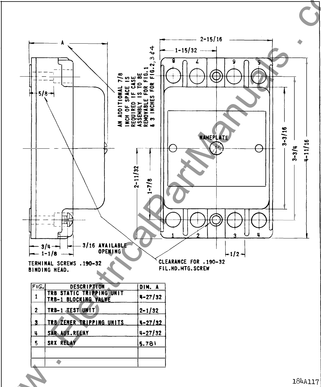
Fig. 11. Outline and drilling plan for the type SAR, SAR-1 and SAR-2 relays.
