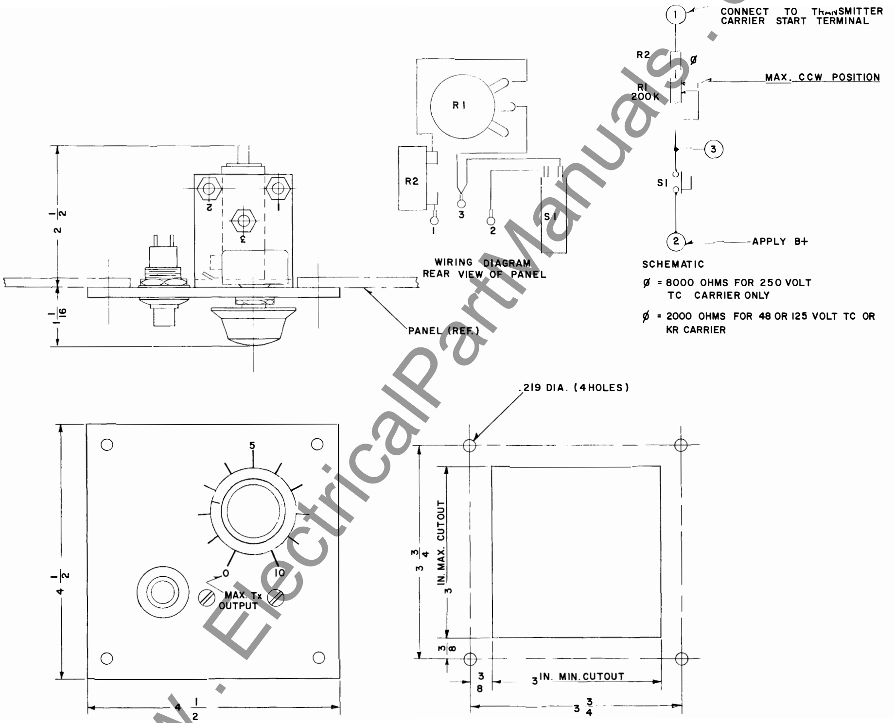
Fig. 11. Reserve Signal Detector Outline (Dwg. 329C703)
