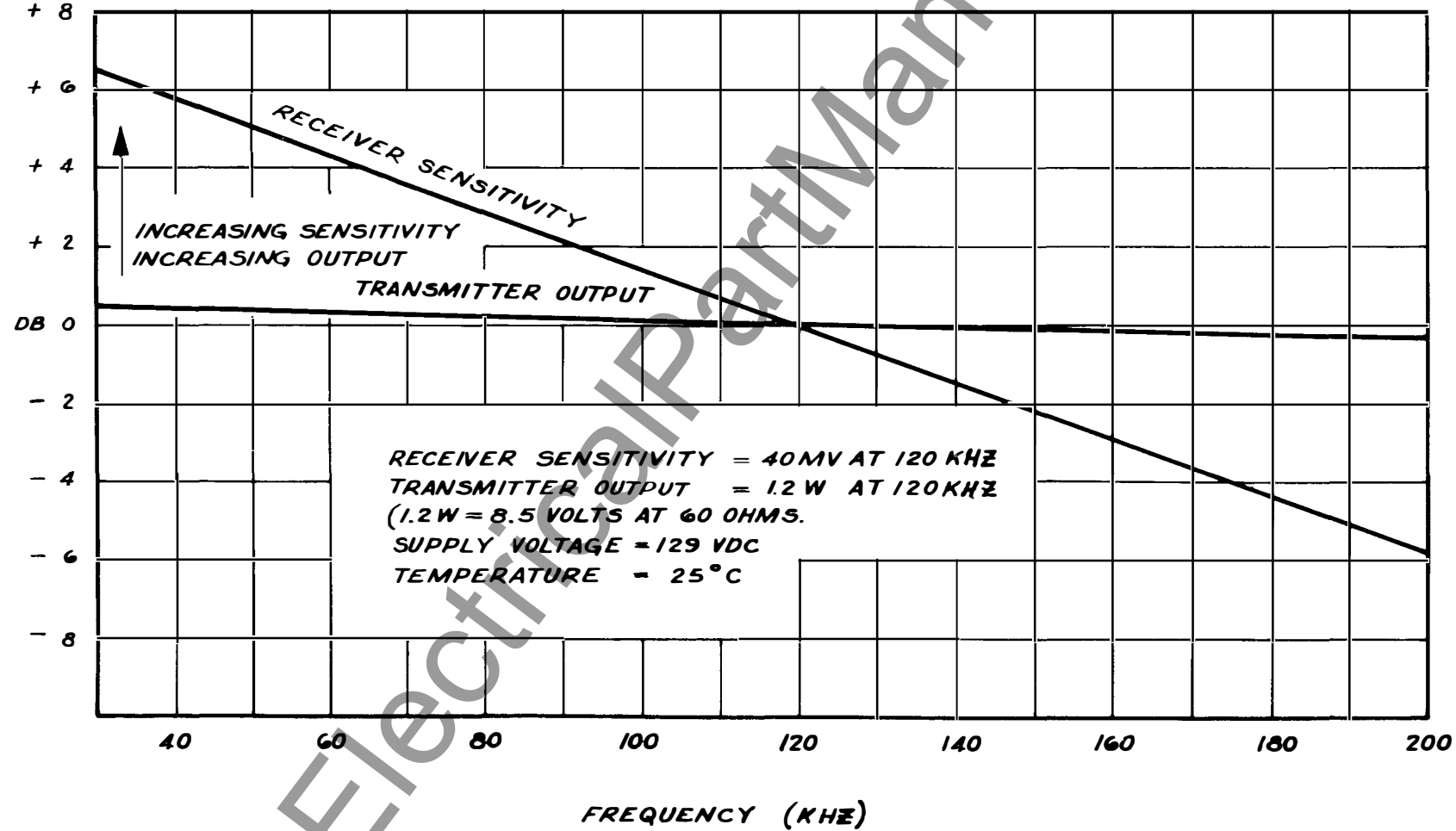
* Fig. 13. Transmitter Output and Receiver Sensitivity Variations with Frequency (Curve# 378000)
