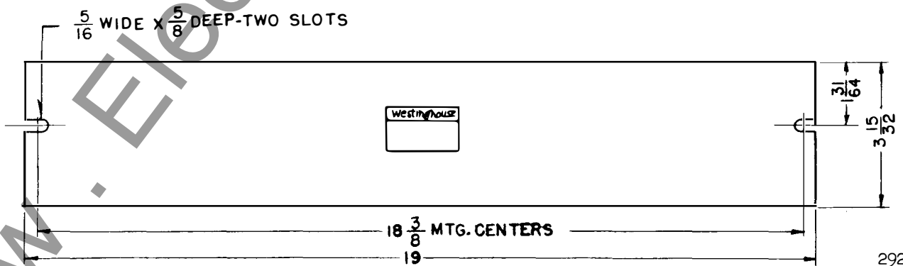
Fig. 7. Supervisory Control Auxiliary Relay Connections (Dwg. 629A552) and Outline (Dwg. 292B991).
