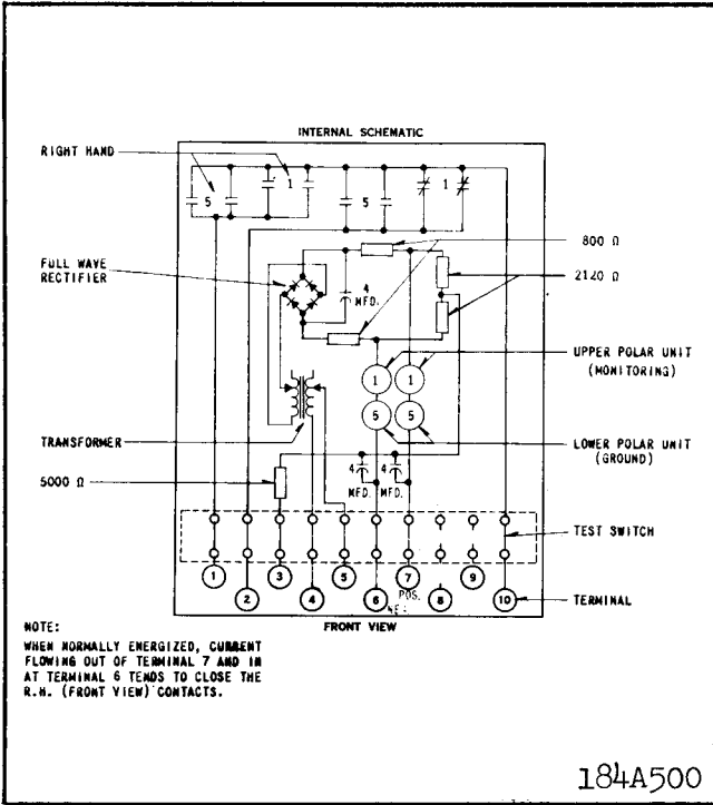
Fig. 2. Internal schematic of the type PMA relay in FT 31 case - 120 volt, 60 hertz supply - For two terminal lines.
