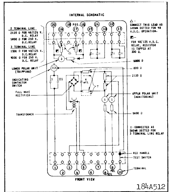
Fig. 17. Internal schematic of the type PM-13 relay in the FT 32 case - 120 volt, 60 hertz supply - For two or three terminal lines.
