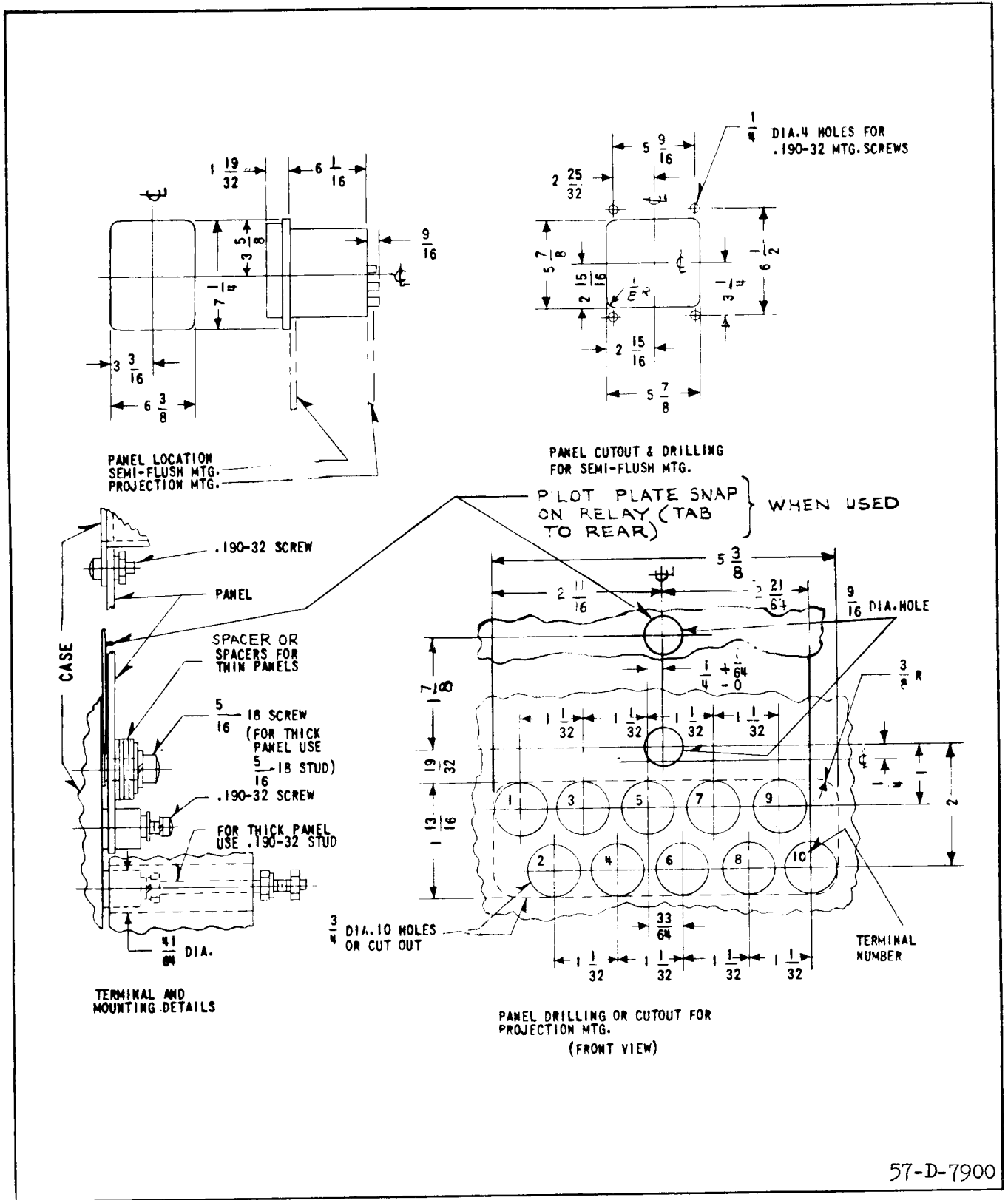
Fig. 36. Outline and Drilling Plan for the type PM-3, PM-5, & PMD-1 Relays in the type FT 11 case.
