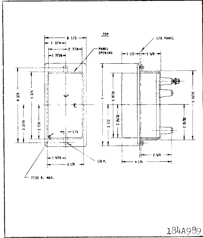
Fig. 35. Outline and Drilling Plan for the type PM-4 Auxiliary unit in the Semi-Flush molded case.
