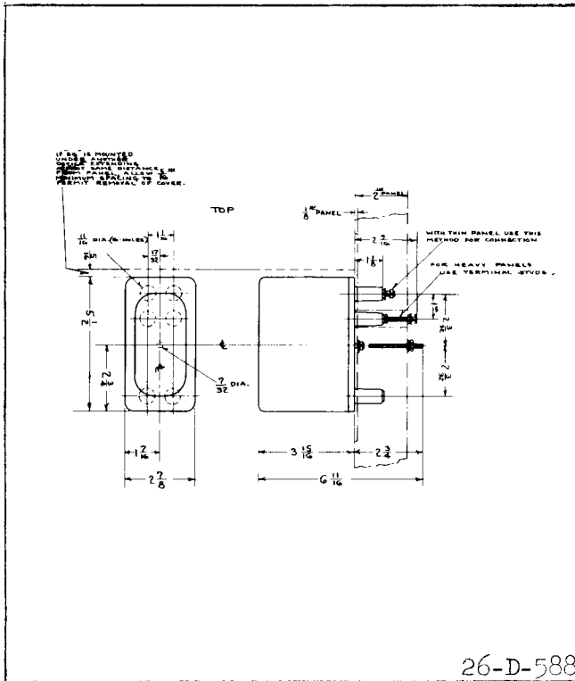
Fig. 34. Outline and Drilling Plan for the type PM-4 Auxiliary unit in the projection molded case.
