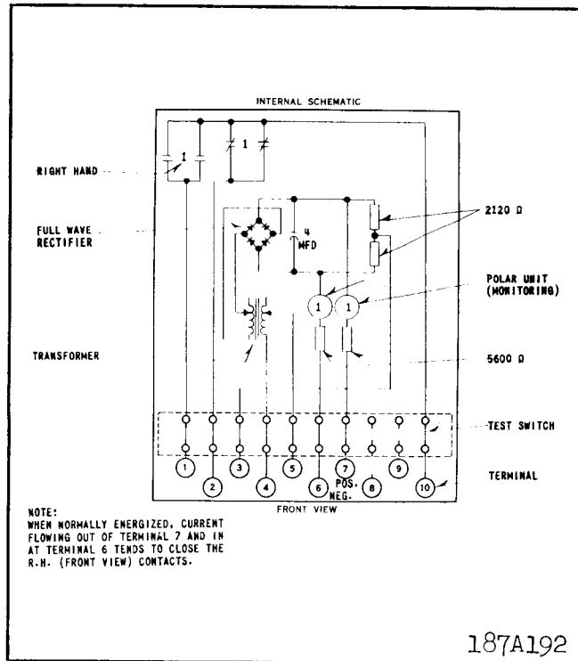
Fig. 5. Internal schematic of type PMA-1 relay in FT 21 case - 120 volt, 60 hertz supply - For three terminal lines.
