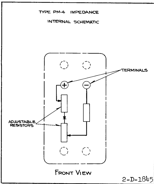
Fig. 12. Internal schematic of the type PM-4 Auxiliary Unit in the small molded case.
