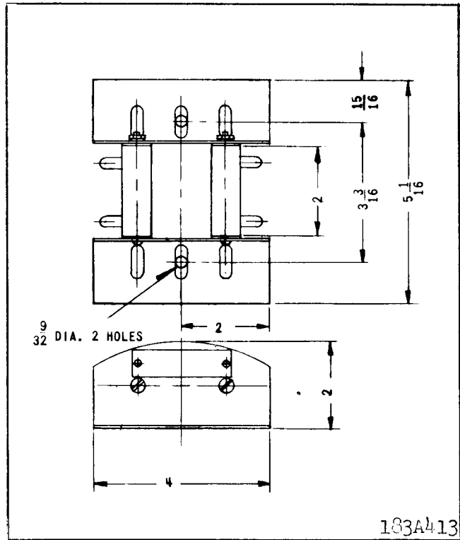
Fig. 33. Outline and Drilling Plan for External Remote trip Resistor Assembly.
