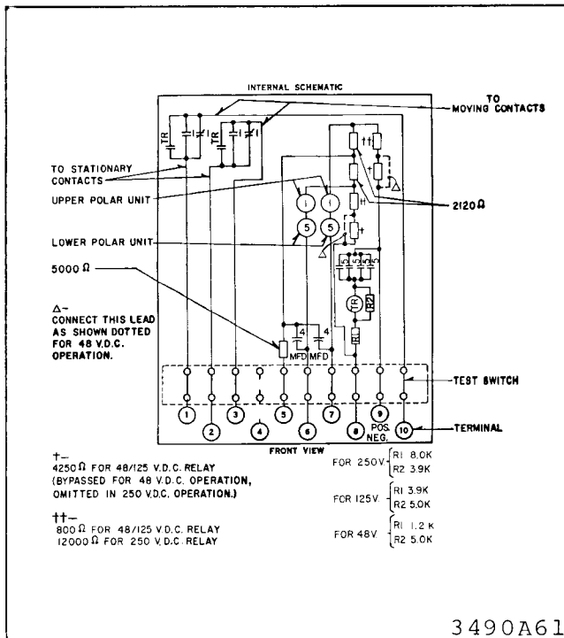
Fig. 23. PMD Relay - Ground Alarm, D.P.D.T. Contacts, Two Terminal Lines with Telephone Relay Output - FT-21 Case.
