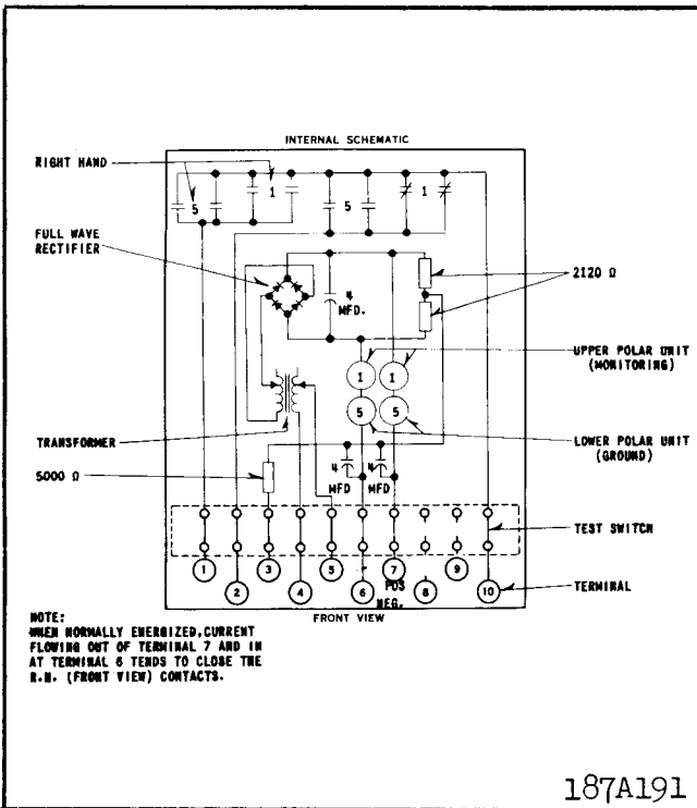
Fig. 4. Internal schematic of type PMA relay in FT 31 case - 120 volt, 60 hertz supply - For three terminal lines.
