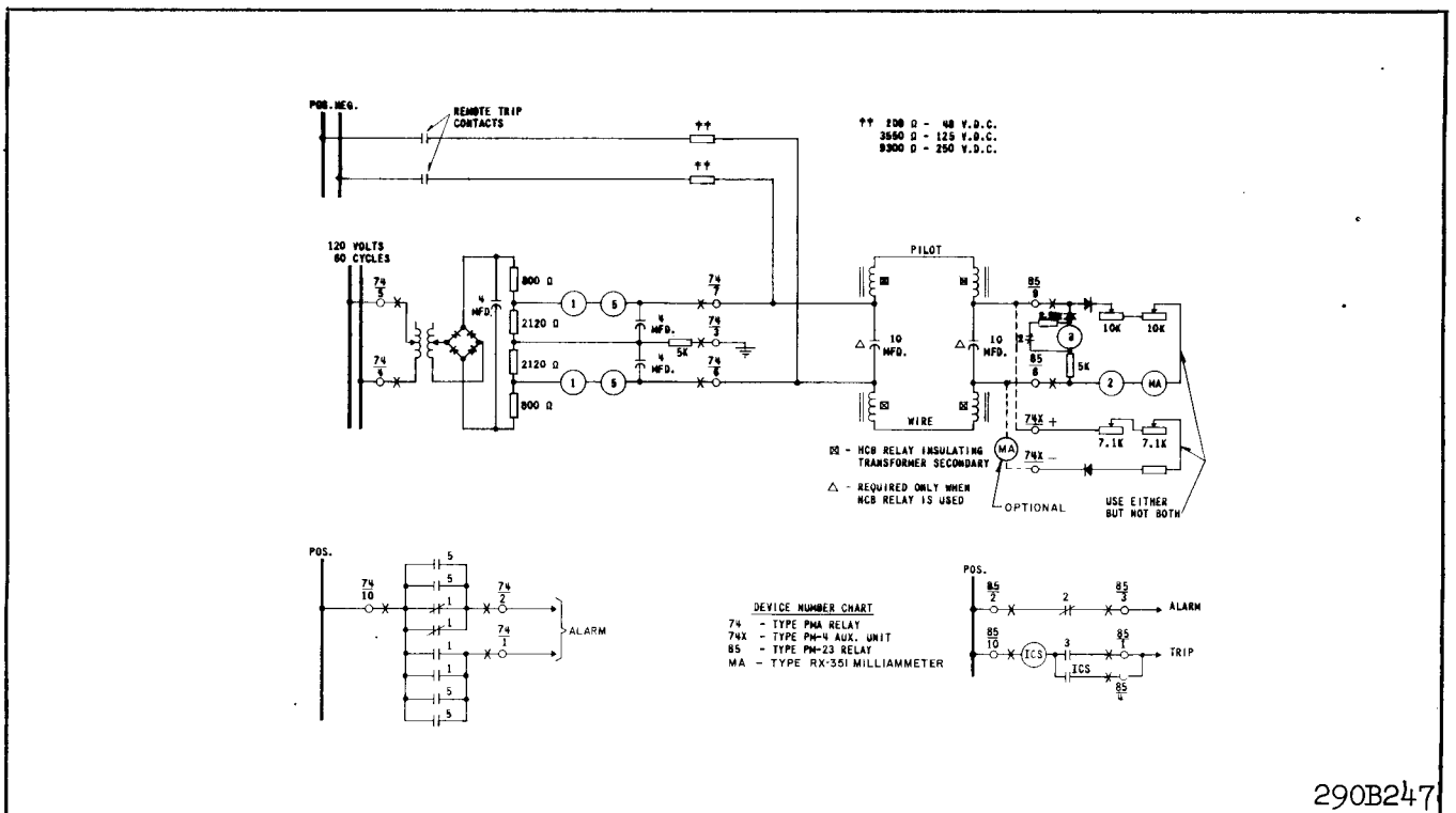
Fig. 22. External schematic of the type PMA relay with type PM-23 or PM-4 relay - Two terminal lines.
