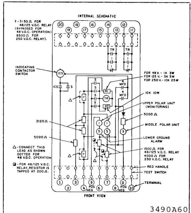
Fig. 22. PMG-13 Relay with Ground Alarm and Remote Trip - Three Terminal Lines with Telephone Relay Output - FT-32 Case.
