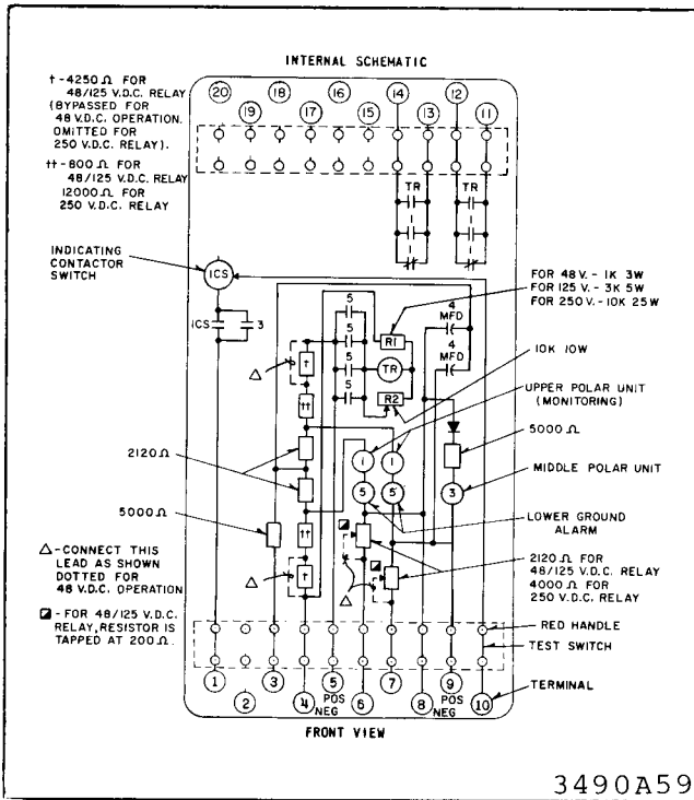
* Fig. 21. PMG-13 Relay with Ground Alarm and Remote Trip - Two Terminal Lines with Telephone Relay Output. FT-32 Case.
