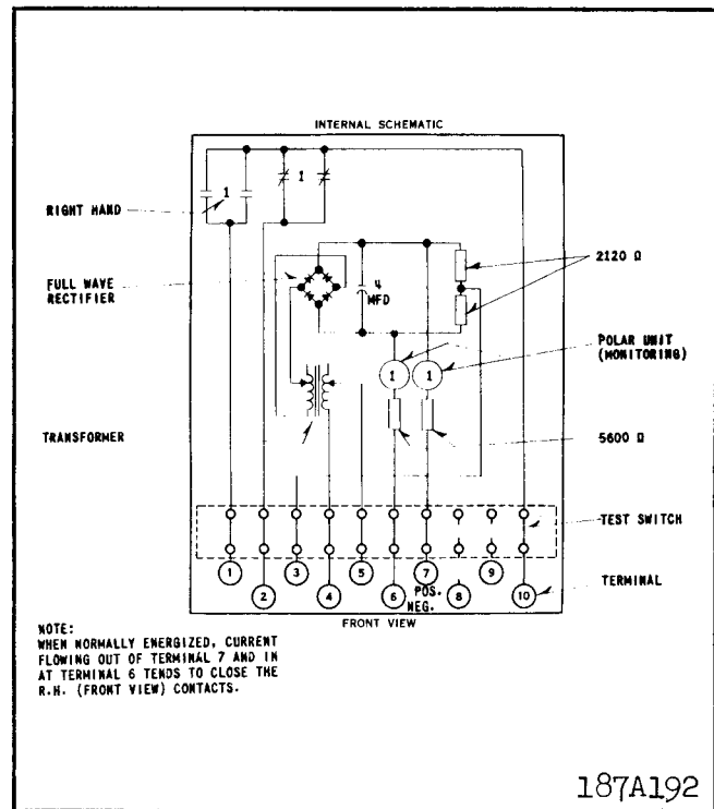
Fig. 5. Internal schematic of type PMA-1 relay in FT 21 case - 120 volt, 60 hertz supply - For three terminal lines.
