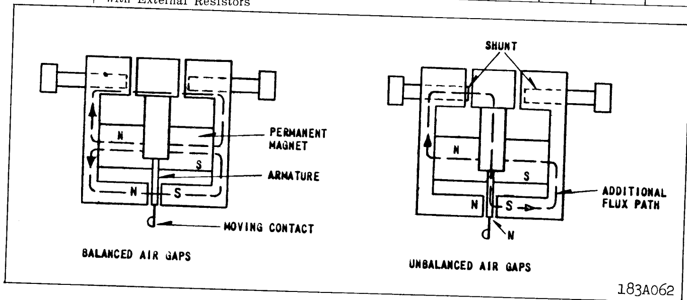
Fig. 1. Polar Unit Permanent Magnet Flux Paths.
