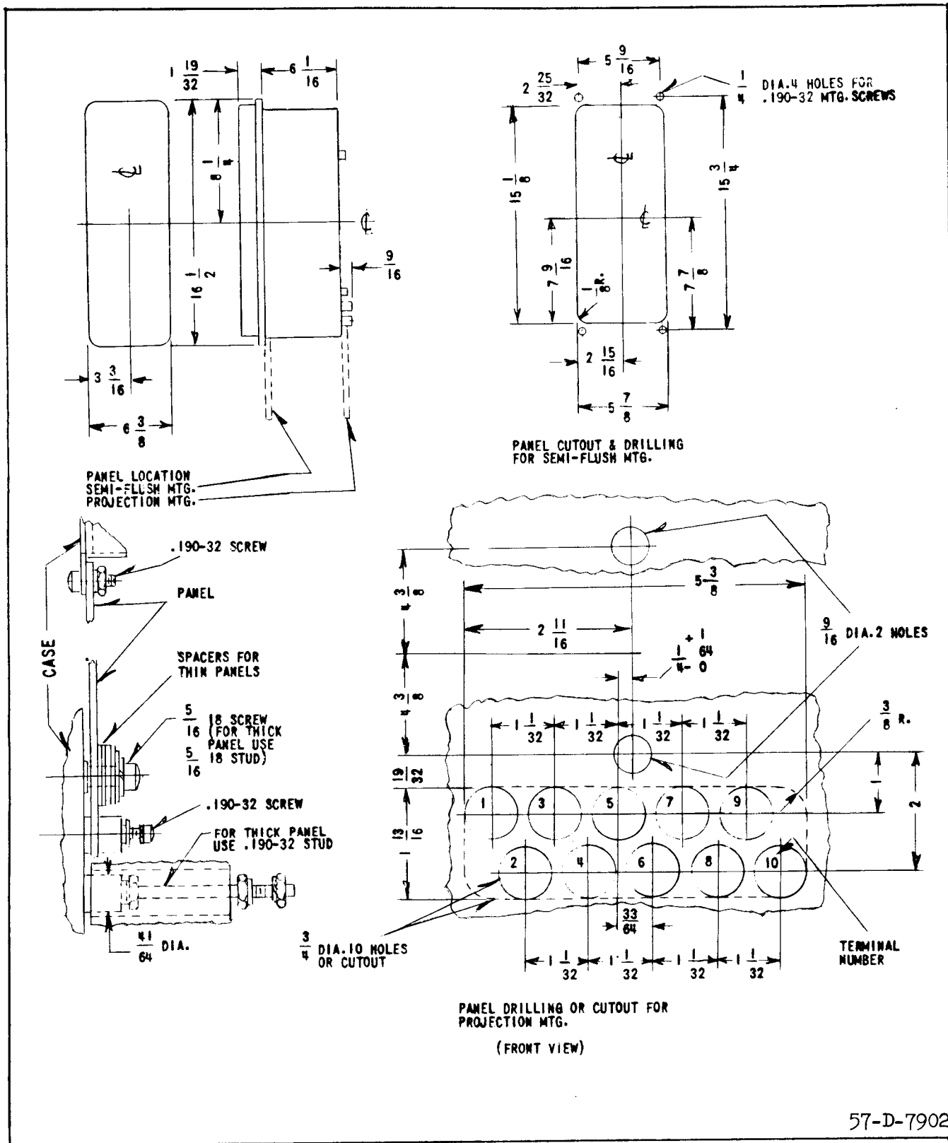
Fig. 38. Outline and Drilling Plan for the type PMA relay in the type FT 31 case.
