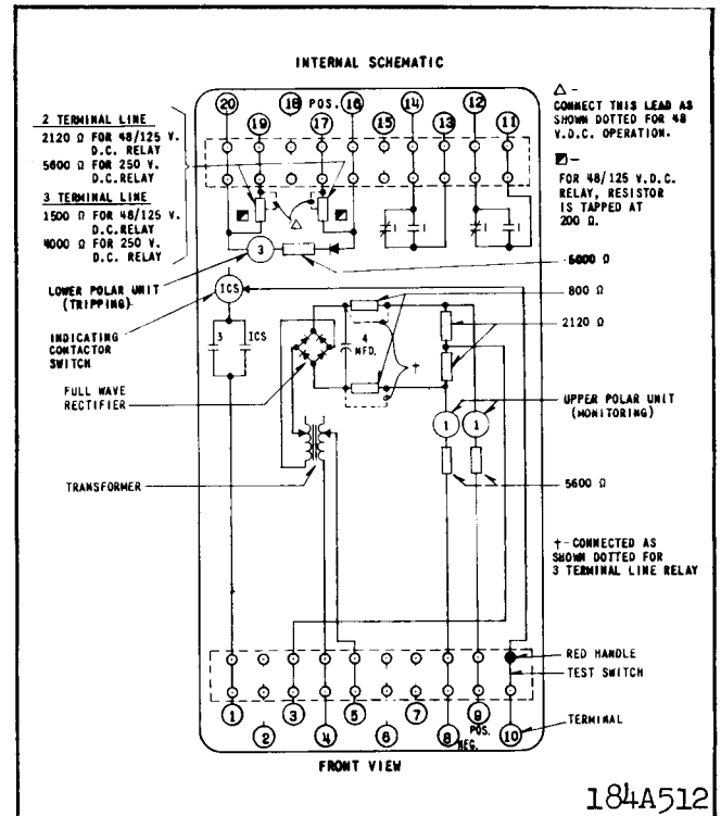
Fig. 17. Internal schematic of the type PM-13 relay in the FT 32 case - 120 volt, 60 cycle supply - For two or three terminal lines.
