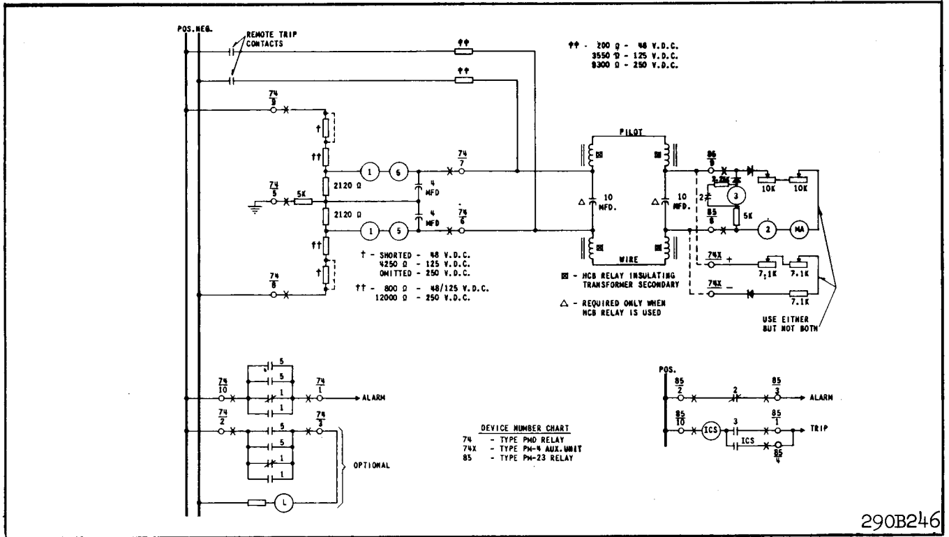
Fig. 21. External schematic of the type PMD relay with type PM-23 or PM-4 relay – Two terminal lines.
