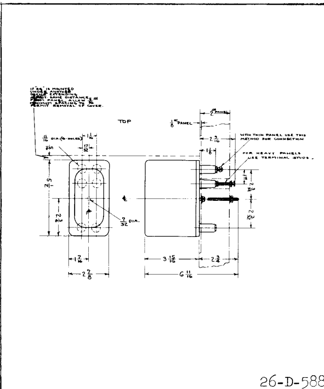
Fig. 30. Outline and Drilling Plan for the type PM-4 Auxiliary unit in the projection molded case.
