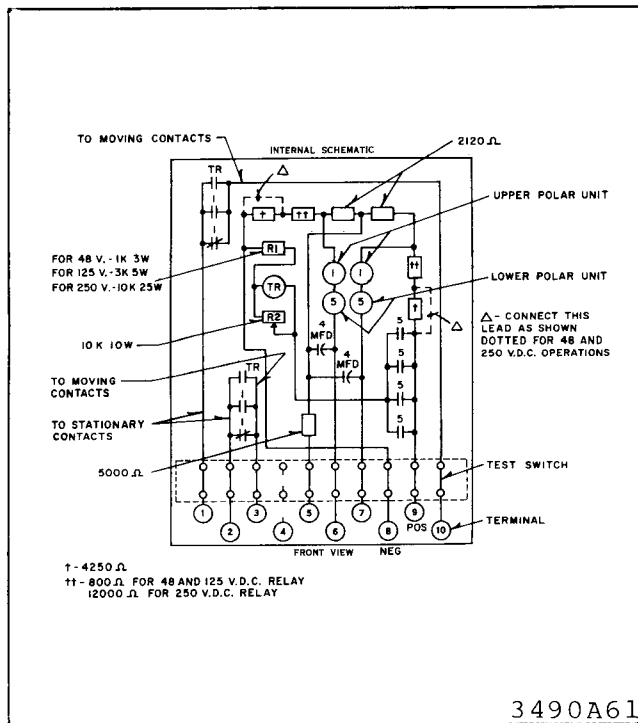
Fig. 23. PMD Relay - Ground Alarm, D.P.D.T. Contacts, Two Terminal Lines with Telephone Relay Output - FT-21 Case.
