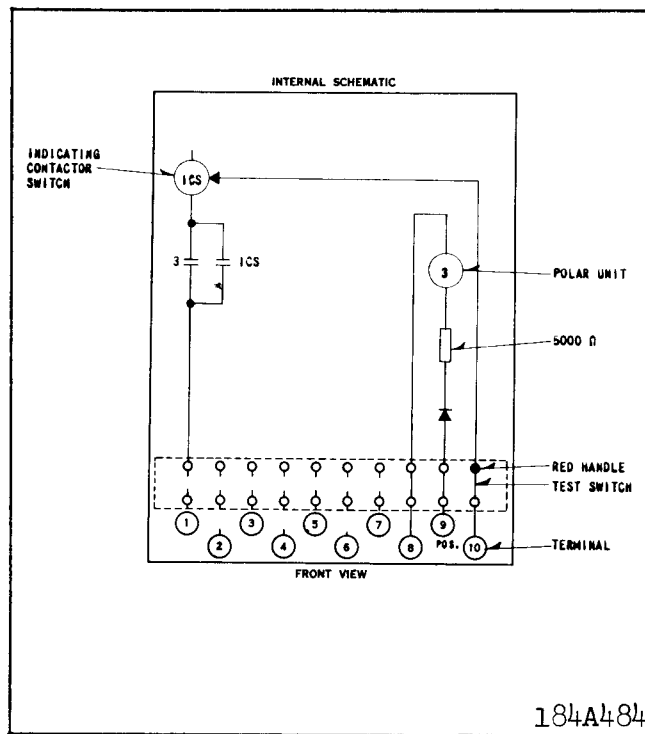
Fig. 11. Internal schematic of the type PM-3 relay in the FT 11 case.
