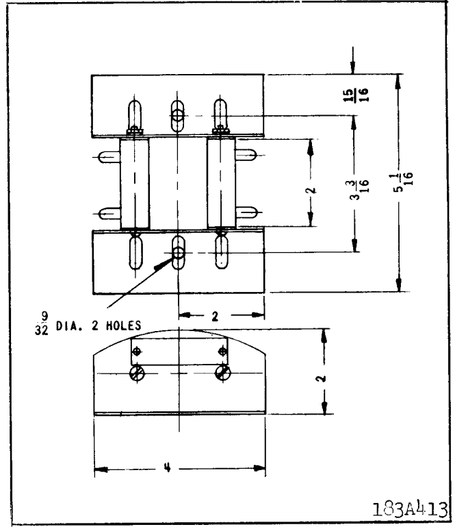
Fig. 29. Outline and Drilling Plan for External Remote trip Resistor Assembly.
