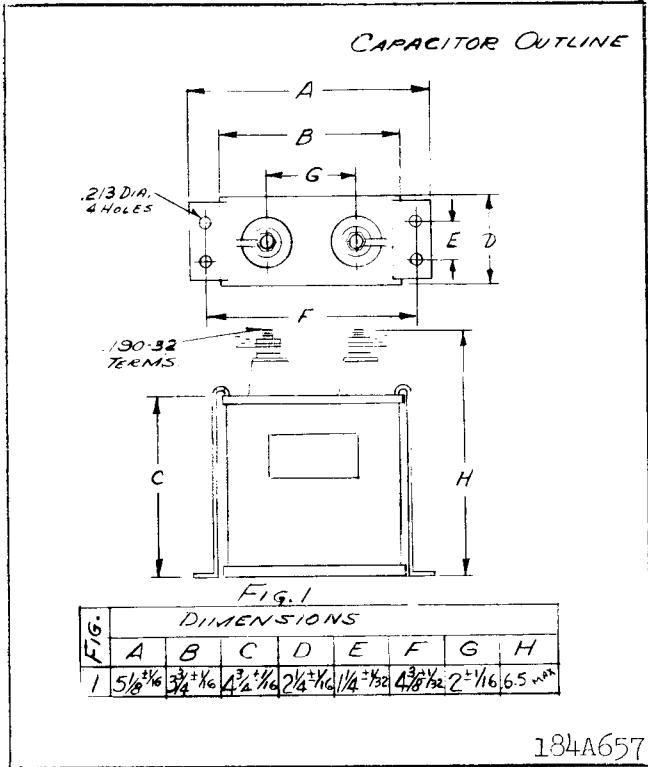
Fig. 32. Outline and Drilling Plan for 10 mfd. capacitor - For reference only.
