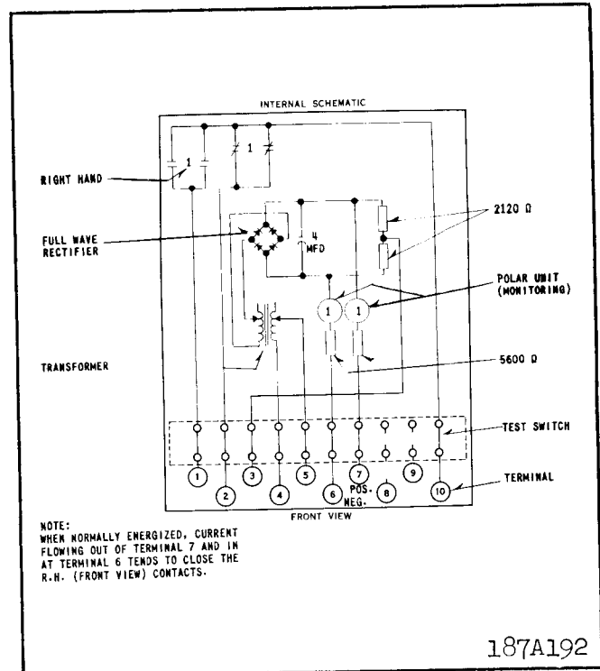
Fig. 5. Internal schematic of type PMA-1 relay in FT 21 case - 120 volt, 60 cycle supply - For three terminal lines.
