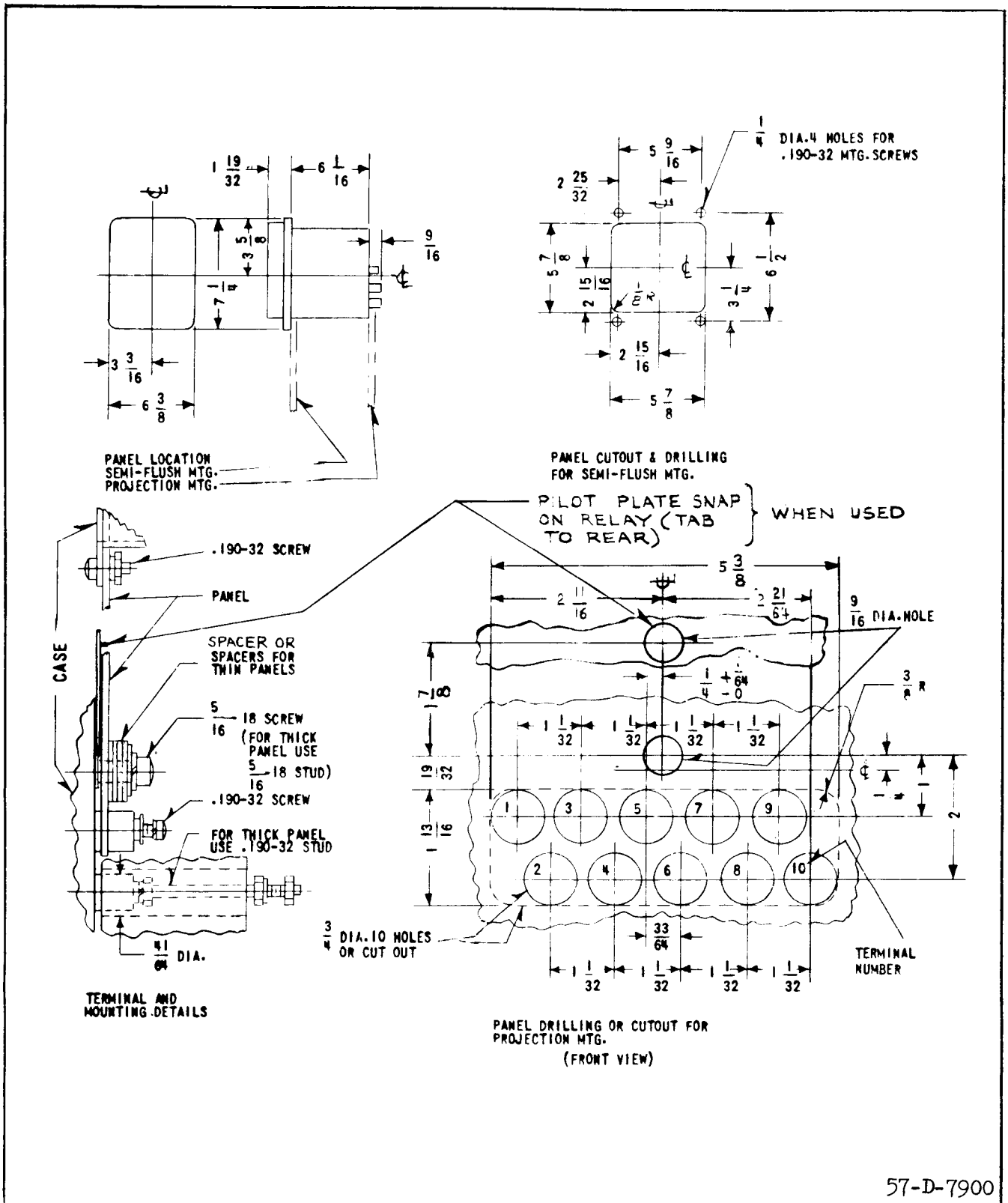
Fig. 36. Outline and Drilling Plan for the type PM-3, PM-5, & PMD-1 Relays in the type FT 11 case.
