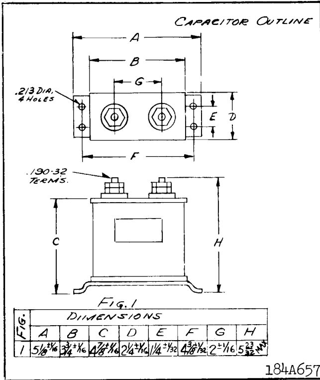
Fig. 28. Outline and Drilling Plan for 10 mfd. capacitor – For reference only.
