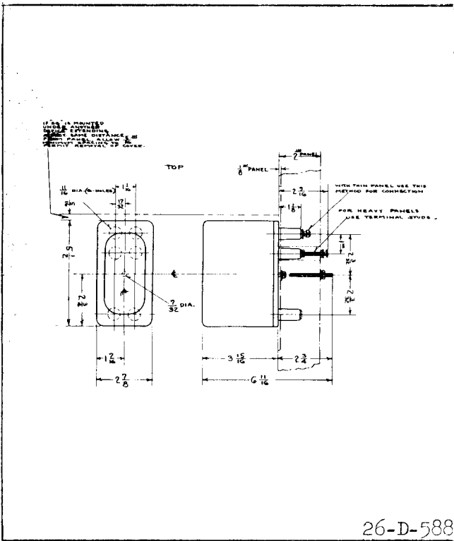
Fig. 34. Outline and Drilling Plan for the type PM-4 Auxiliary unit in the projection molded case.
