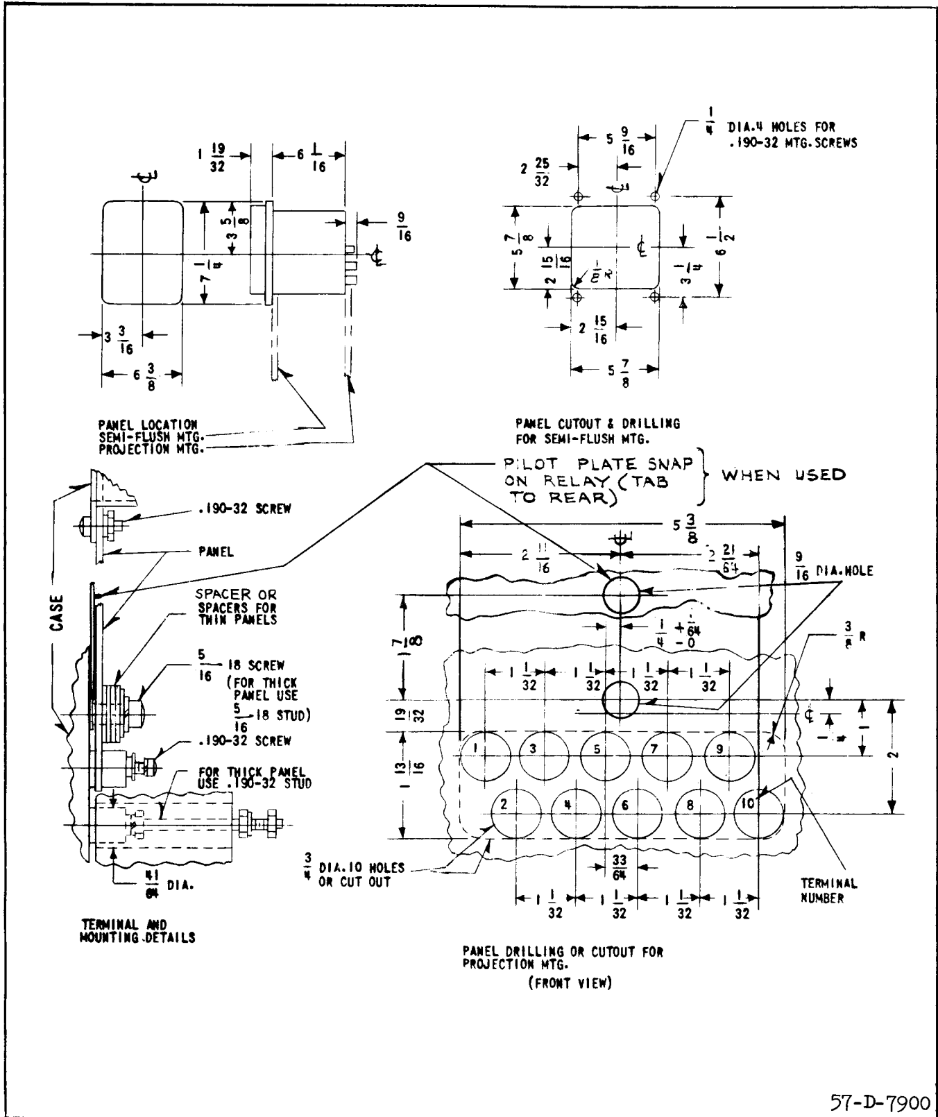
Fig. 32. Outline and Drilling Plan for the type PM-3, PM-5, & PMD-1 Relays in the type FT 11 case.
