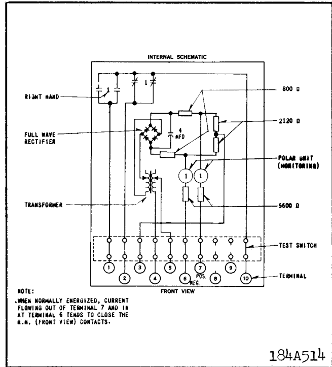
Fig. 3. Internal schematic of type PMA-1 relay in the FT 21 case - 120 volts, 60 hertz supply - For two terminal lines.
