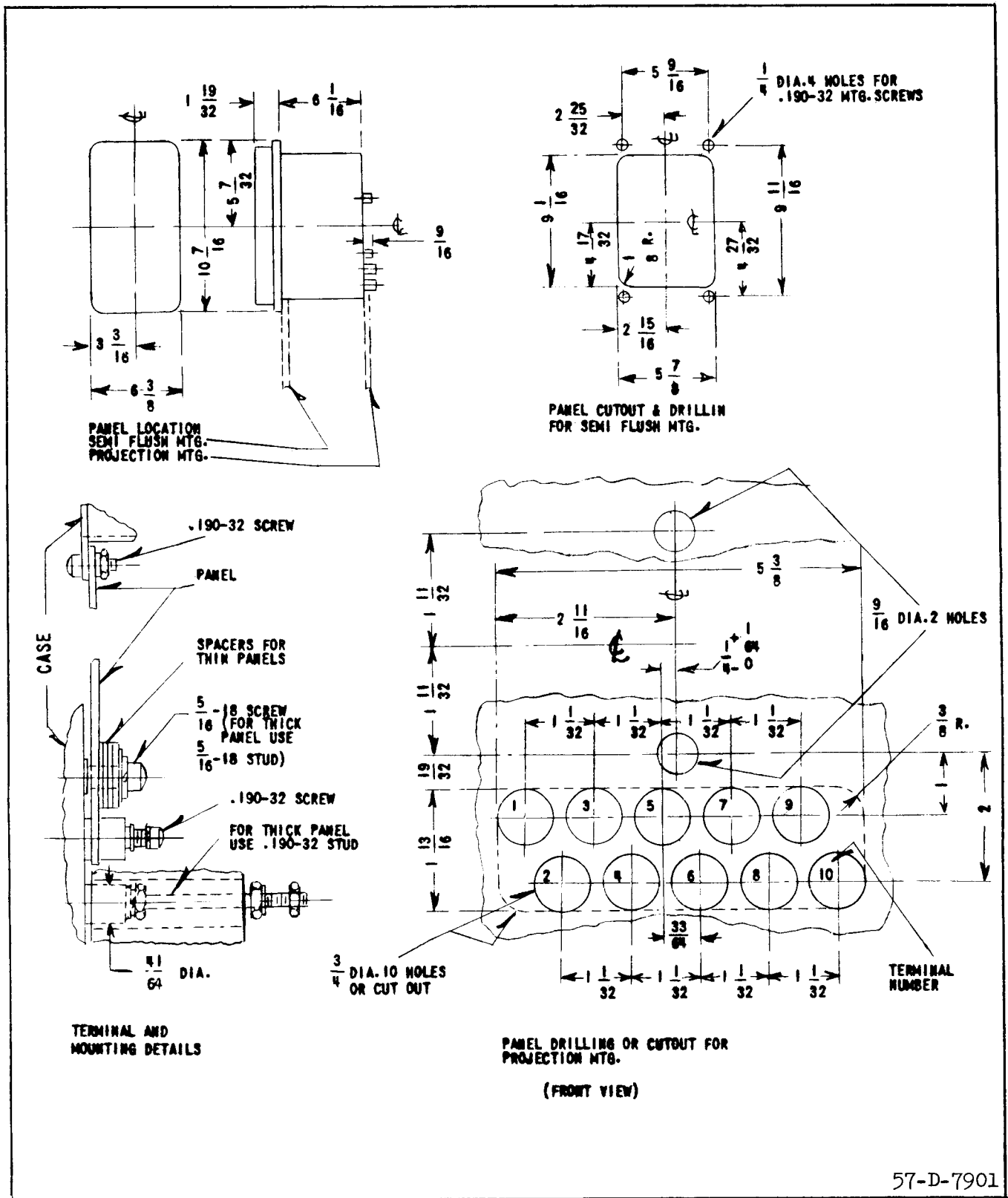
Fig. 37. Outline and Drilling Plan for the type PM-2, PM-23, PMA-1 and PMD relays in the type FT 21 case.
