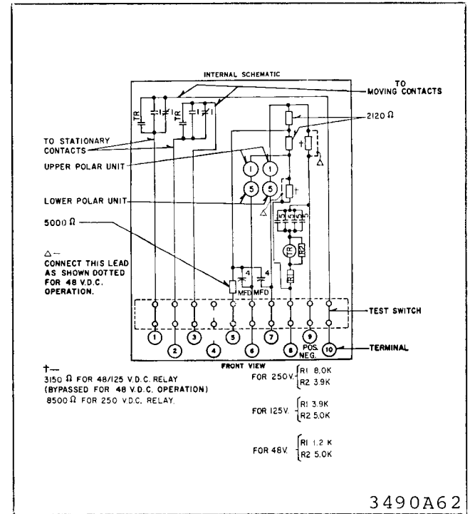
Fig. 24. PMD Relay - Ground Alarm, D.P.D.T. Contacts, Three Terminal Lines with Telephone Relay Output - FT-21 Case.
