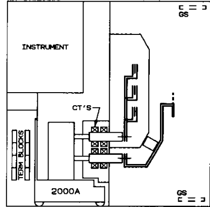
INSTRUMENT/BREAKER (TOP OR BOTTOM ENTRY)
