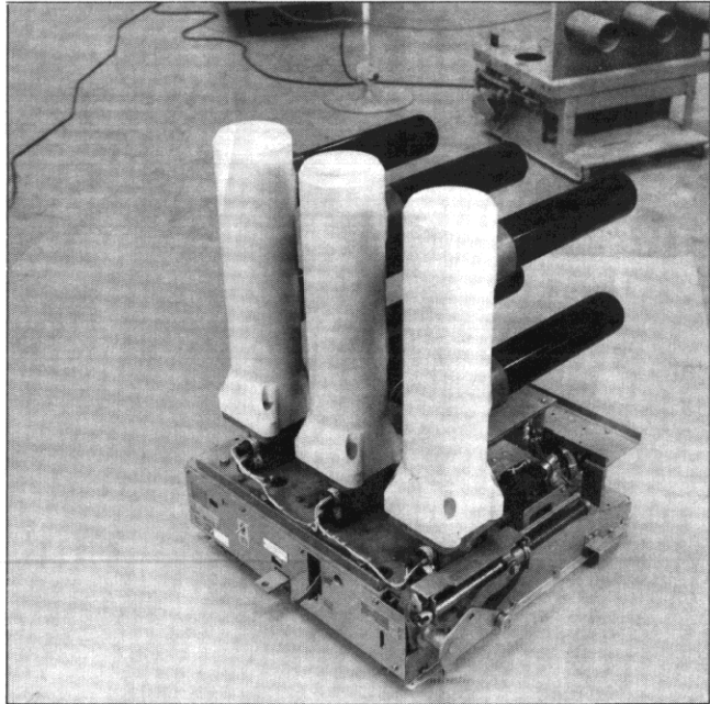
Type 27GHK 500, 1200 ampere circuit breaker (Personnel safety barrier has been removed).
