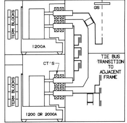
BREAKER/BREAKER (BOTTOM TIE) (TOP ENTRY) (CAN ALSO BE SUITED FOR BOTTOM ENTRY)
