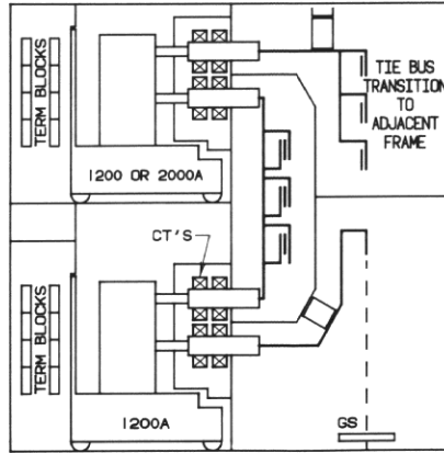
BREAKER/BREAKER (TOP TIE) (BOTTOM ENTRY) (CAN ALSO BE SUITED FOR TOP ENTRY)
