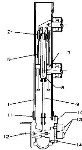
SF 6 INTERRUPTER CROSS SECTION
