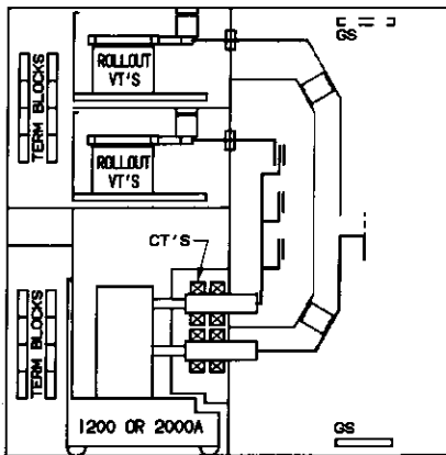
AUXILIARY/BREAKER (TOP OR BOTTOM ENTRY)
