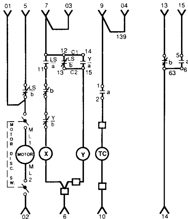
TYPICAL DC SCHEMATIC DIAGRAM OF CONTROL CIRCUIT
