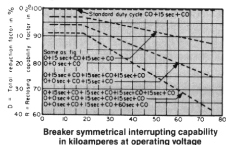
Fig. 2 Examples of Popular Reclosing Capabilities
