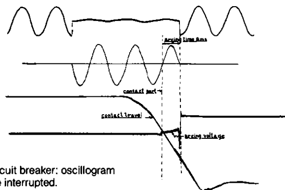
POLE DURING ARC QUENCHING SEQUENCE
