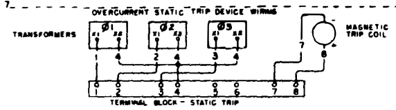
TYPICAL WIRING DIAGRAM FOR ELECTRICALLY OPERATED BREAKERS
