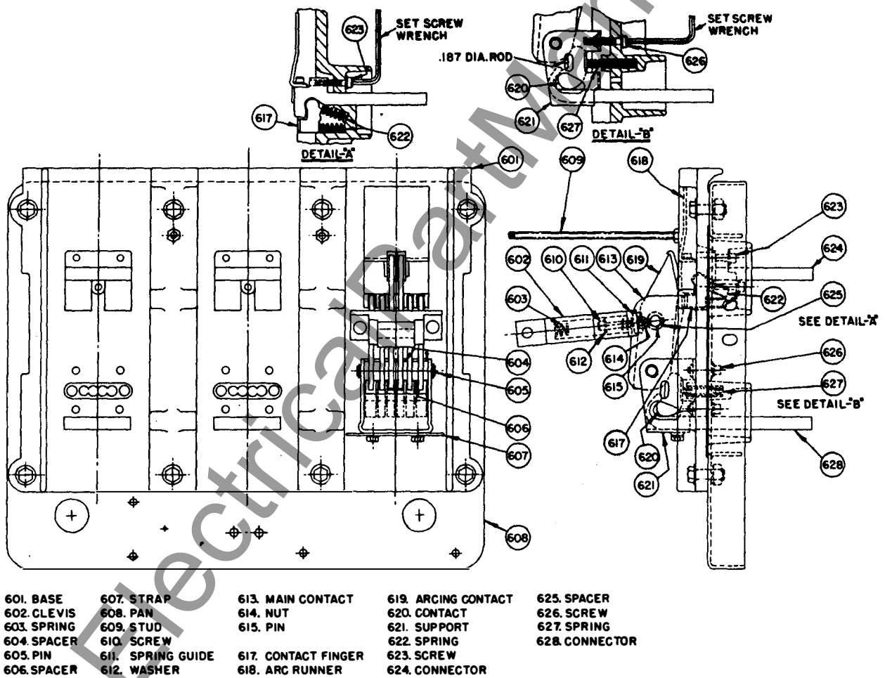
FIG.6 TYPICAL PANEL ASSEMBLY MARCH 8, 1967 72-340-021-401
