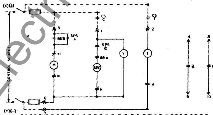
FIG. 2A TYPICAL OPERATING MECHANISM ELECTRICALLY OPERATED BREAKER MARCH 11, 1967 72-340-018-401
