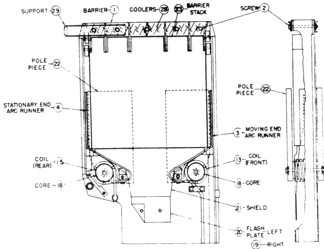
FIG 2 -B TYPICAL MA-350-C ARC CHUTE
