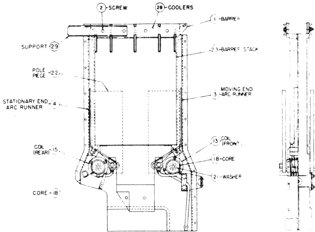
FIG 2 -A TYPICAL MA-150/250-C ARC CHUTE
