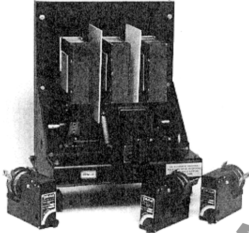
Electromechanical Trip Units
