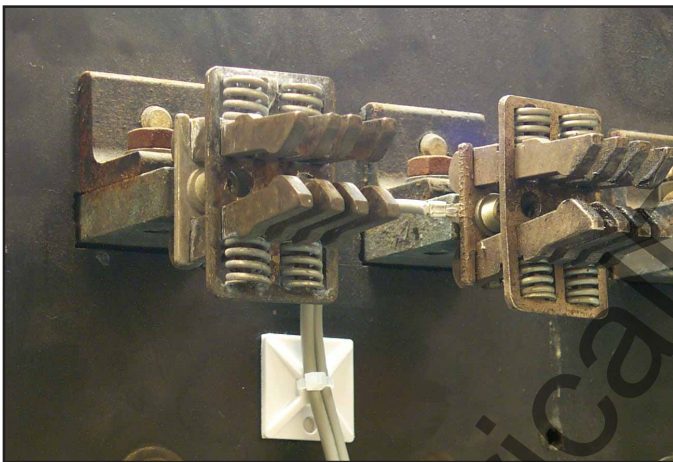
Fig. 36 HV Wires Connected to the Top Breaker Stabs.
