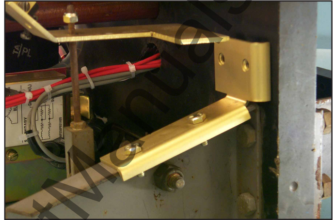
Fig. 43 DTA Mounting Bracket Installed on the Right Breaker Foot.
