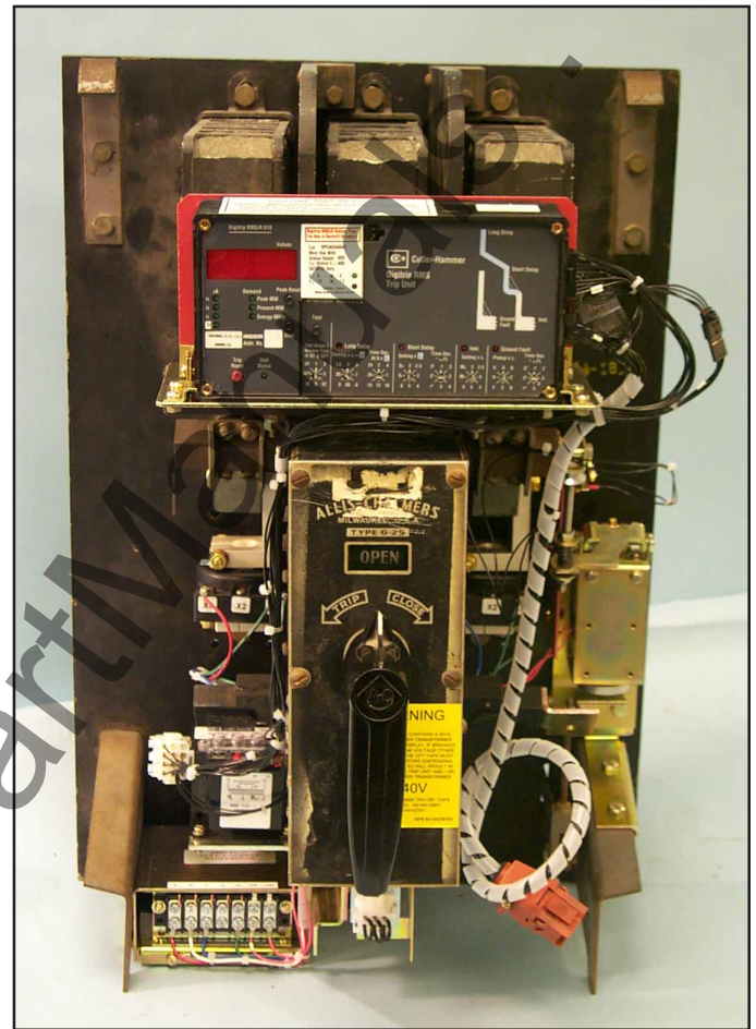
Fig. 59 Overview: External Harness Installed on the Breaker.
