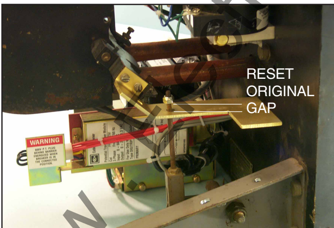
Fig. 42 Resetting the Interlock Mechanism.
