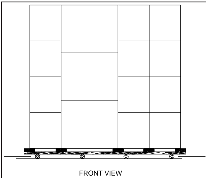
Figure 2-4 Assembly Rolling Procedure
