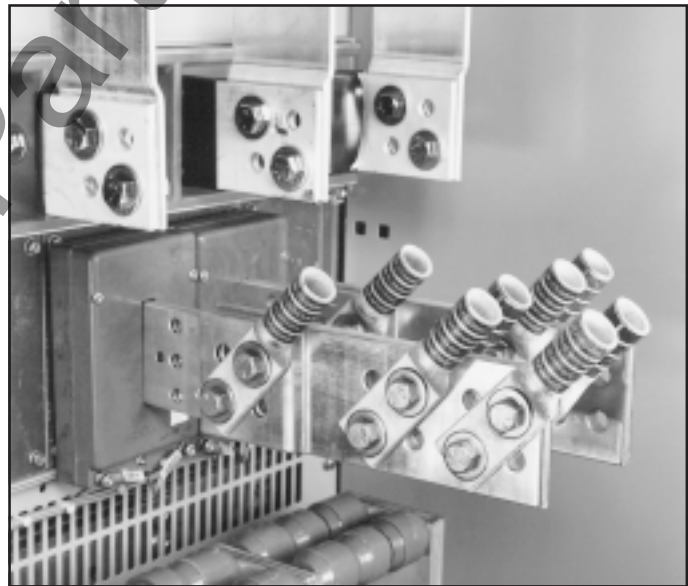
Figure 3-10 Load Runbacks with Lug Adapters
