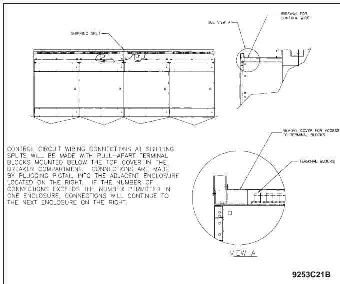
Figure 4-5 Shipping Split Control Terminal Block Connection
