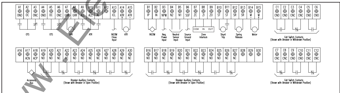
Figure 3-6 Secondary Disconnect Terminal Arrangement
