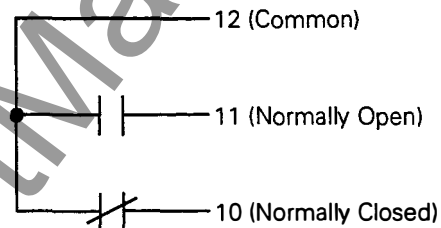
Figure 14. Bell Alarm with Lockout connections on the right terminal block. The contacts are shown in the reset state.
