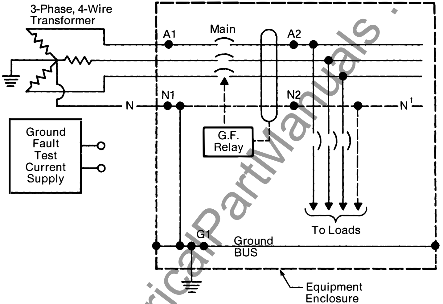
FIGURE 2 Main Breaker with G.F. Relay and Zero-Sequence Sensor Arrangement
