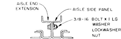
ASSEMBLY OF DETAILS J&K
