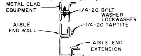
SHIPPING ASSEMBLY OF DETAILS AA&BB
