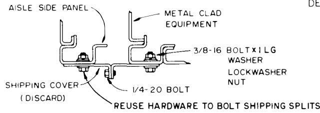
SHIPPING ASSEMBLY OF DETAILS S&T
