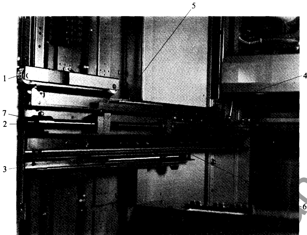
Fig. 37 Racking Mechanism
