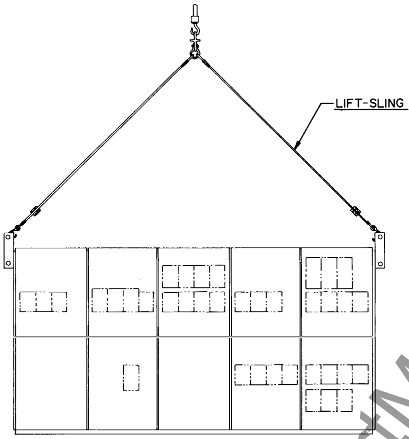
FRONT VIEW
