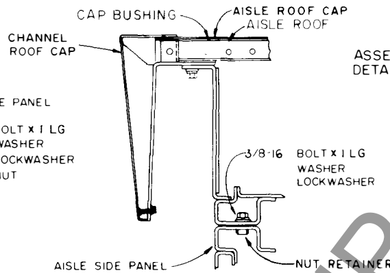
ASSEMBLY OF DETAILS L&M
