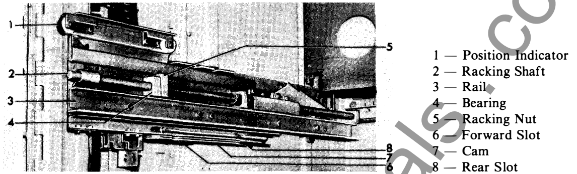
Fig. 41 Negative Interlock
