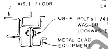
ASSEMBLY OF DETAILS E&F
