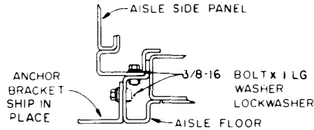
ASSEMBLY OF DETAILS C&D
