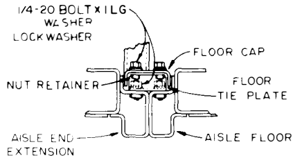
ASSEMBLY OF DETAILS A&B
