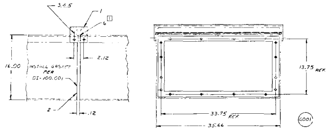
Fig. 32 Bus Duct Gasket
