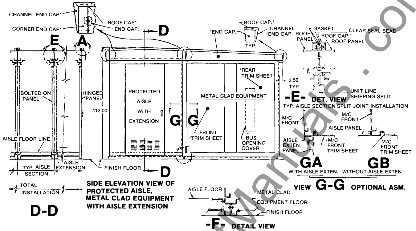
Fig. 7 (0209B4649-1 Rev. 1)
