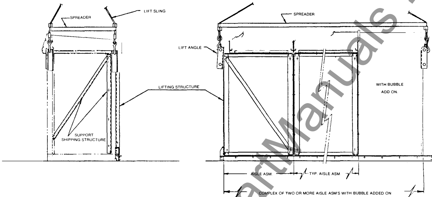
Fig. 7 (0209B4652 Rev. 0)
