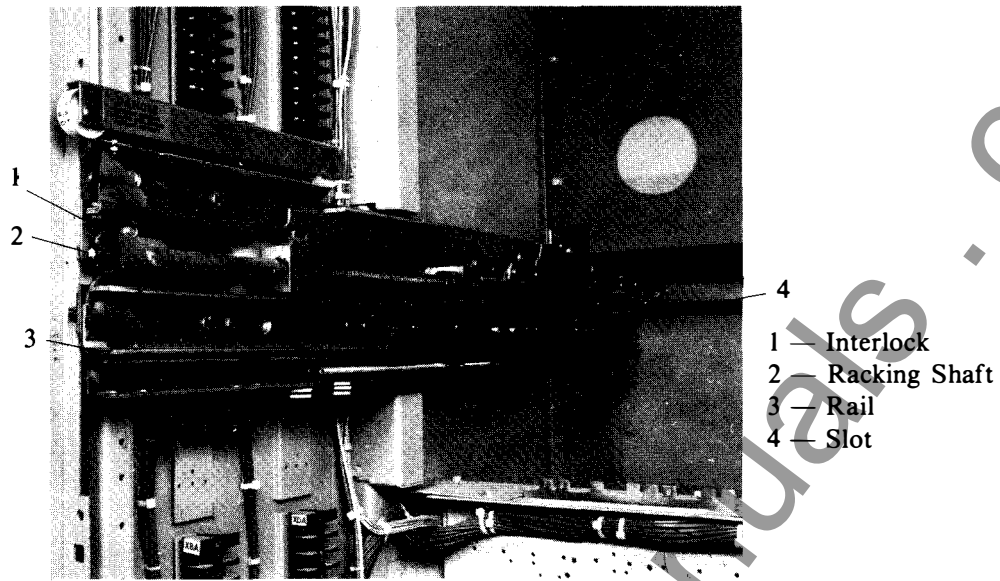
Fig. 40 Positive Interlock
