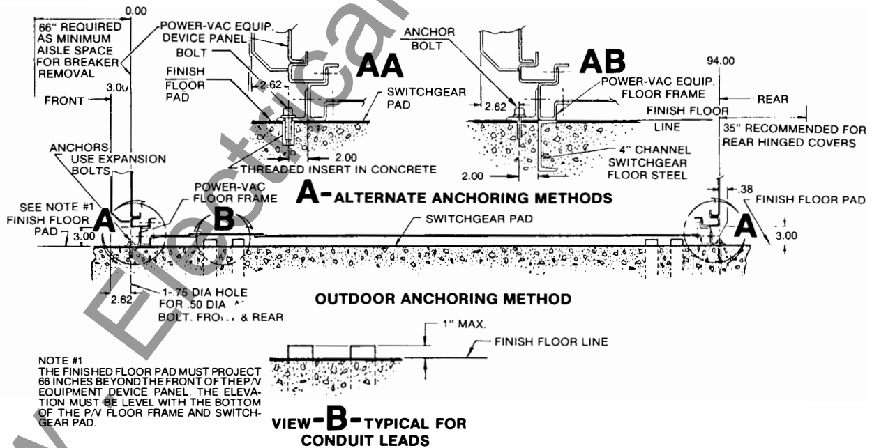
Fig. 6 (0209B4644 Rev. 4)
