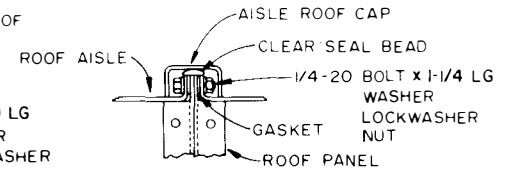
DETAIL R WITH END CAP REMOVED
