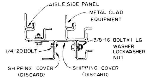
SHIPPING ASSEMBLY OF DETAILS W&X
