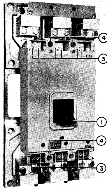
Fig. 2 — Front View of Circuit Breaker End Covers Removed
