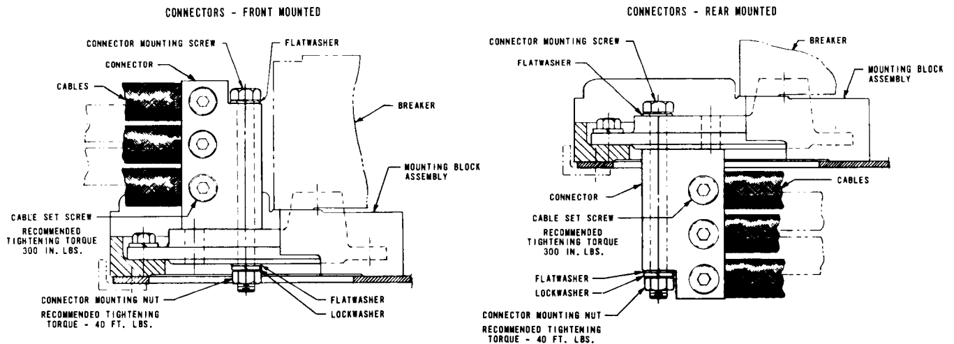
Fig. 5 — Connector Mounting
