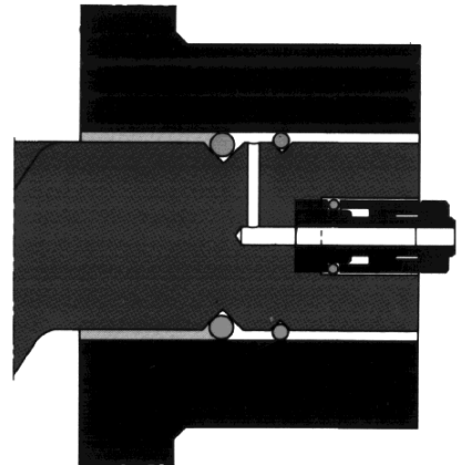
Diagram of a connecting flange with its two o-rings. The venting aperture is for the checking of the inner seal gastightness.
