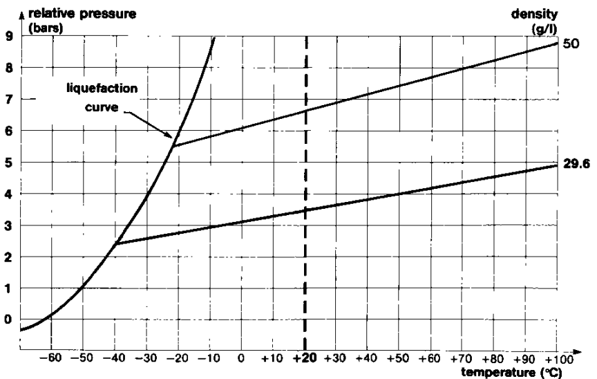
SF6 pressure variation versus temperature
