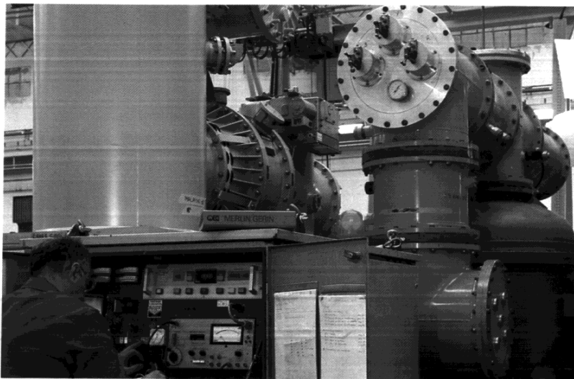
Dielectric routine tests using a gas insulated test unit
