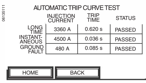
Figure 63: Automatic Trip Curve Test Screen
