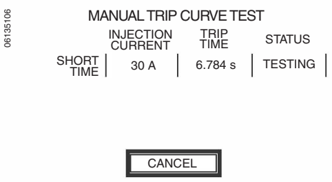
Figure 36: Manual Trip Curve Test Screen
