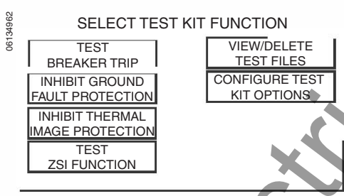
Figure 64: Select Test Kit Function Screen
