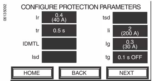
Figure 15: Configure Protection Parameters Screen
