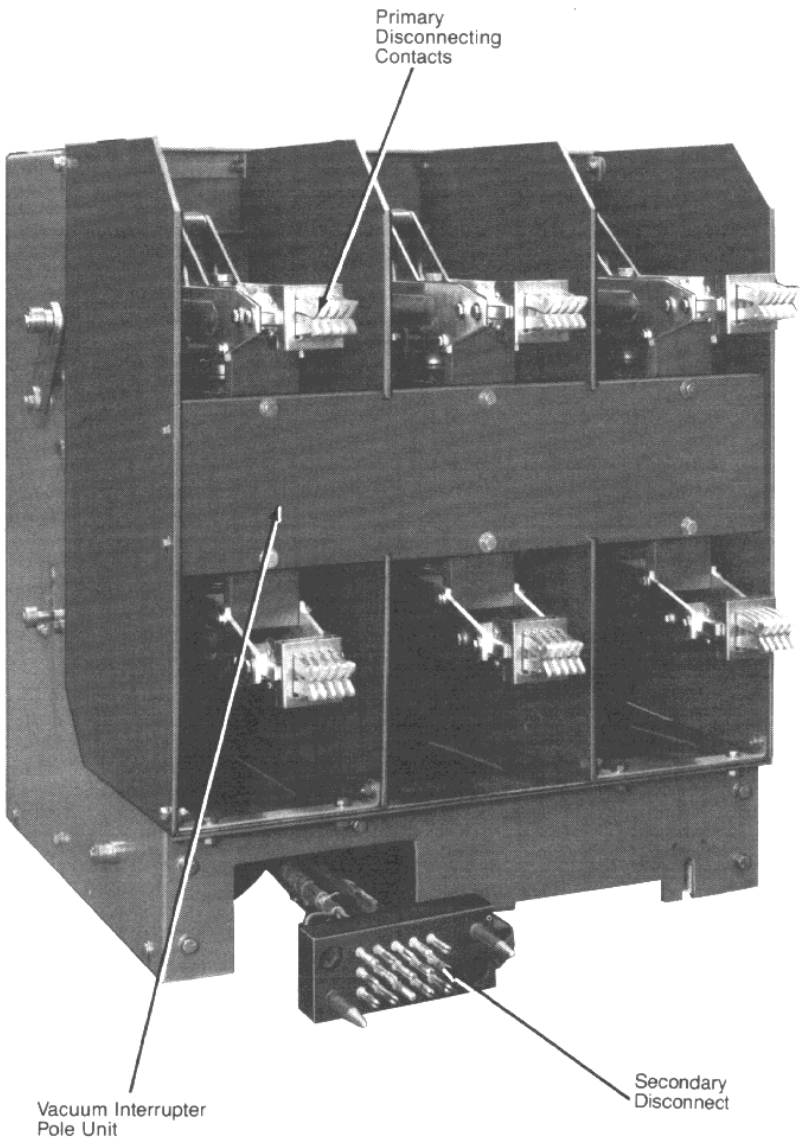
REAR VIEW
