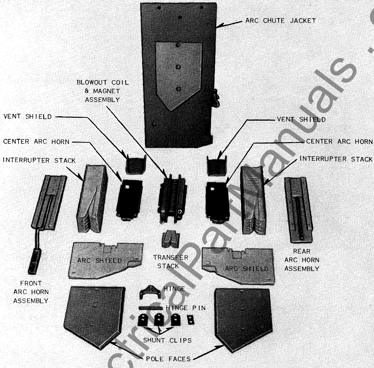
FIG. 10. Arc Chute Assembly
