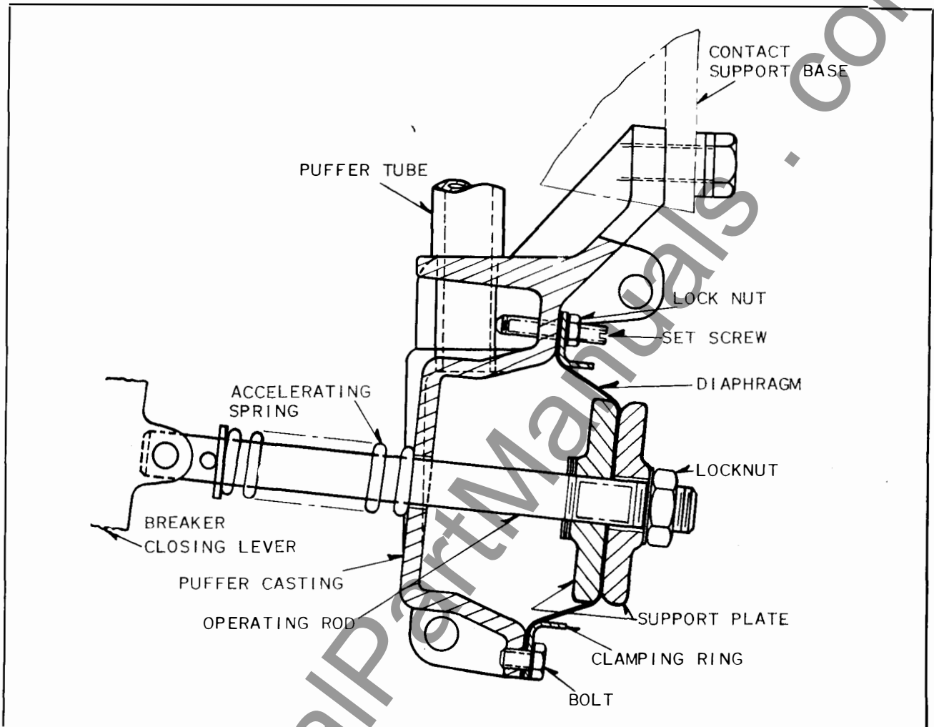
FIG. 5. Puffer Assembly
