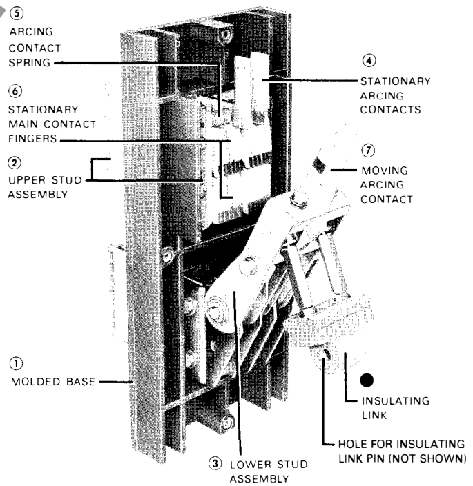
Fig. 11 Type DS-840 Pole Unit Assembly—Front View
