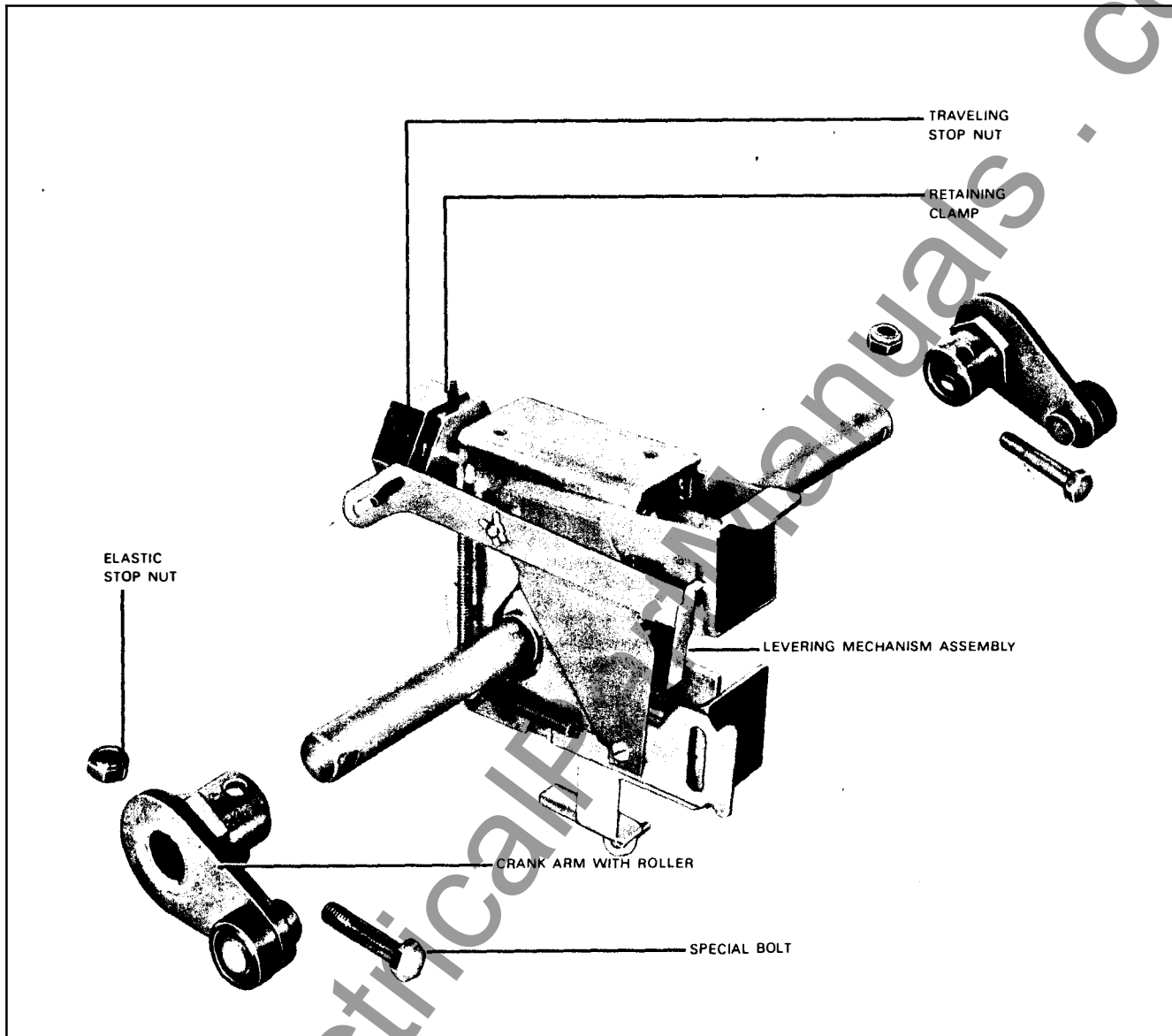
Fig. 18 Levering Mechanism
