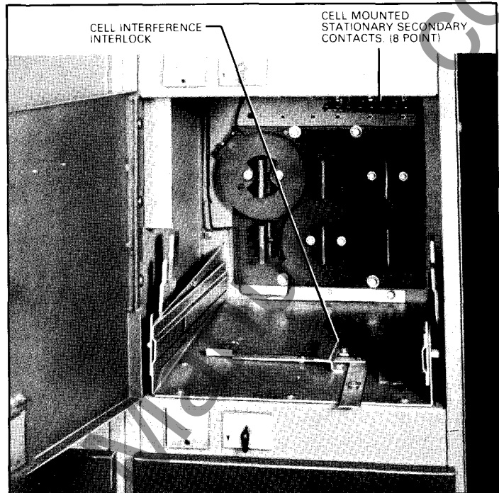
Fig. 34 Interference Bracket (set-up shown for a DS-416 breaker)
