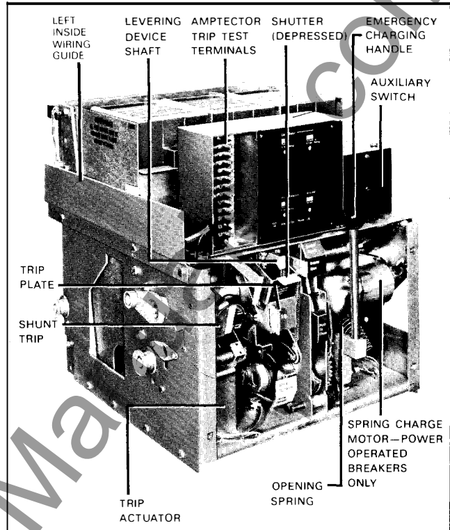
Fig. 2 DS 416 Breaker with Front Panel Removed
