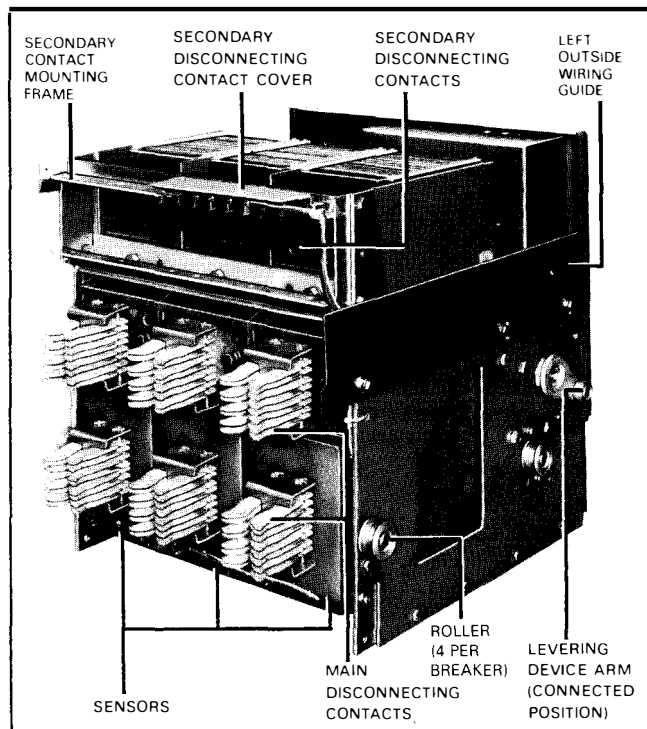
Fig. 3 Rear View Showing Levering Device Arm in CONNECT Position
