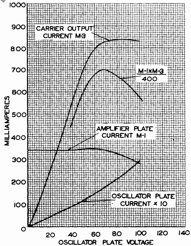
Figure 11 Oscillator Output Characteristics Using Eight Type 6L6 Tubes (50 ohm load).
