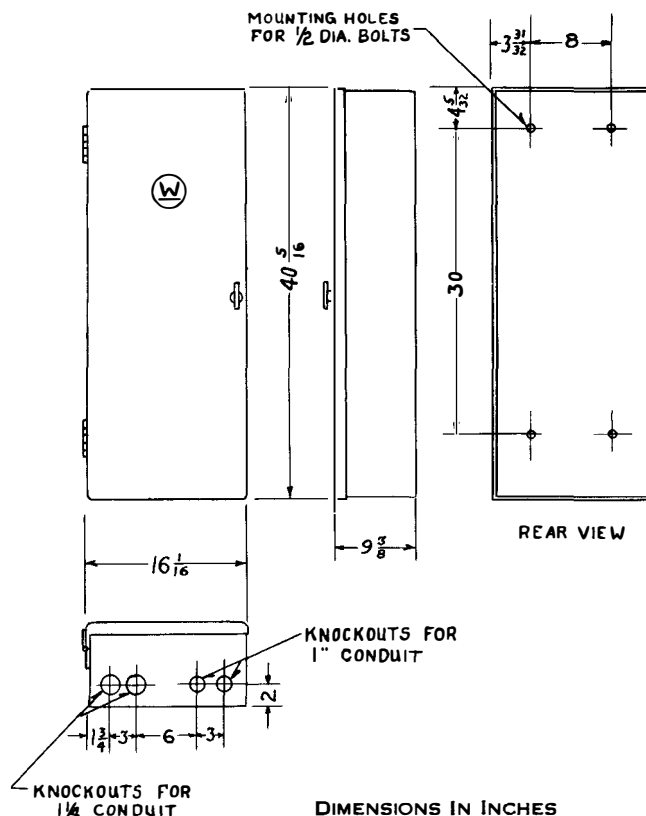
Figure 12 Outline and Drilling Plan for the Transmitter-Receiver Cabinet.
