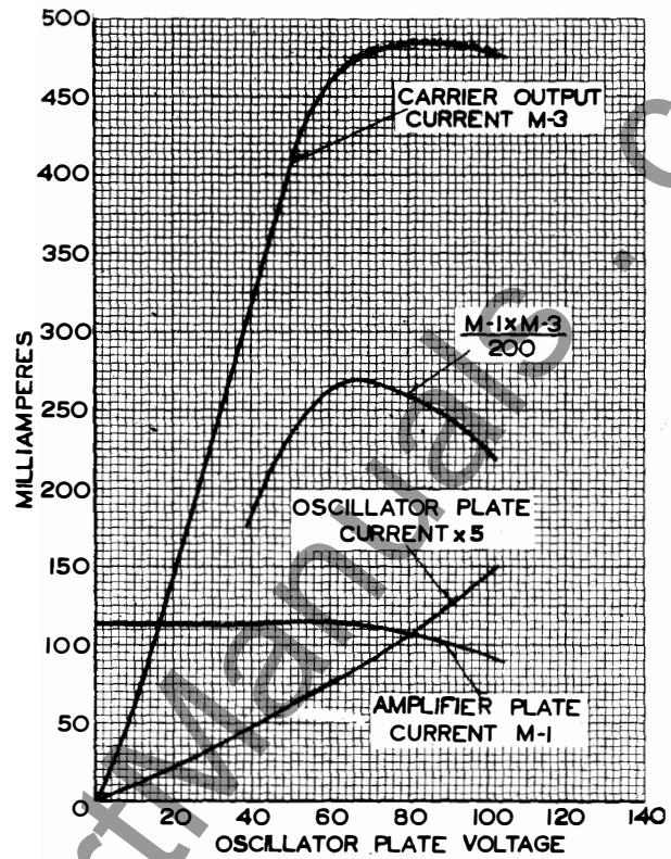
Figure 9 Oscillator Output Characteristics Using Four Type 6L6 Tubes (50 ohm load).
