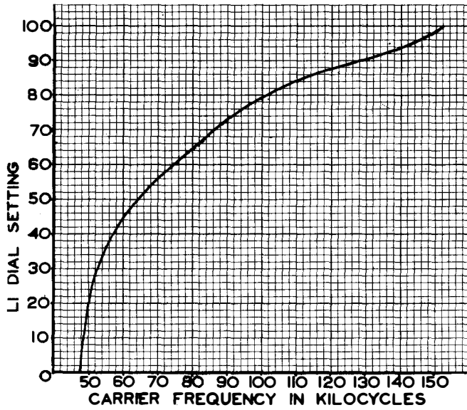
Figure 5 Frequency Calibration Curve of the Oscillator
