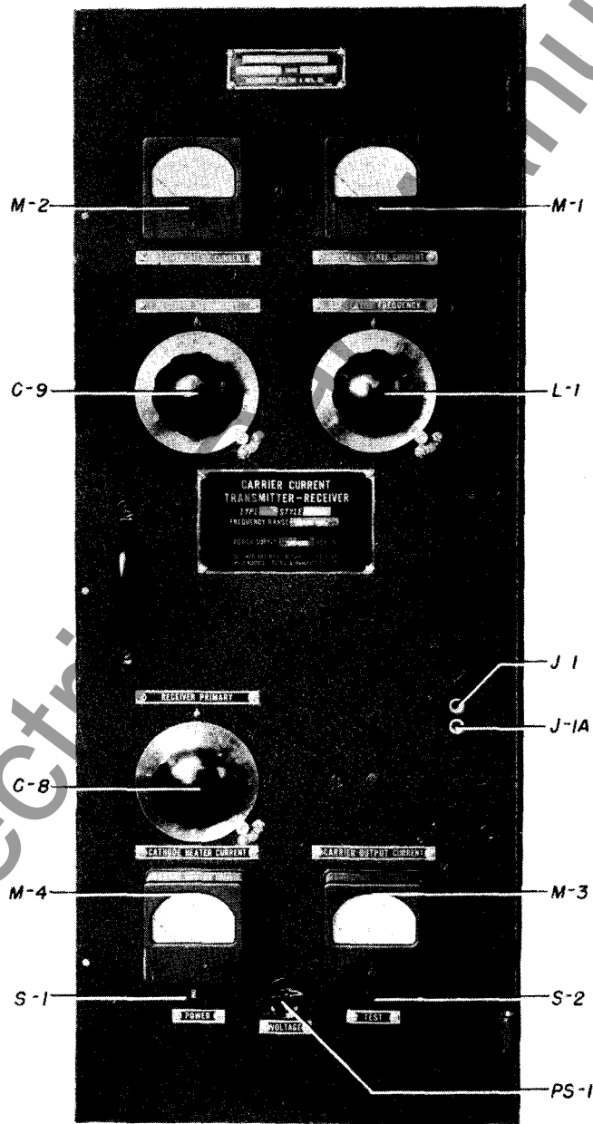
FIGURE 1 FRONT VIEW OF TRANSMITTER-RECEIVER (CABINET DOOR REMOVED)
