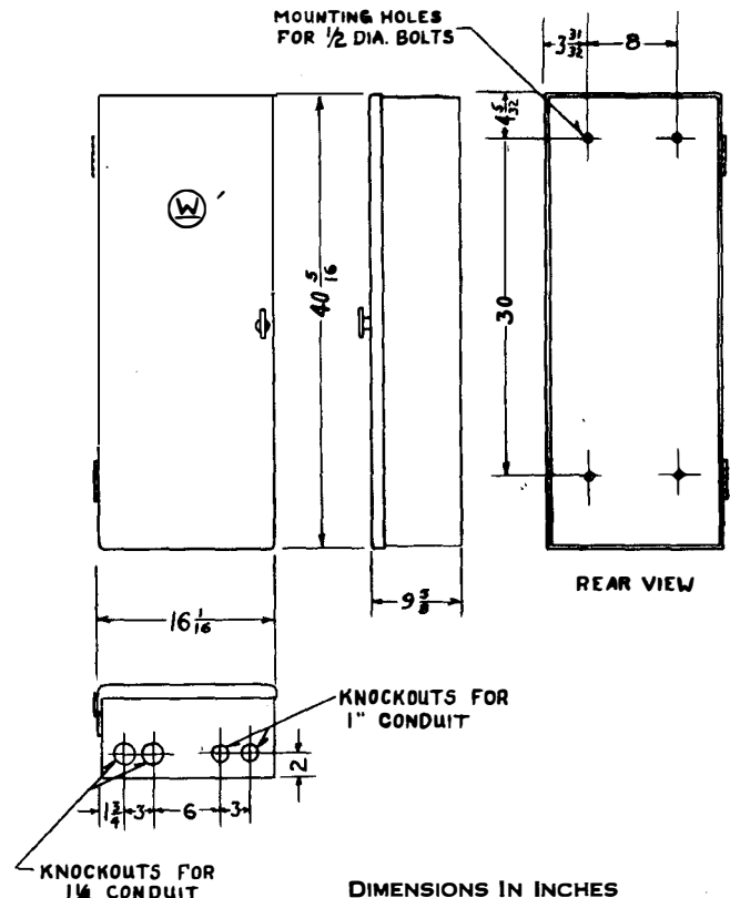
Figure 12 Outline and Drilling Plan for the Transmitter- Receiver Cabinet.
