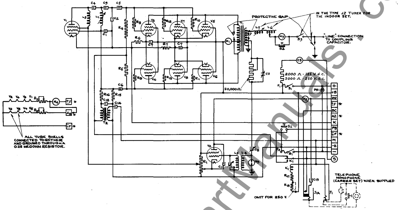
Figure 1 Internal Connections of the Type G0 Carrier Current Transmitter-Receiver with the Sleet Detection Equipment.
