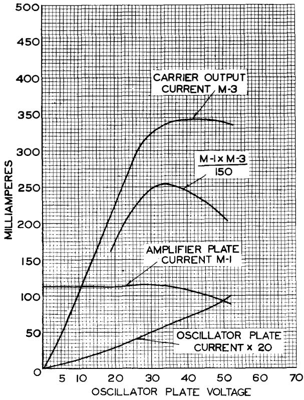
Figure 8 Oscillator Output Characteristics Using Four Type 25L6 Tubes (50 ohm load).
