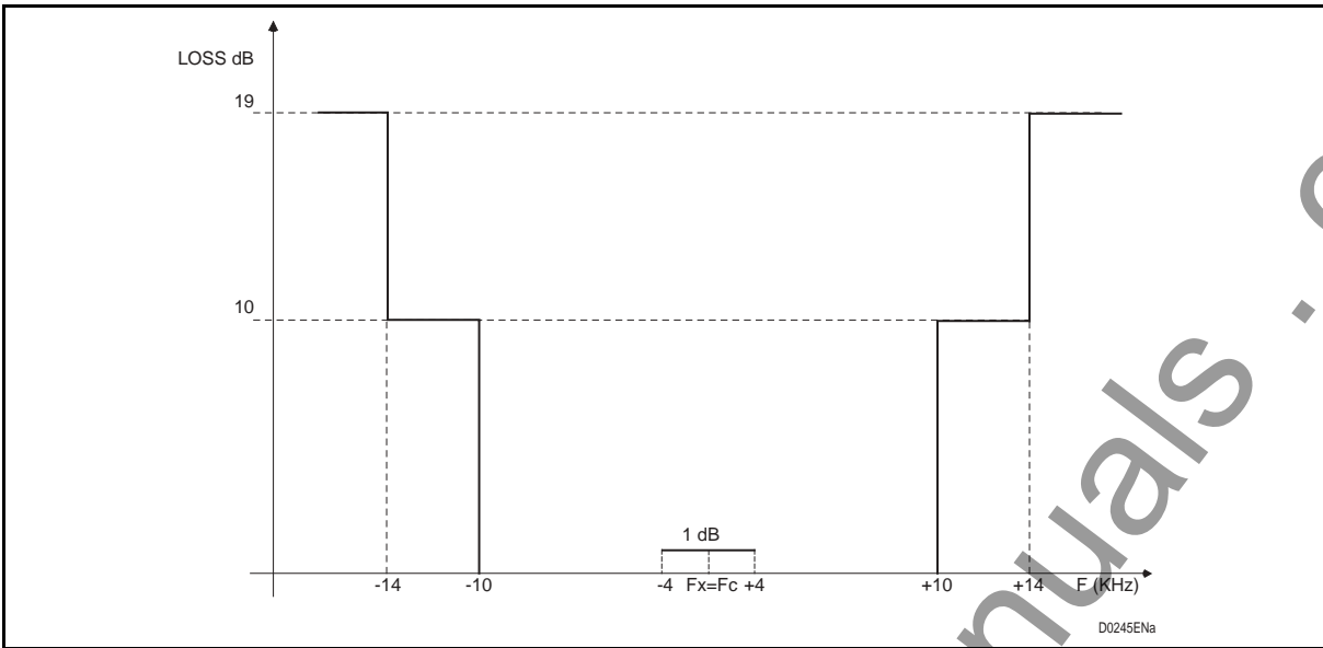
FIGURE 25 – FREQUENCY / LOSS MASK DOUBLE CHANNEL
