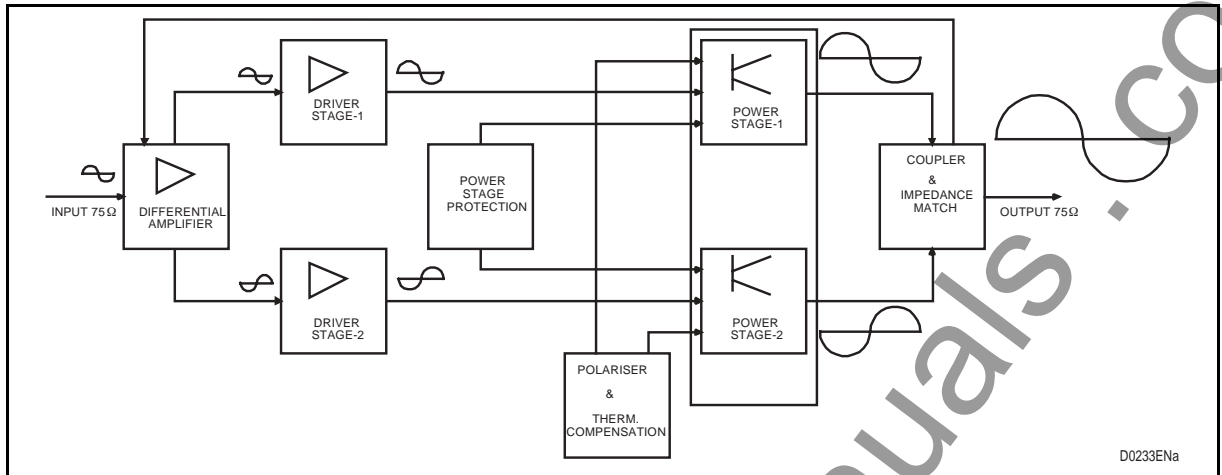
FIGURE 13 – 20 W AMPLIFIER
