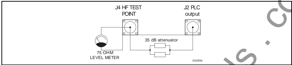
FIGURE 20 – HF TEST MEASUREMENT CONNECTORS
