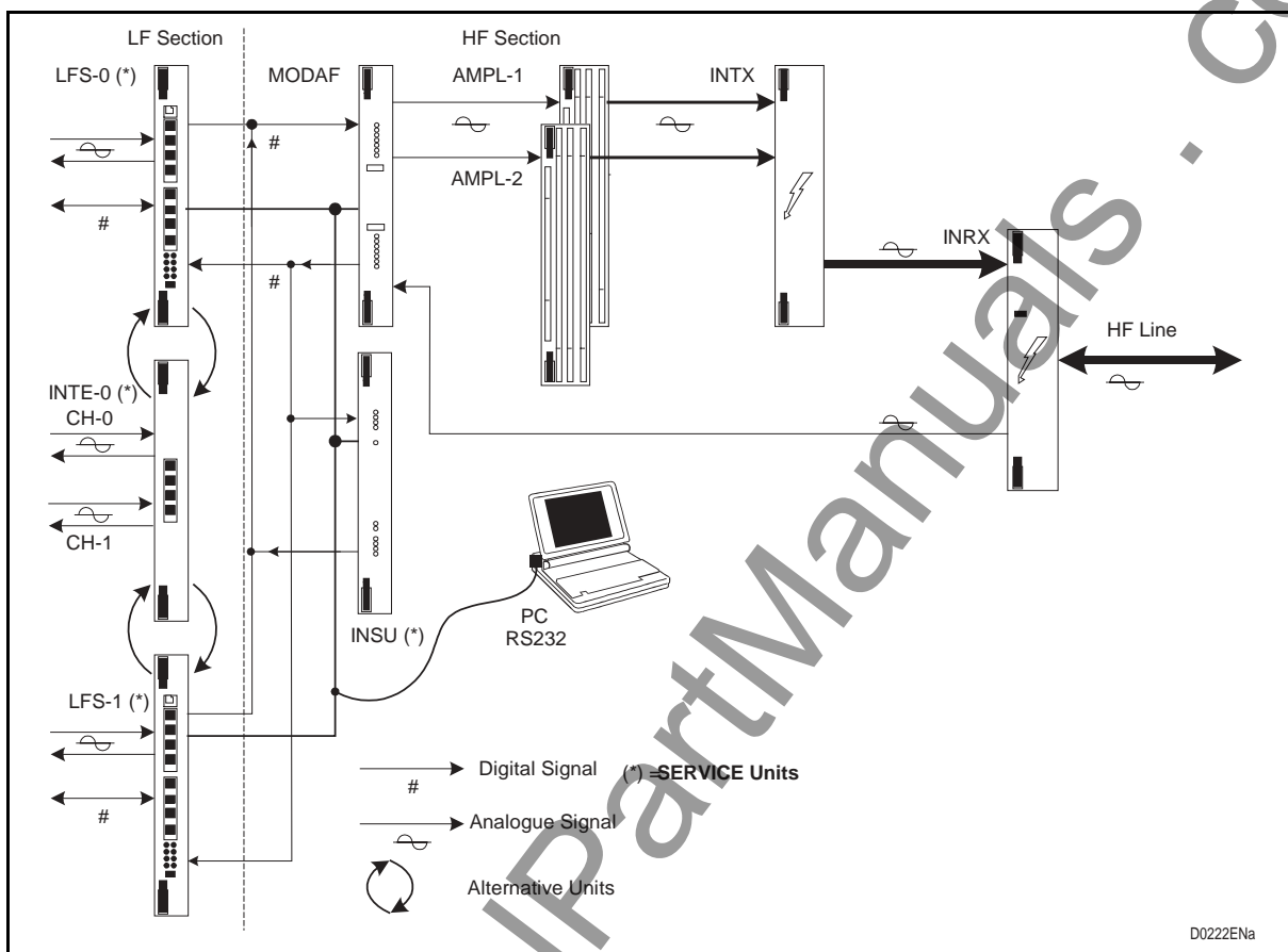
FIGURE 1 – PLC 1790/B REVISION2 FUNCTIONAL DIAGRAM
