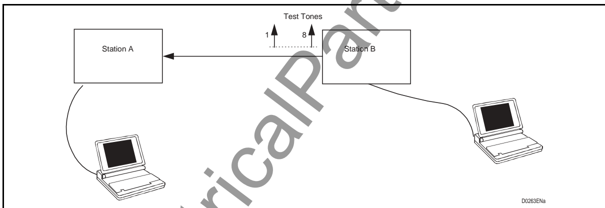
FIGURE 33 – EQUALIZATION PROCEDURE
