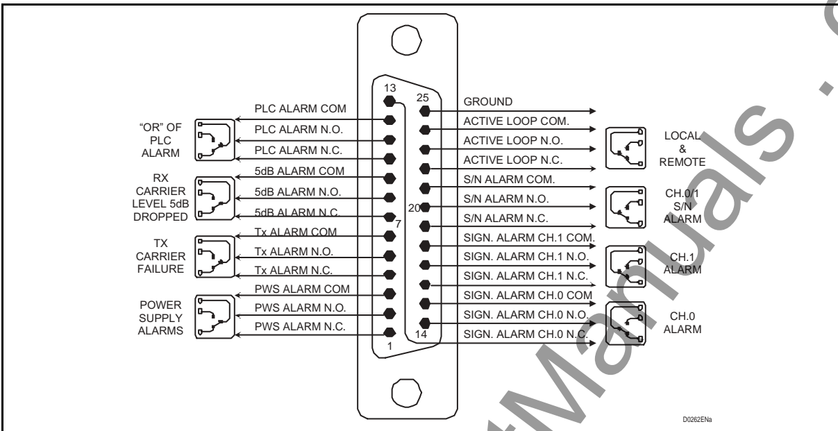
FIGURE 34 – M8 ALARM FIELD CONNECTOR
