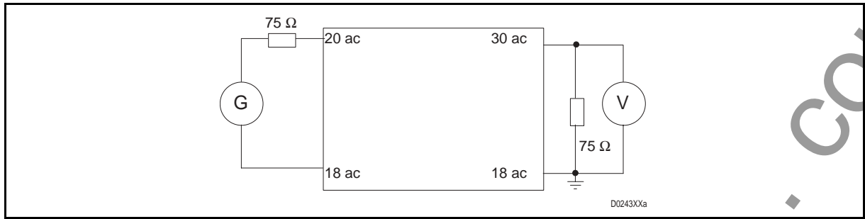
FIGURE 23 – RX FILTER TUNING TEST RIG
