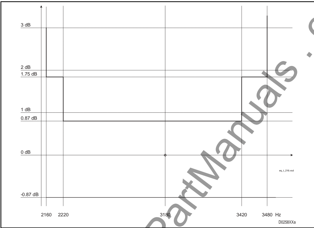
FIGURE 41 – TELEGRAPH CHANNEL 2160 ÷ 3480 HZ
