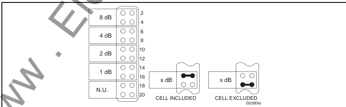
FIGURE 11 – INPUT / OUTPUT ATTENUATION CELL
