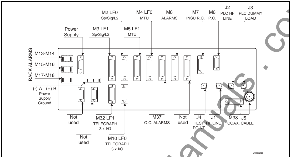
FIGURE 2 – FRONT SIDE PLC JUMPERS
