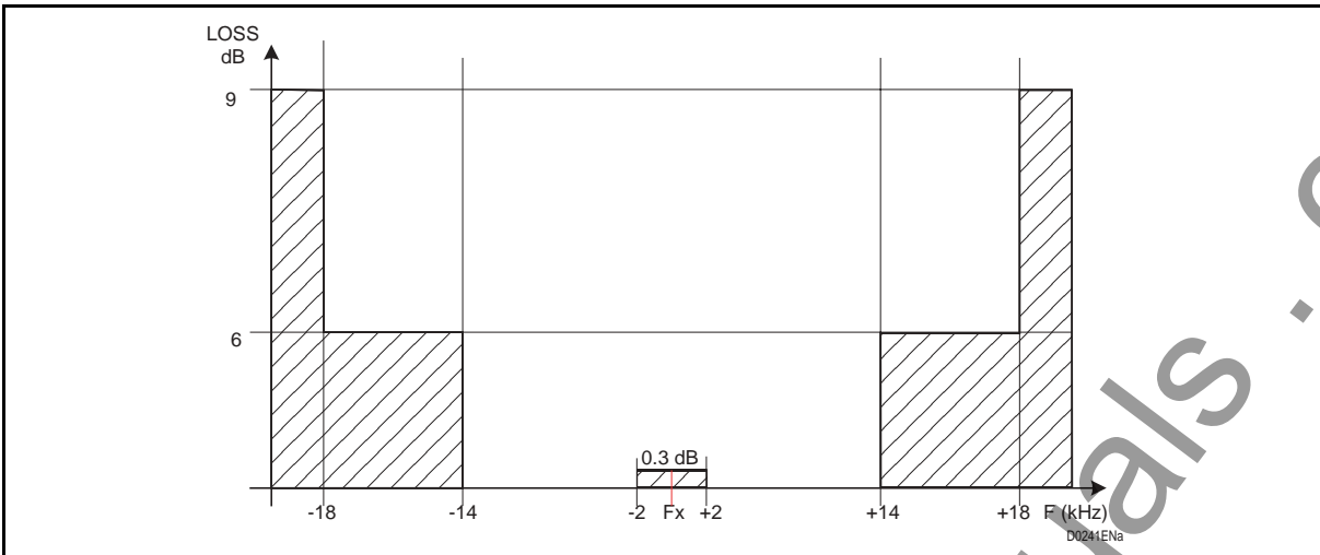
FIGURE 18 – FREQUENCY LOSS MASK FOR FC ≥ 396 KHZ-
