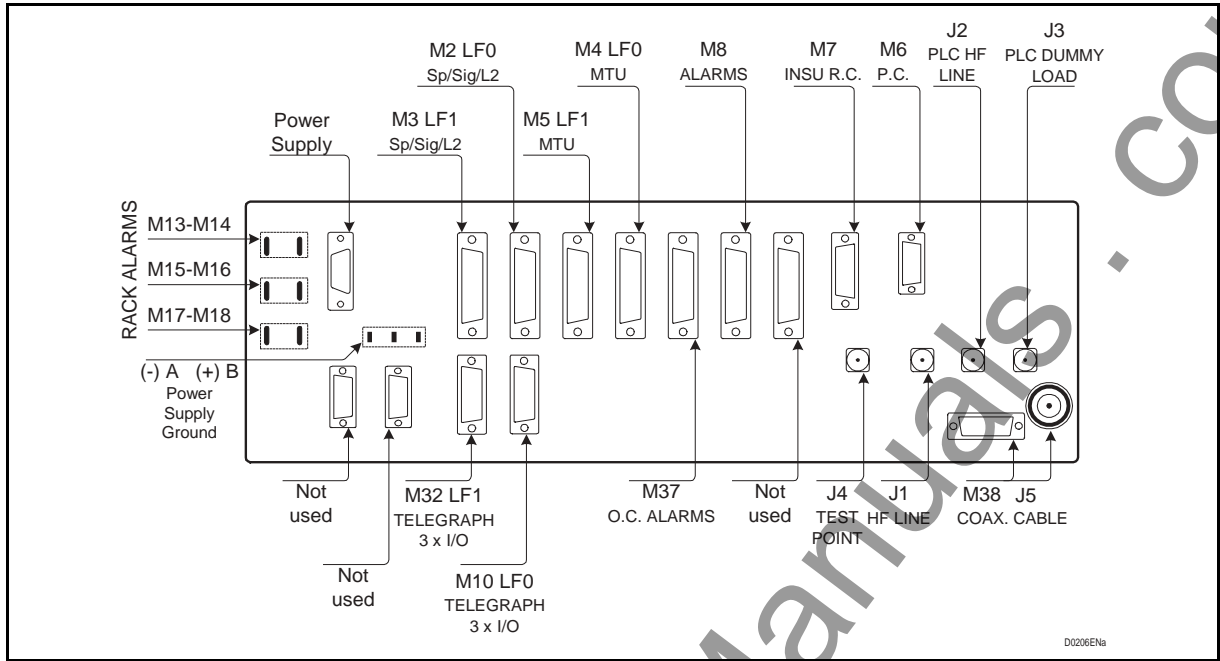
FIGURE 3 – FIELD INTERCONNECTION PANEL
