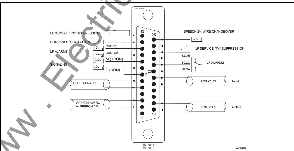
FIGURE 35 – LFS FIELD CONNECTOR M2 - LF0 OR M1 - LF1
