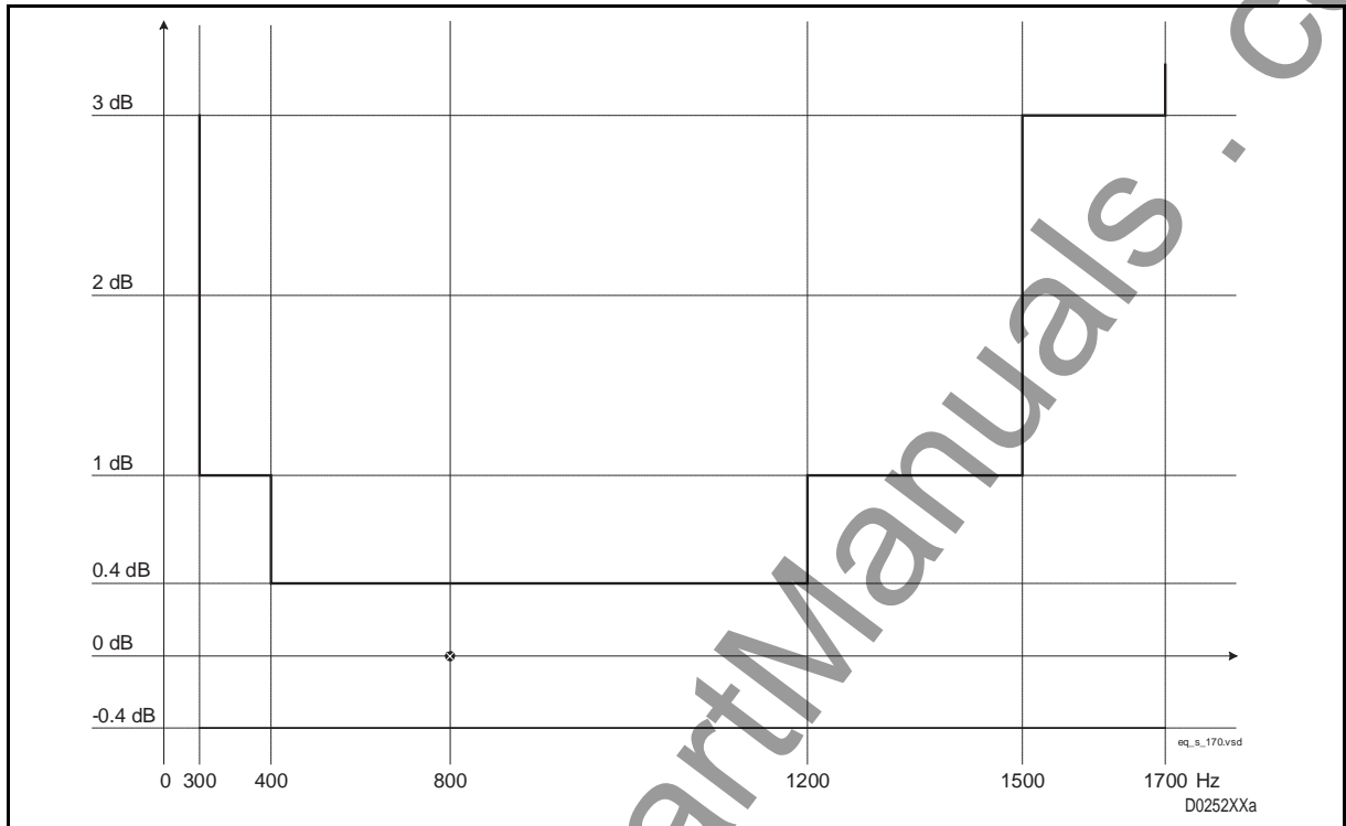
FIGURE 36 – SPEECH 300 ÷ 1700 HZ
