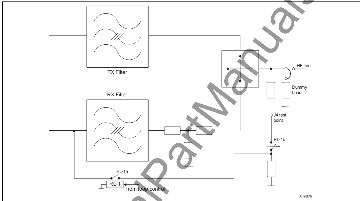
FIGURE 1 – LOCAL LOOP BLOCK DIAGRAM
