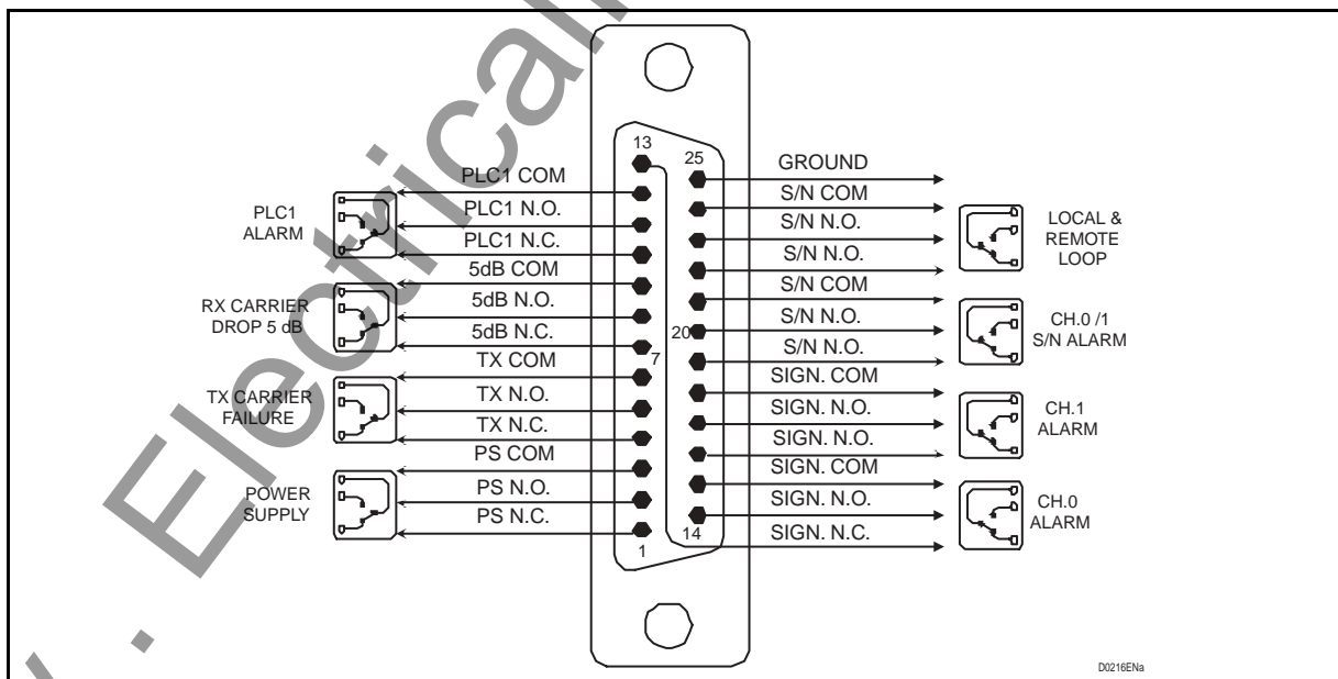
FIGURE 16 – M8 ⇨ ALARMS
