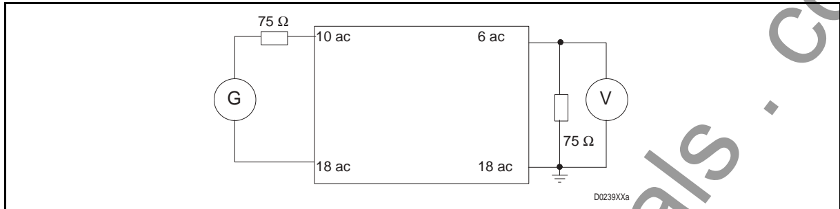
FIGURE 16 – TX FILTER TUNING TEST RIG
