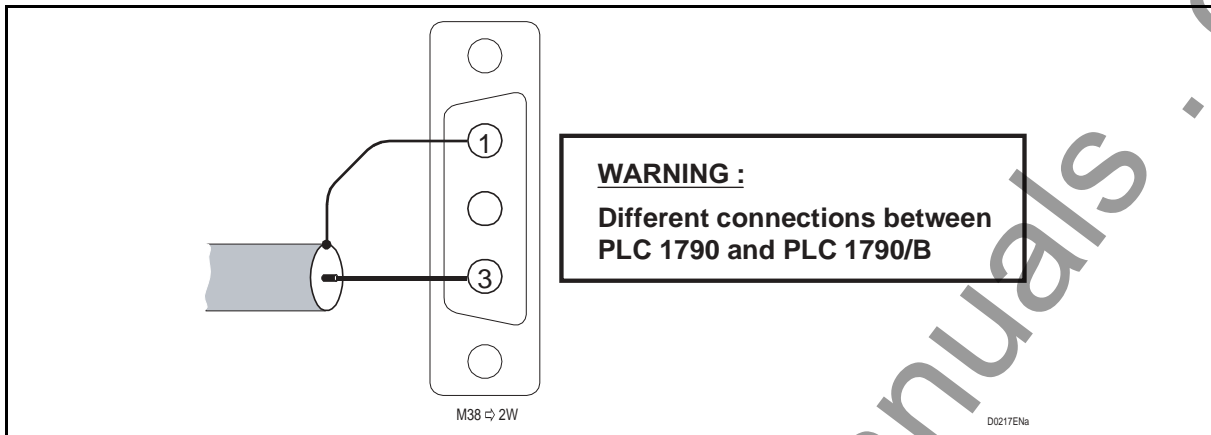
FIGURE 17 – HF CONNECTORS
