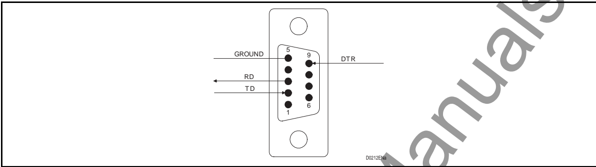
FIGURE 12 – M6 COMPUTER INTERFACE ( PROGRAMMING / MAINTENANCE )
