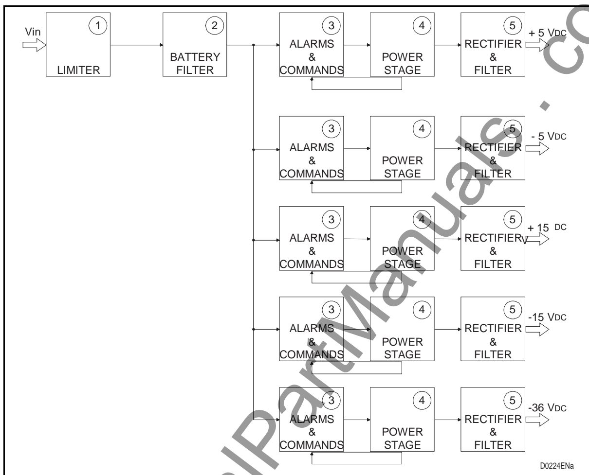
FIGURE 4 – POWER SUPPLY UNIT BLOCK DIAGRAM
