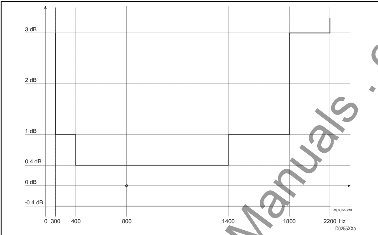
FIGURE 38 – SPEECH 300 ÷ 2200 HZ
