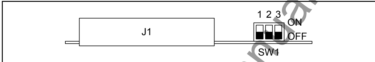
FIGURE 5 – ALIM SWITCH
