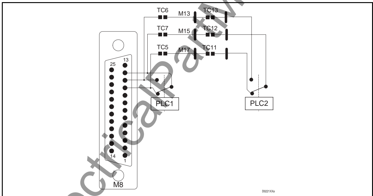
FIGURE 21 – CABINET ALARM CONNECTOR
