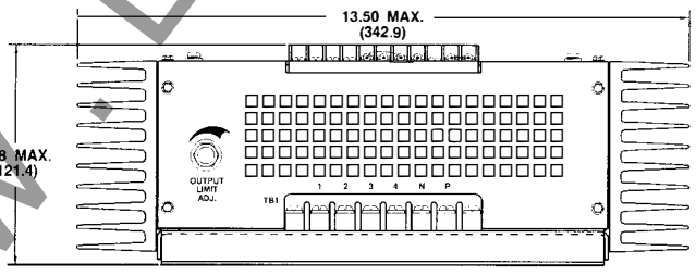
FIGURE 3. OUTLINE DRAWING.
