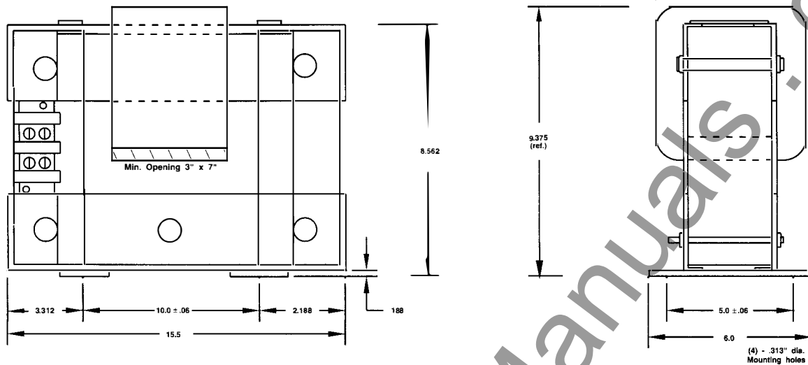
FIGURE 7. OUTLINE DRAWING BE 25929-001.
