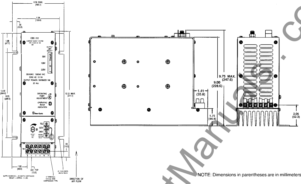
FIGURE 2. OUTLINE DRAWING.
