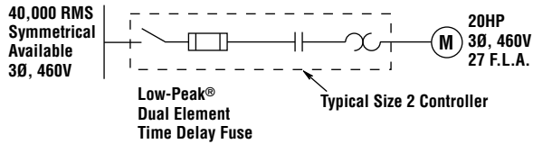
Figure 15. Short-Circuit Protection of Motor Controller
