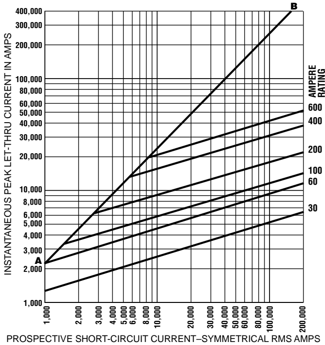
LPN-RK_SP – RMS & Peak Let-Thru Currents (kA)
