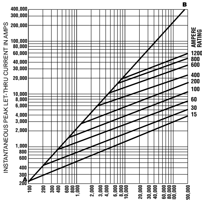
PROSPECTIVE SHORT-CIRCUIT CURRENT—SYMMETRICAL RMS AMPERS
