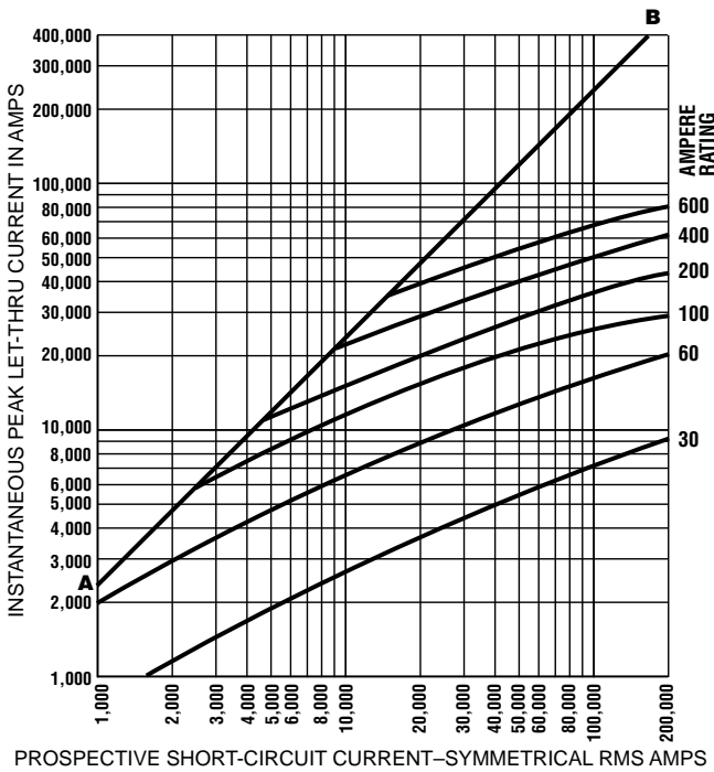
FRN-R – RMS & Peak Let-Through Currents (kA)
