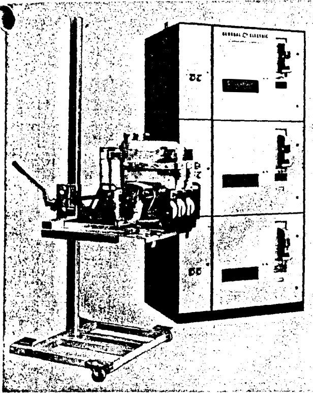
Fig. 13. A lifting device should be used to assure safe handling of the contactor during moving
