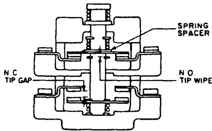
Fig. 44. Interlock block with one set of normally open contacts and one set of normally closed contacts in operated position
