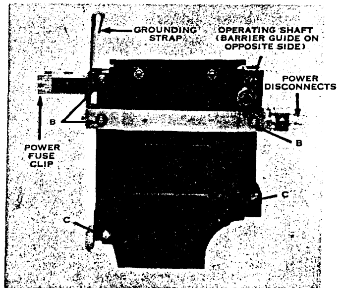
Fig. 20. Arc-chute assembly with power fuse clip, grounding strap and power disconnects
