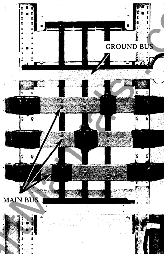
Figure 28. Rear view of horizontal main and ground bus with back covers removed
