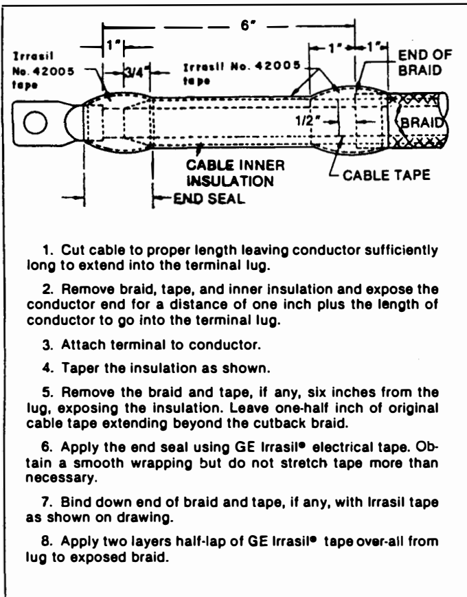
Figure 34. Termination of varnished-cambric-insulated, non-shielded, non-lead-covered, 5000-volt cable
