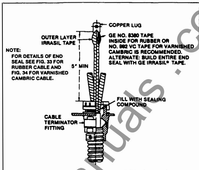
Figure 35. Termination of interlocked-armor, non-shielded, 5000-volt cable
