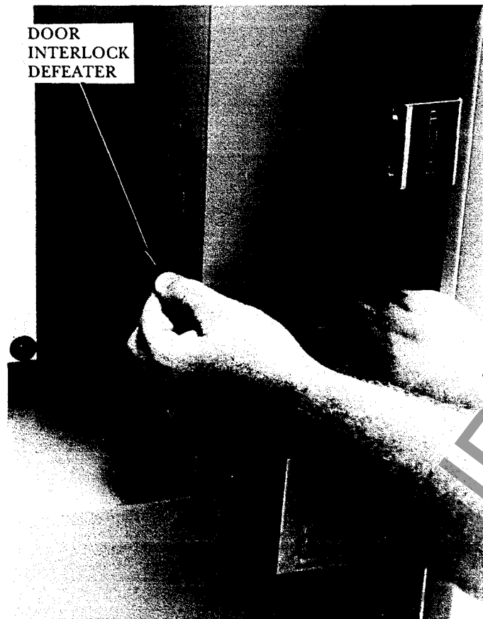
Figure 48. Lift defearer bracket while pulling high-voltage door
