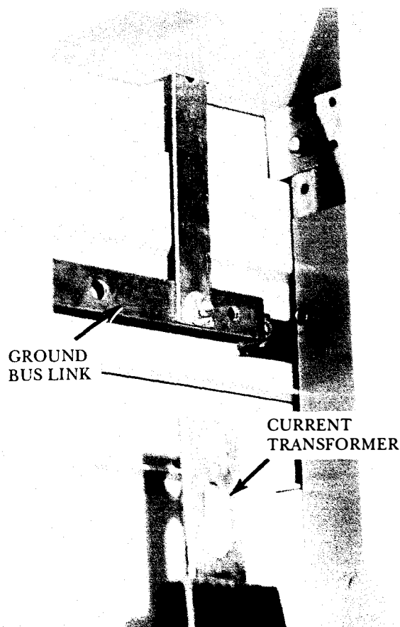
Figure 29. View of motor terminal area showing ground bus link in lower starter
