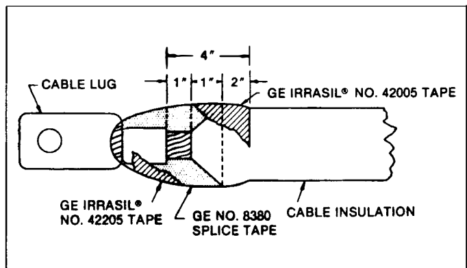
Figure 33. Termination of rubber-insulated, non-shielded, non-lead-covered, 5000-volt cable
