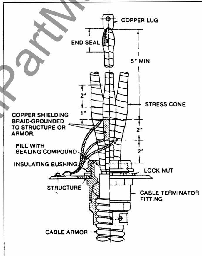
Figure 36. Termination of interlocked-armor, shielded, 5000-volt cable
