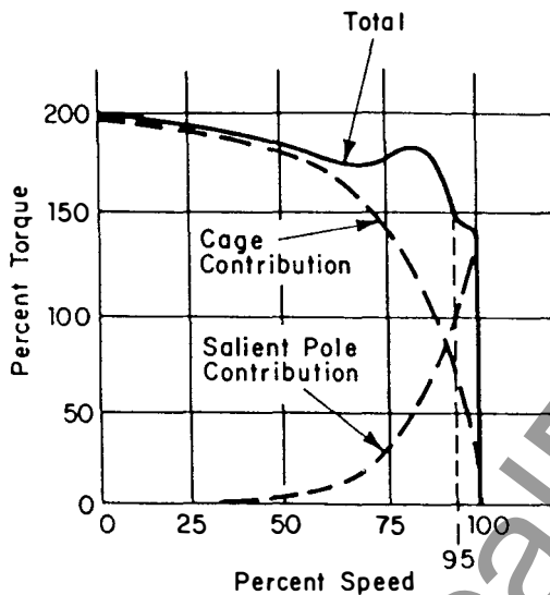
Fig. 4a. High-starting-torque motor
