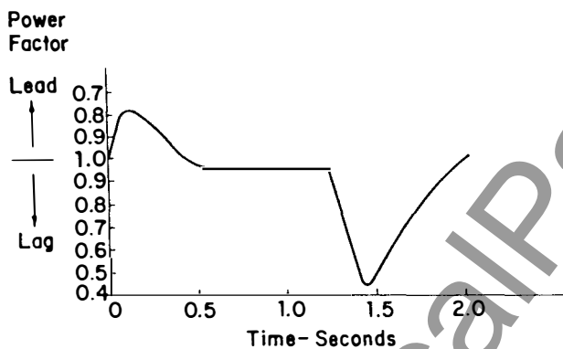
Fig. 21. Motor power-factor response to a two-second line-voltage dip: solid-state exciter
