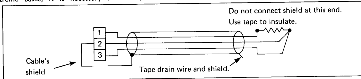
Figure 5.9 – RTD Wiring
