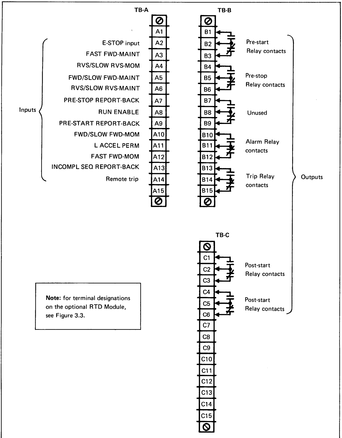
Figure 8.3 – Terminal Designations
