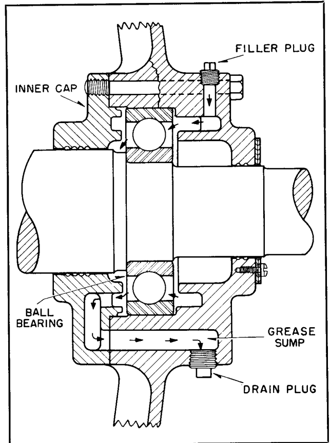
FIG. 4. Typical Ball Bearing
