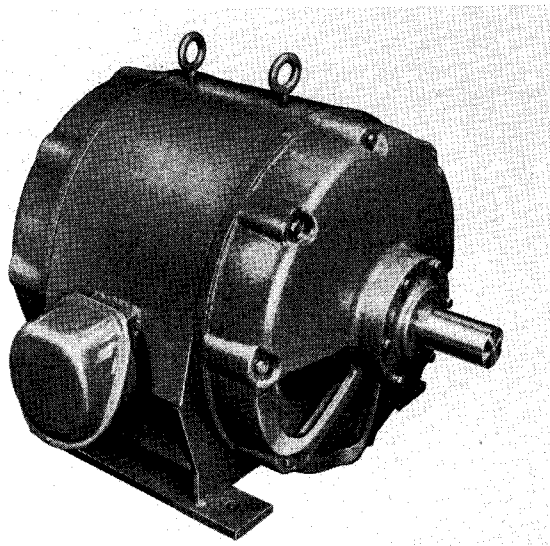
FIG. 1. Open Drip-Proof Ball Bearing Type CSP Life-Line Motor, Frames 580-683
