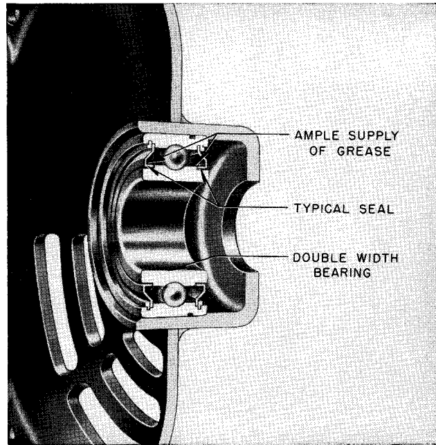
FIG. 3. Sectional View—Pre-lubricated Ball Bearing
