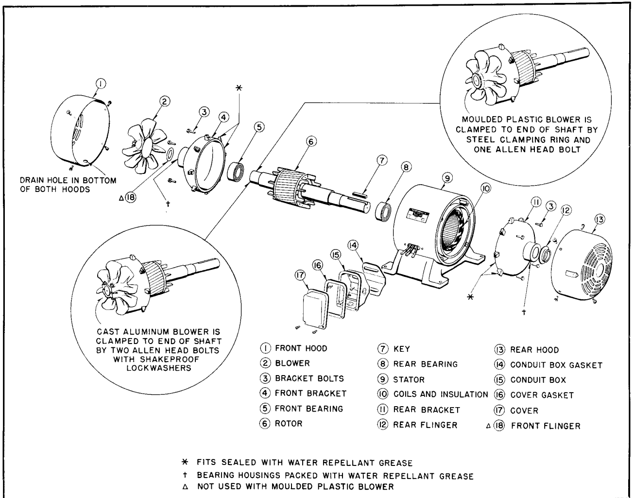
FIG. 2. Arrangement of Parts—Totally Enclosed Fan-Cooled Type CSP Motor (Frames 224-326)
