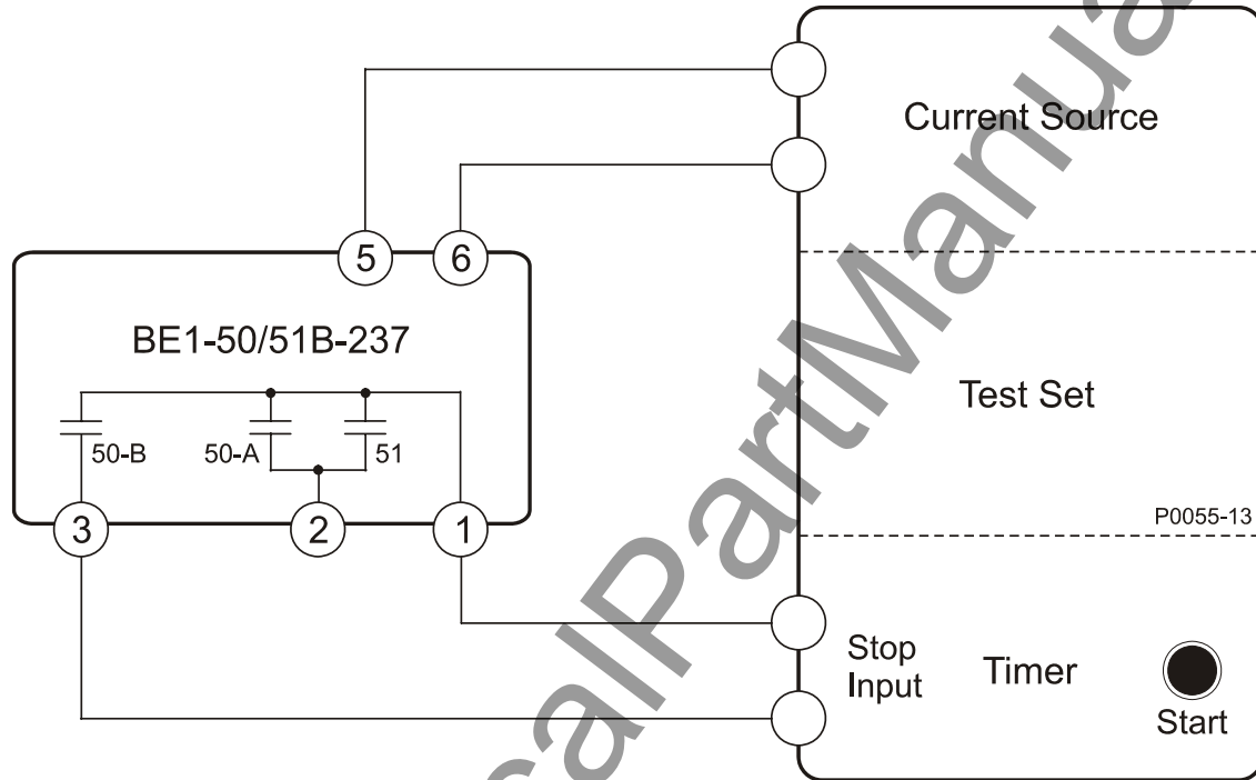
Figure 5-2. 50-B Pickup Test Setup
