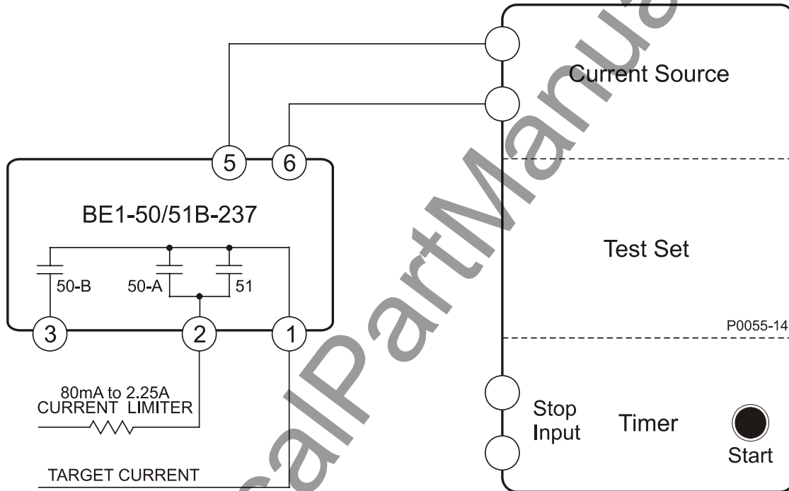
Figure 5-3. Target Indicator Test Setup
