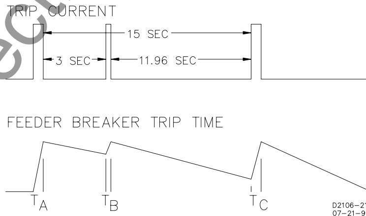
Figure 4-5. Coordination Timing Diagram
