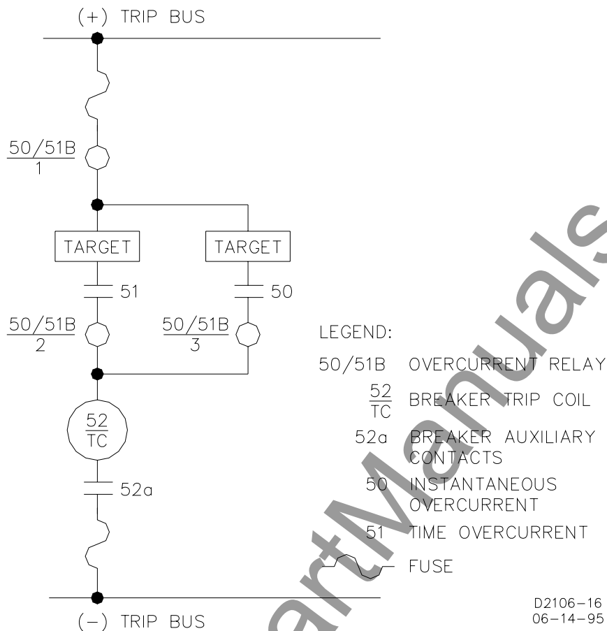
Figure 4-7. DC Control Connections
