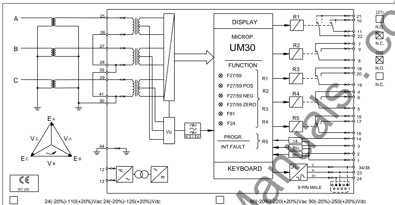
Figure 2. Wiring Diagram for the UM30 Three-Phase, Frequency and Universal Voltage Relay.
