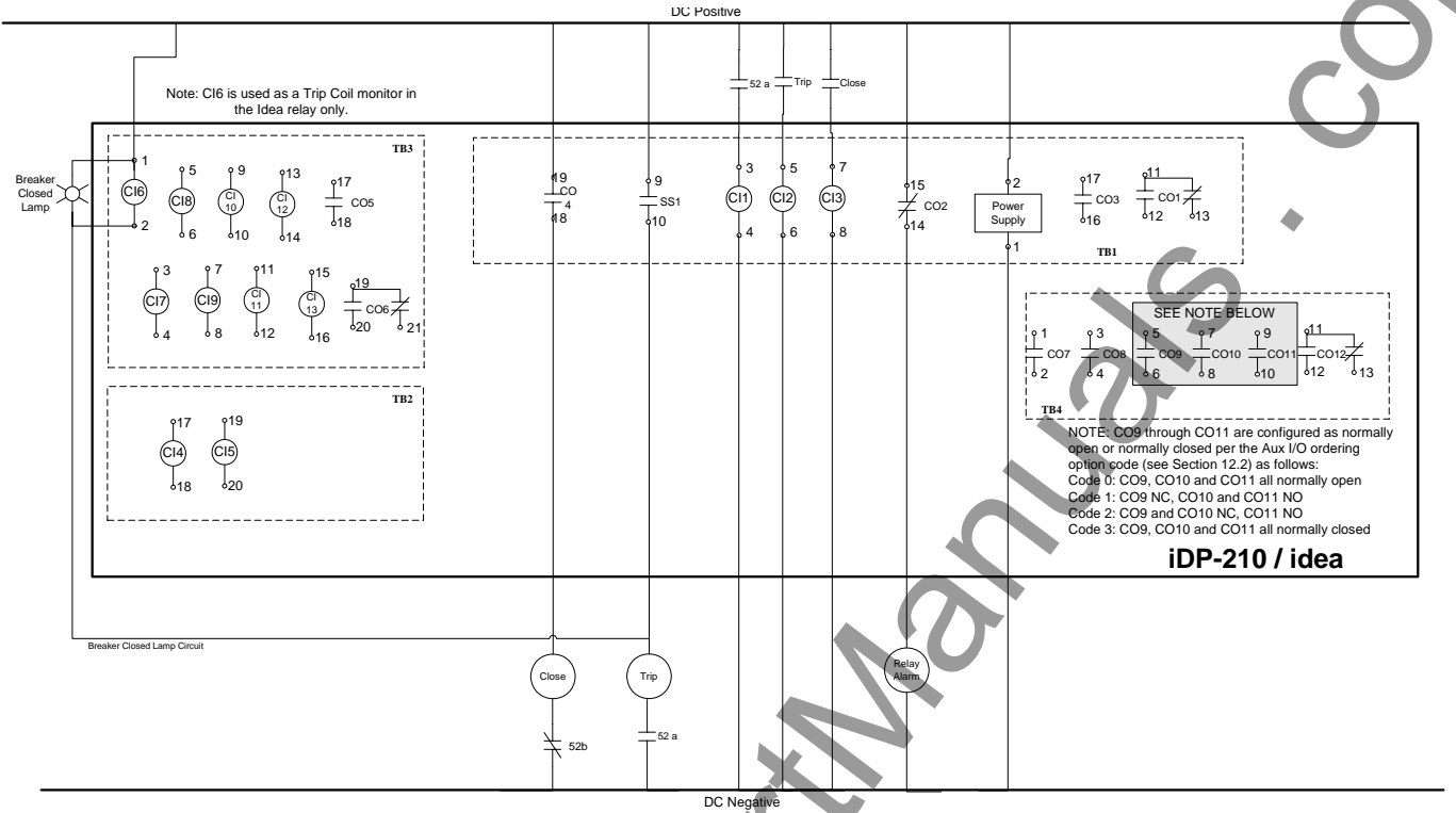
Figure 17: Edison Idea DC Connection Diagram Where Optional Contact I/O Board IS Present
