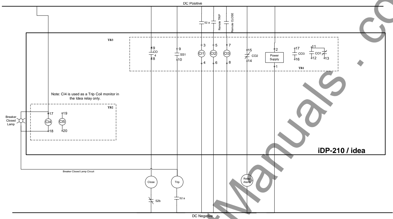
Figure 18: Edison Idea DC Connection Diagram Where Optional Contact I/O Board is NOT Present
