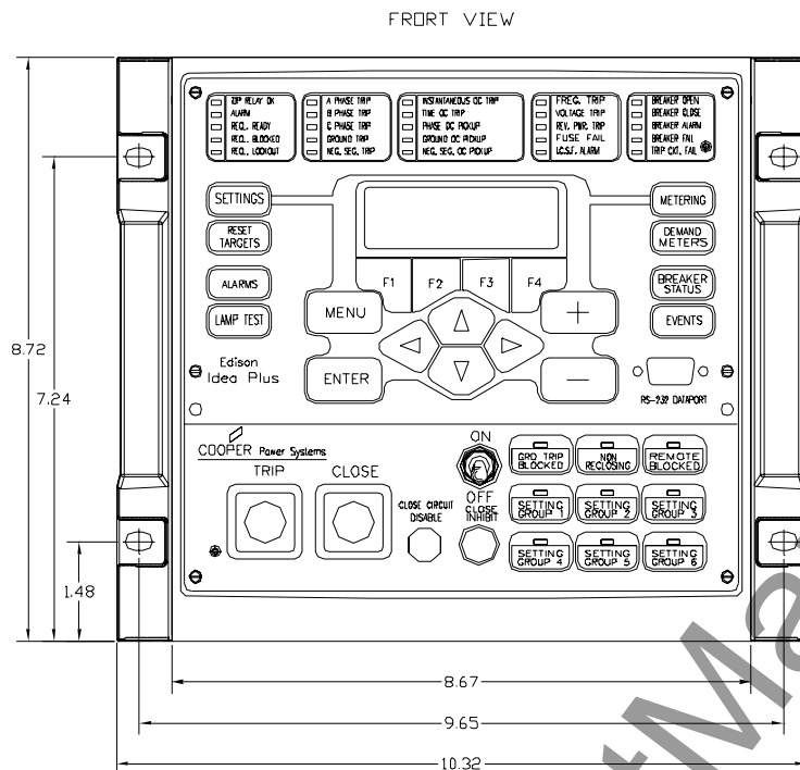
Figure 9: Idea PLUS Relay, Front View (inches)
