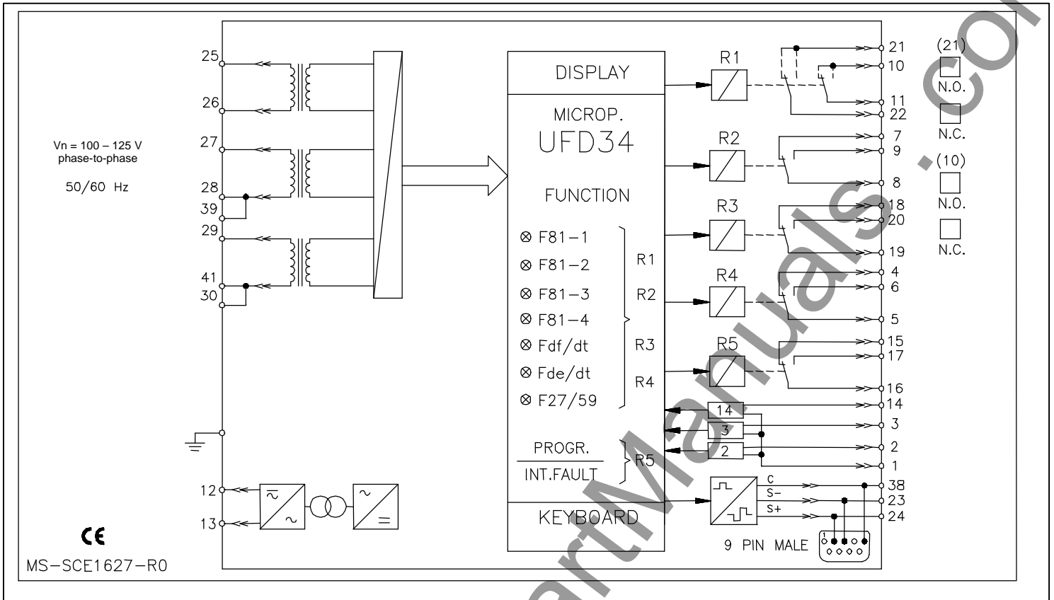
FIGURE 3: Wiring Diagram for the UFD34 Three Phase Relay
