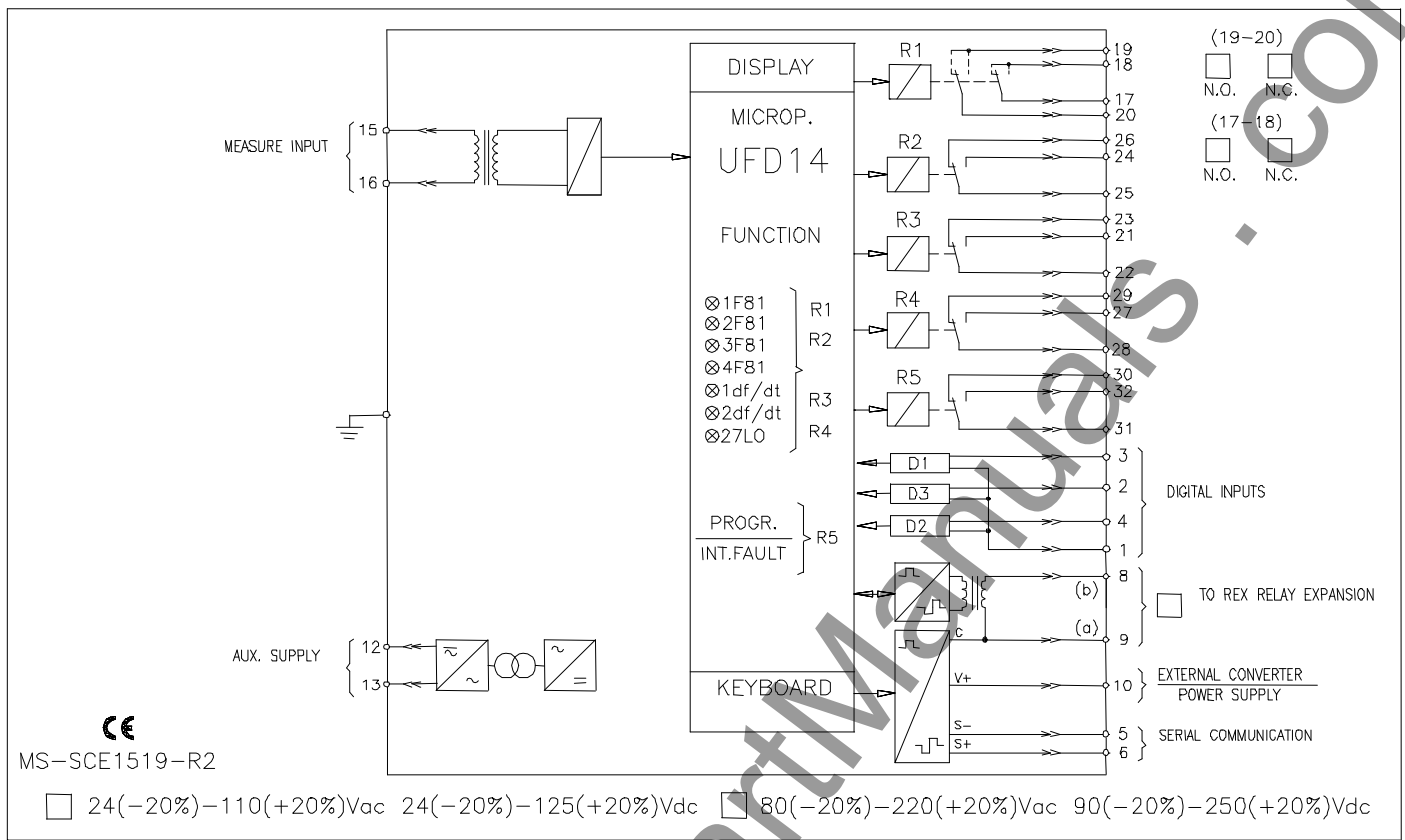
FIGURE 2: Wiring Diagram of the UFD14 Single Phase Relay
