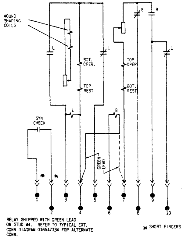
Fig. 7 (0165A7608-1) Internal Connection Diagram for Relay Type IJS52E
