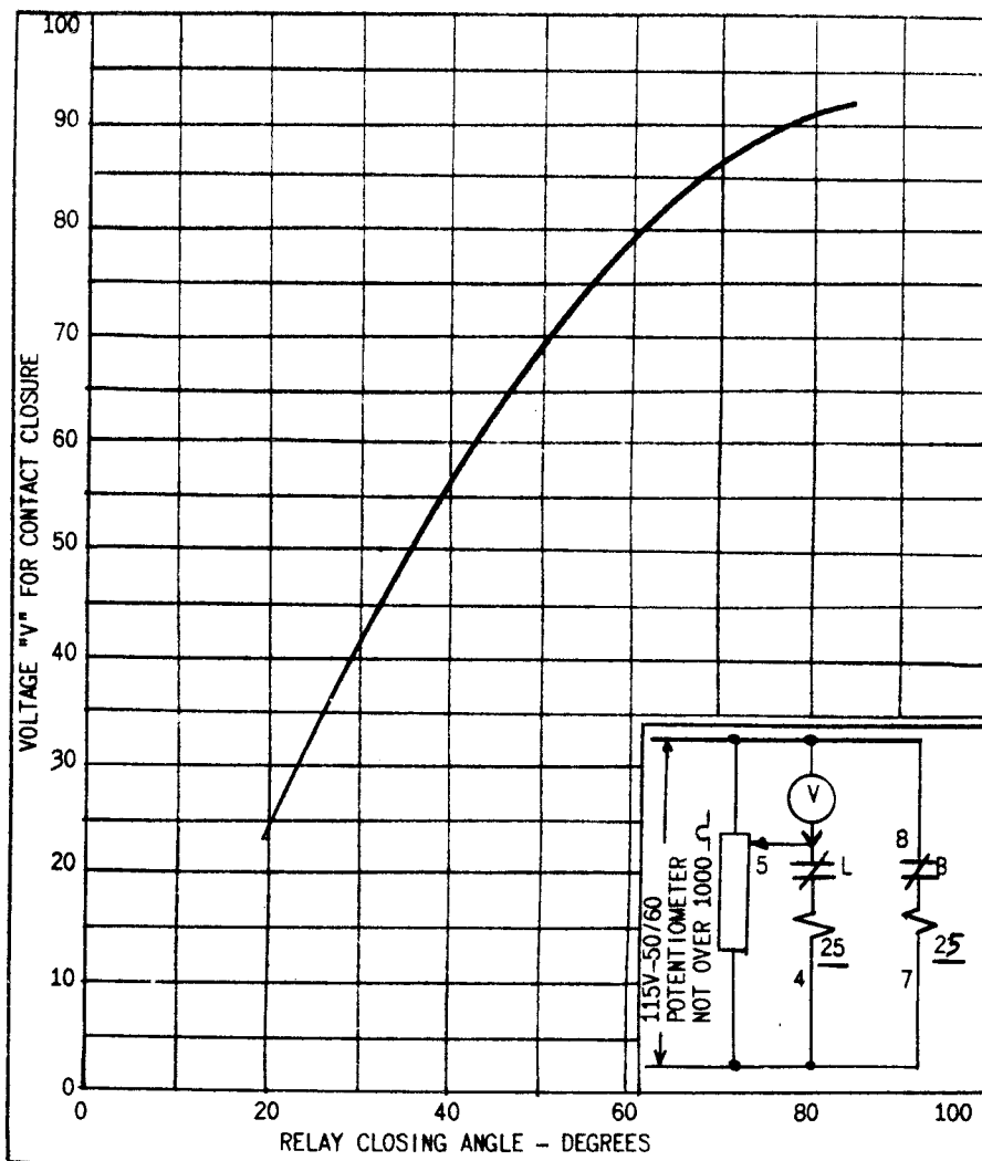
Fig. 11 (0165A7739-0) Connections and Curve to Make Closing Angle Adjustment Without Phase Shifter on 115 Volt 50/60 Cycle Relay. Relay Type IJS52E
