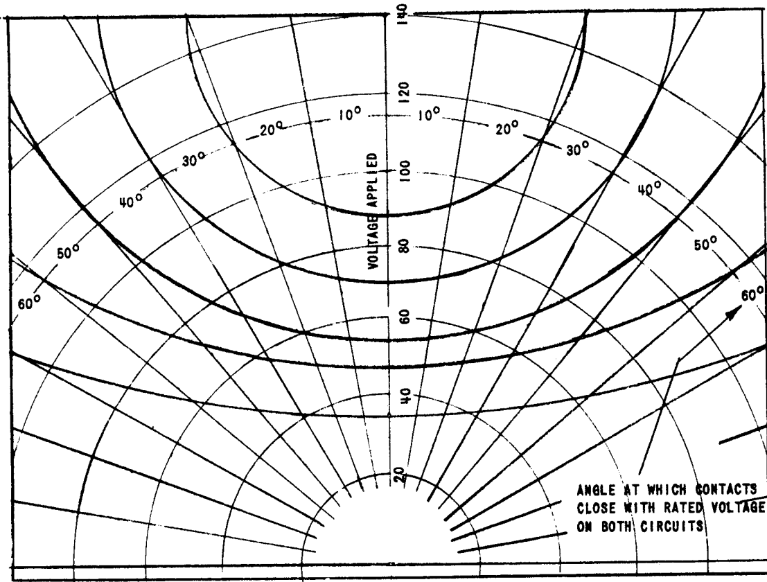
Fig. 1 (0165A7535-0) Typical Phase-Angle Characteristic of 115 Volt 50/60 Cycle Relay for Various Closing Adjustments with Rated Voltage Maintained on One Circuit. Standard Closing Angle Adjustment 20°
